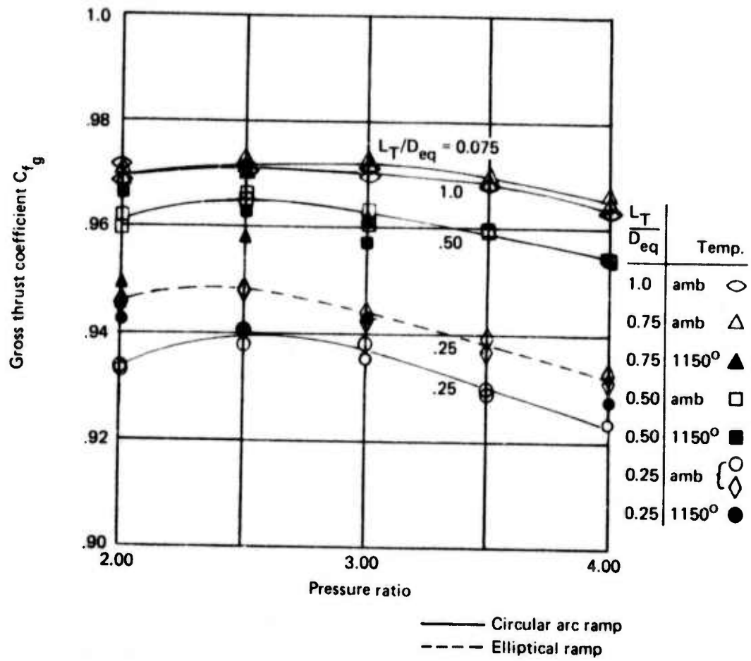
Figure 66.—Gross Thrust Coefficient for the 37-Tube, Area Ratio 2.75, Close-Packed Array
