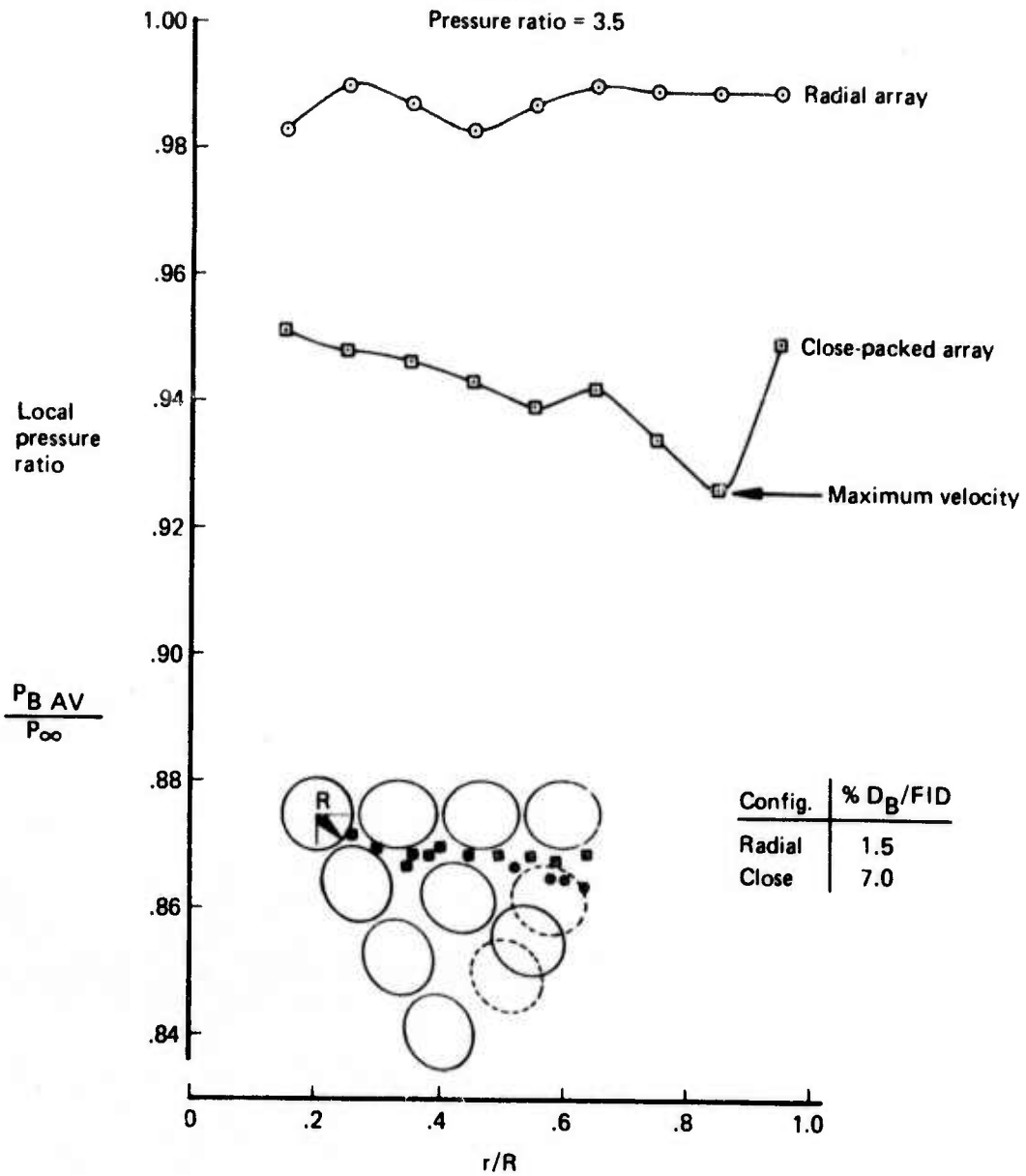
Figure 93.—Effect of Tube Array on Base Pressures and Drag
