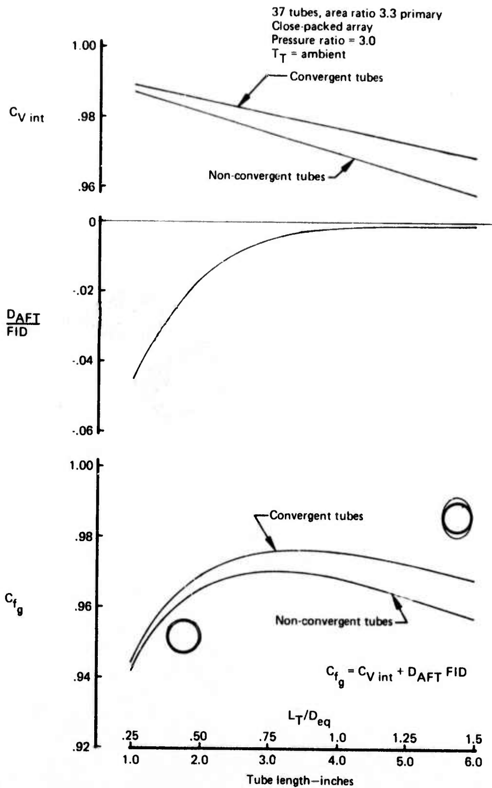
Figure 89.—Effect of Elliptical Convergent Versus Nonconvergent Tubes on Nozzle Performance
