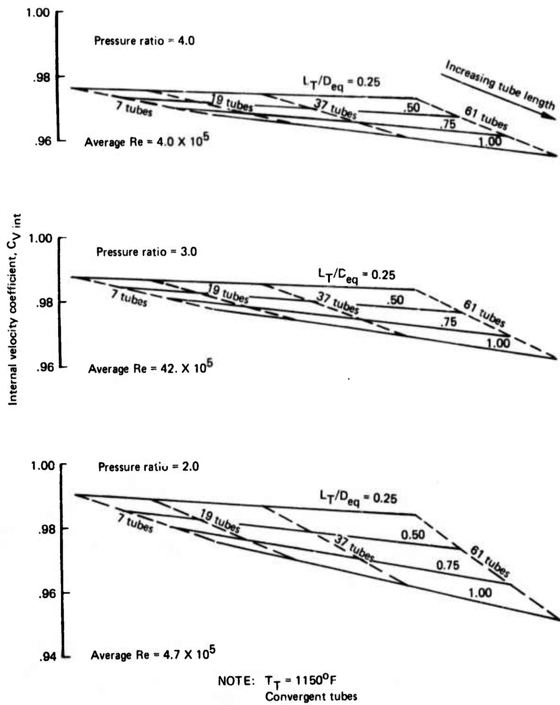
Figure 86.—Effect of Tube Length and Number on Internal Velocity Coefficient at 1150°F
