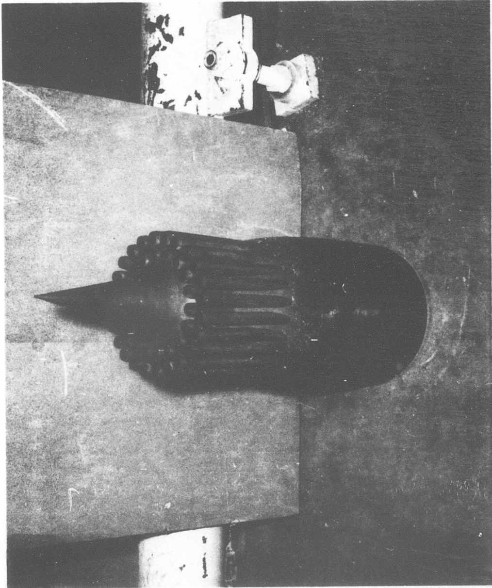
Figure 43.—42-Tube Annular Plug Nozzle
