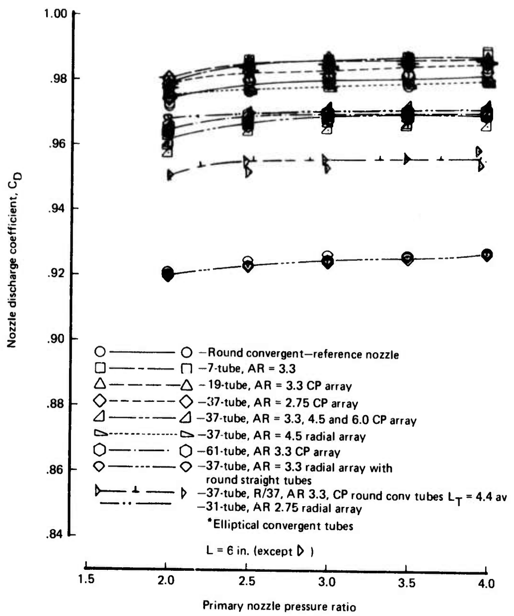
Figure 50.—Discharge Coefficients Ambient and 1150°F
