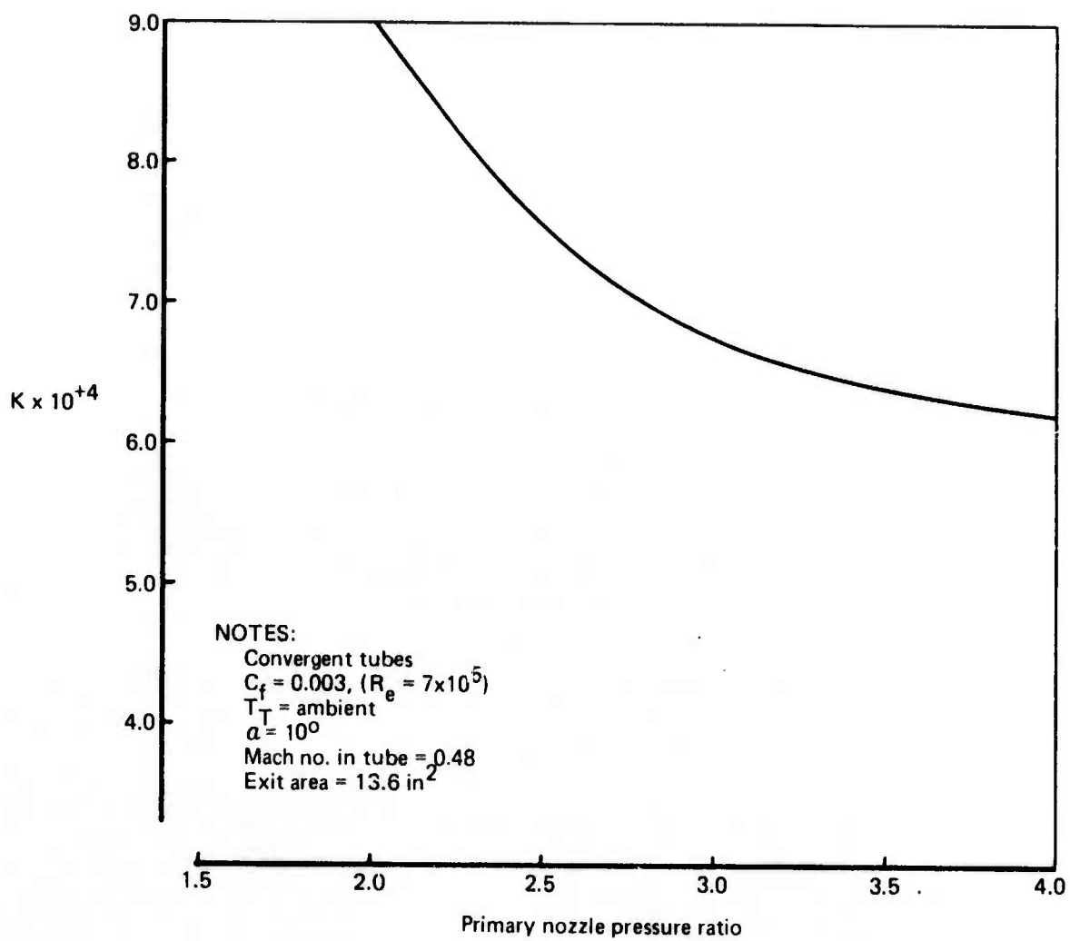
Figure 49.—Parameters in Performance Equation C_{V int} = C_V R/C - K L \sqrt{N}
