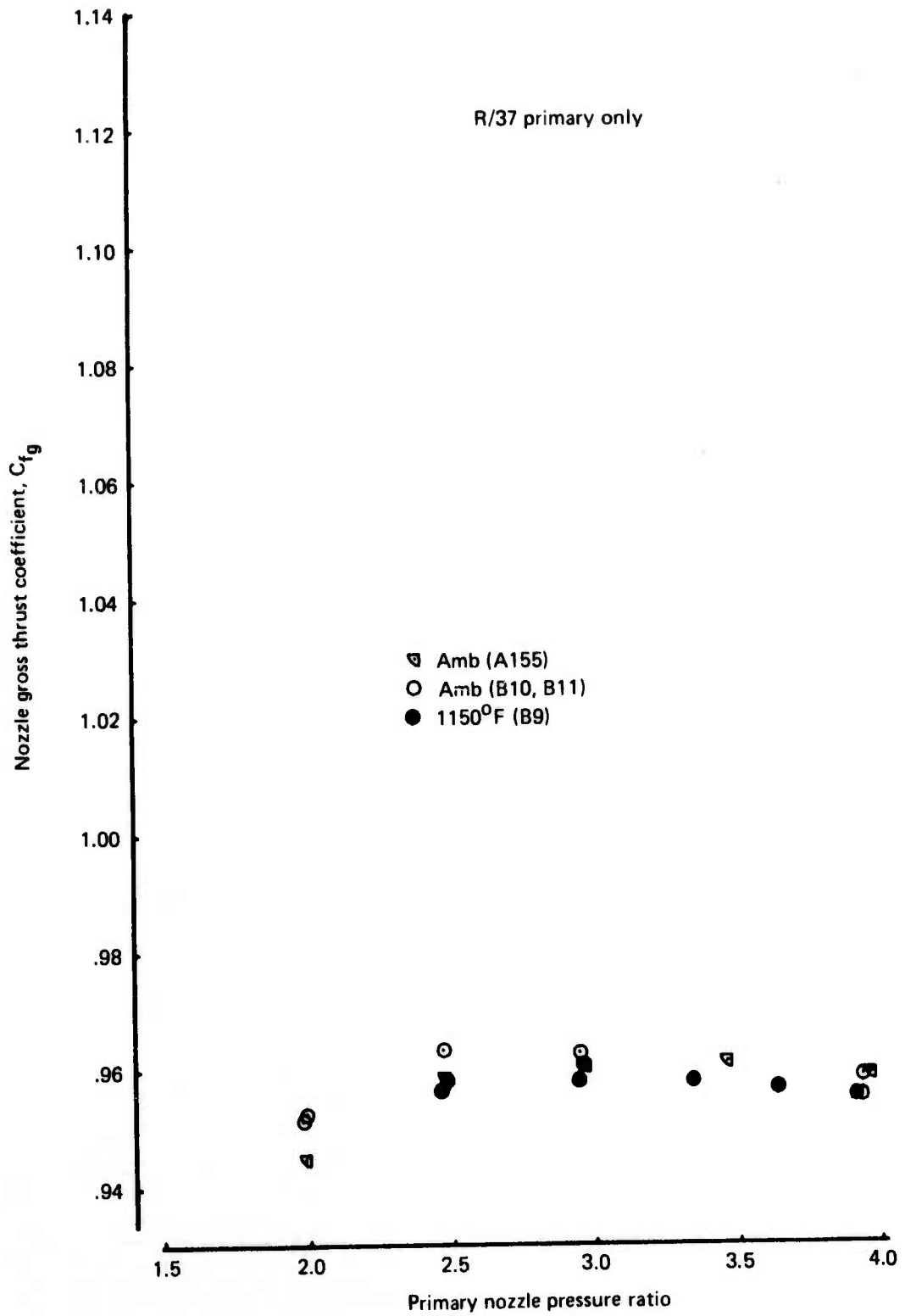
Figure 52.—Gross Thrust Coefficient Versus Pressure Ratio for R/37 Nozzle
