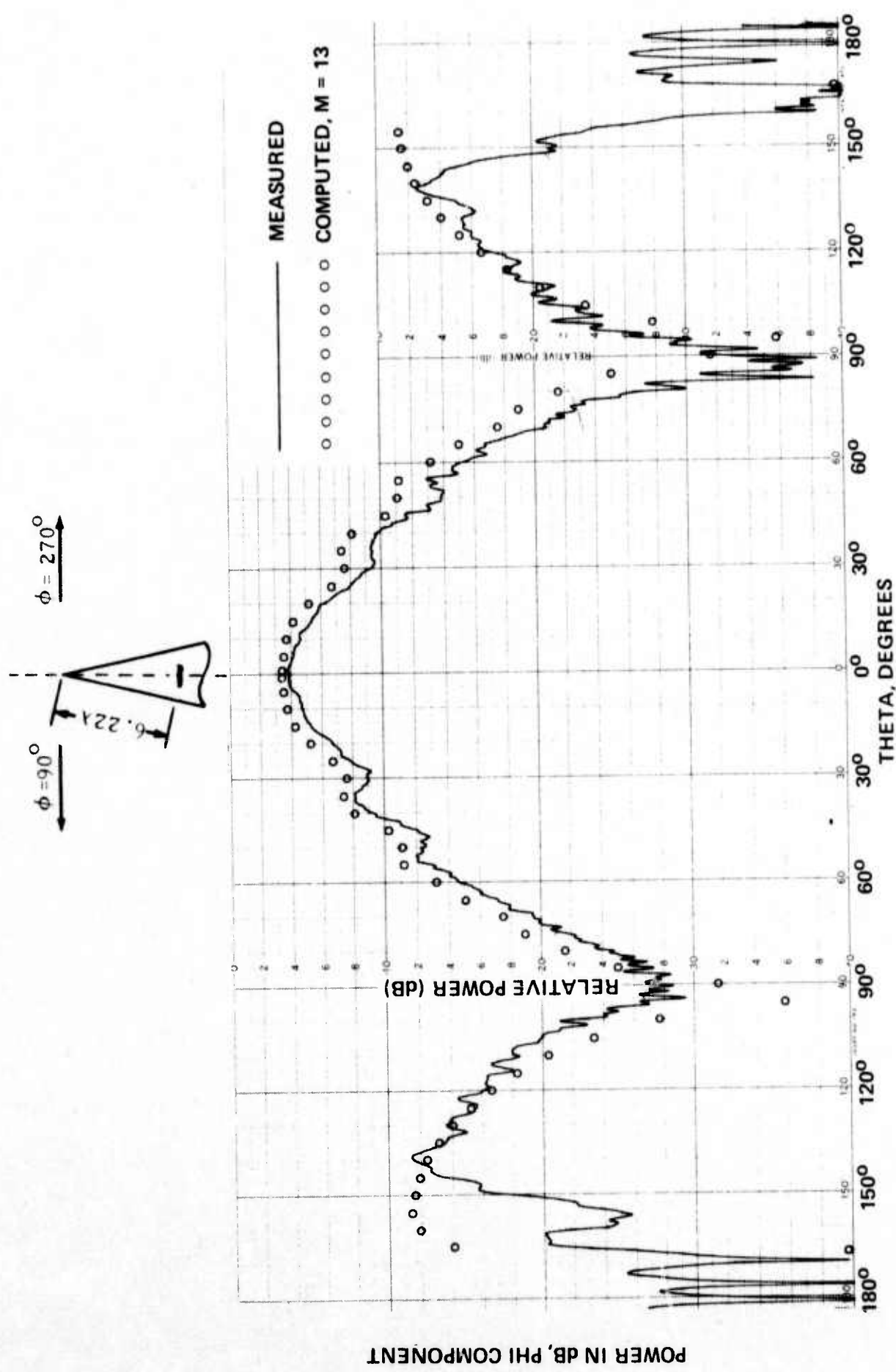
Figure 9. Measured and Computed ( M = 13 ) \phi -Polarized Patterns of \lambda/2 Circumferential Slot for \phi = 90^\circ , \phi = 270^\circ .
