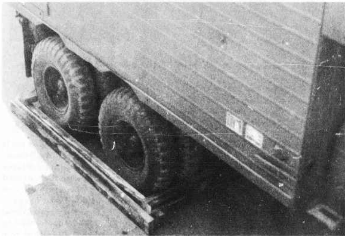
Figure 36. Views of Vehicle Wheel Blocking in SEABEE Barge.
