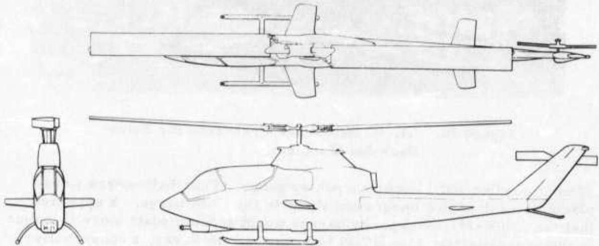
Figure 18. AH-1G Cobra Helicopter.
