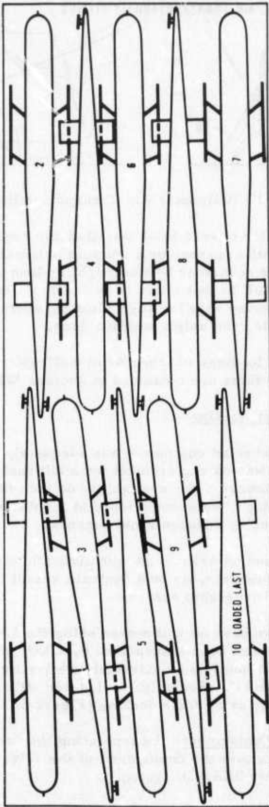
Figure 49. Stowage of 10 AH-1G Helicopters in SEABEE Barge.
