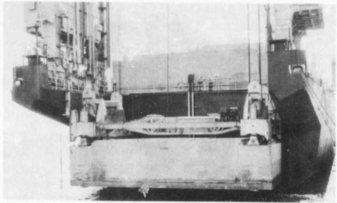
Figure 14. LASH Lighter Being Lifted Aboard.
