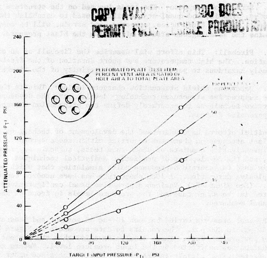
Figure 8. Input Pressure Versus Attenuated Pressure for Different Vent Areas
