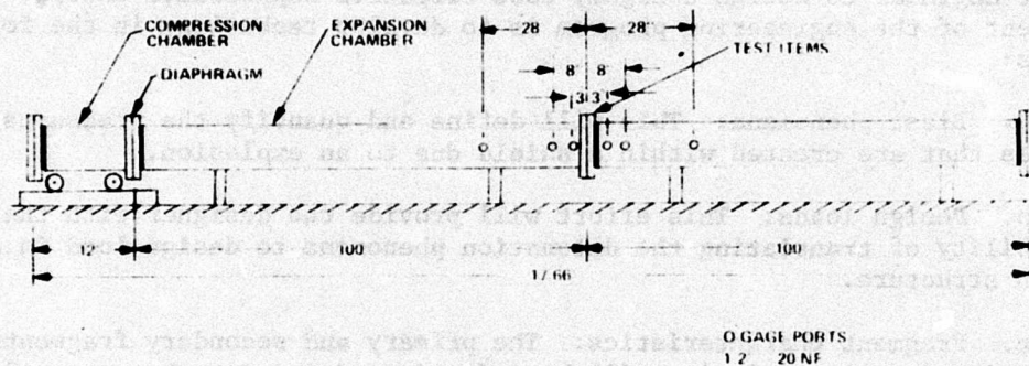
Figure 7. Shock Tube Test Setup
