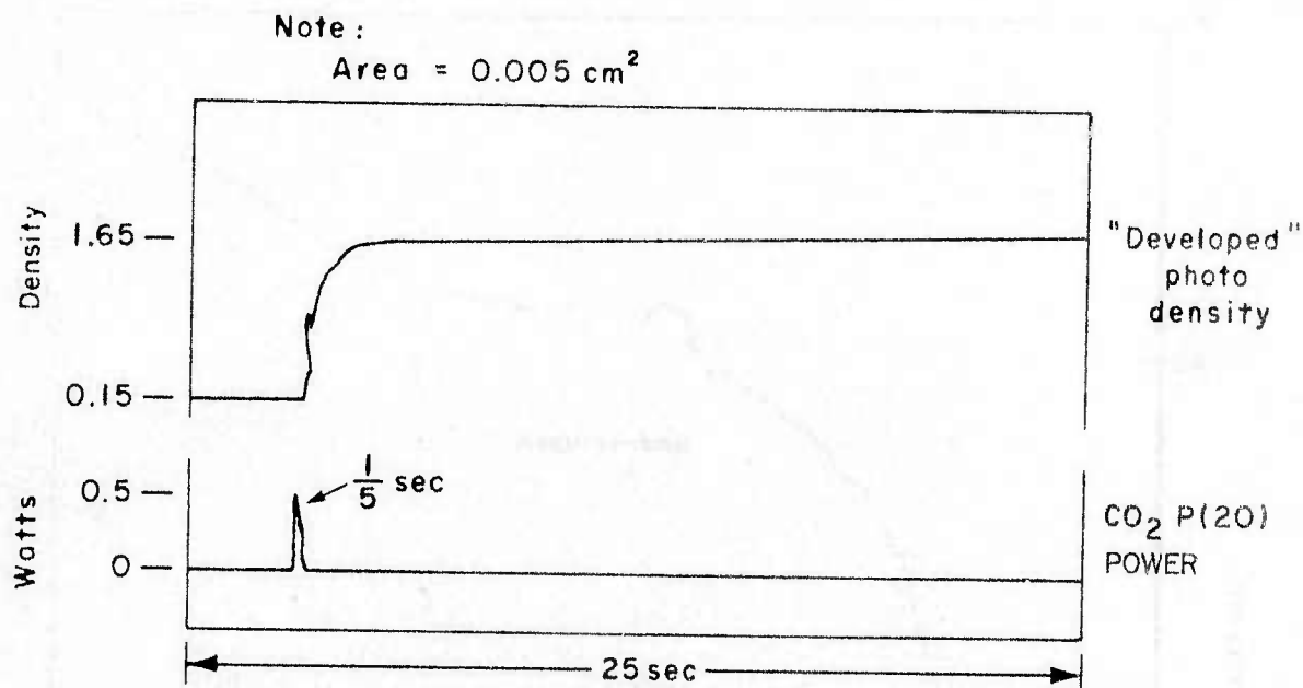
Figure 7. Representative Oscilloscope Trace of Film Development Time Using CO 2 Laser Irradiation and 0.005 cm 2 Film Development Area
