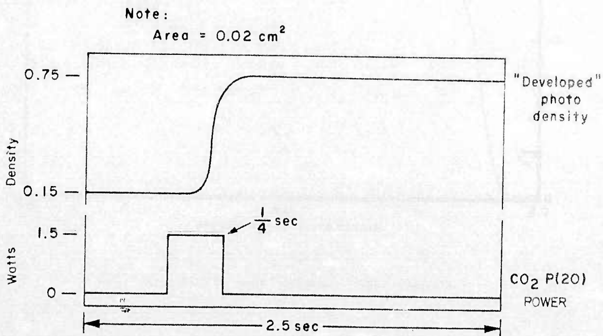
Figure 8. Representative Oscilloscope Trace of Film Development Time Using CO 2 Laser Irradiation and 0.02 cm 2 Film Development Area.
