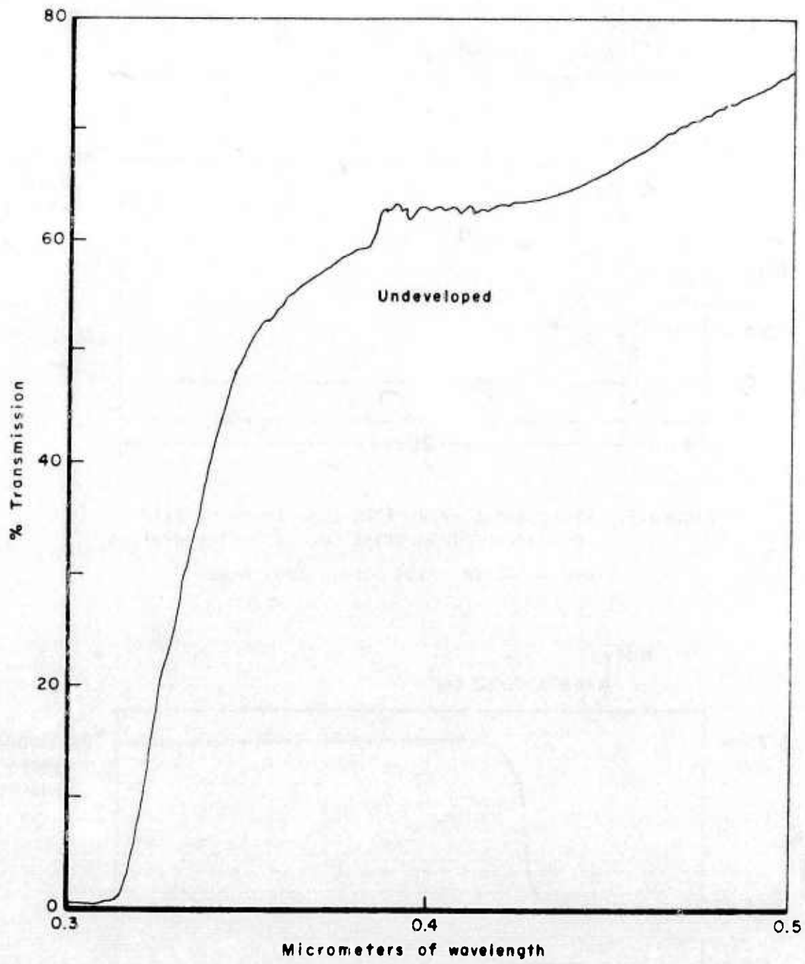
Figure 9. "UV" Transmission Curve of 7959 Film
