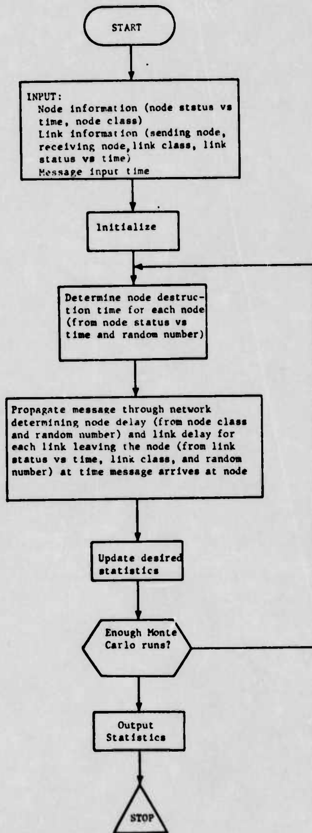
FIGURE 2.2 DYNAMIC NETWORK SIMULATOR
