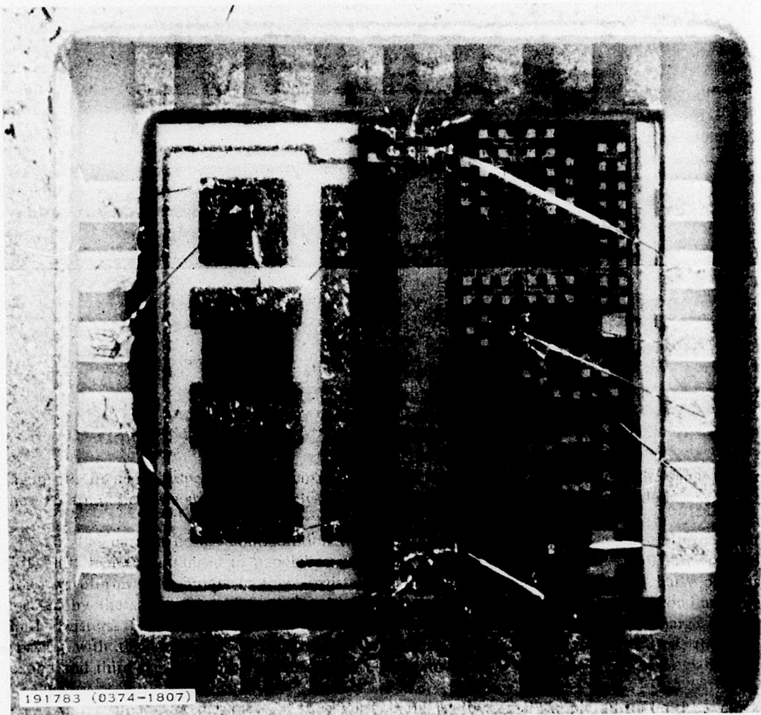
Figure 14. Photomicrograph of DLM Type CCD
