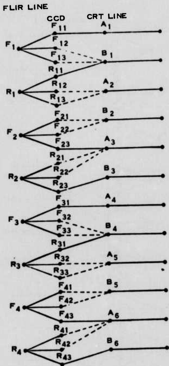
C. 1.5 CRT LINES/IR LINE: FILLED DISPLAY FOR 160 DETECTORS
