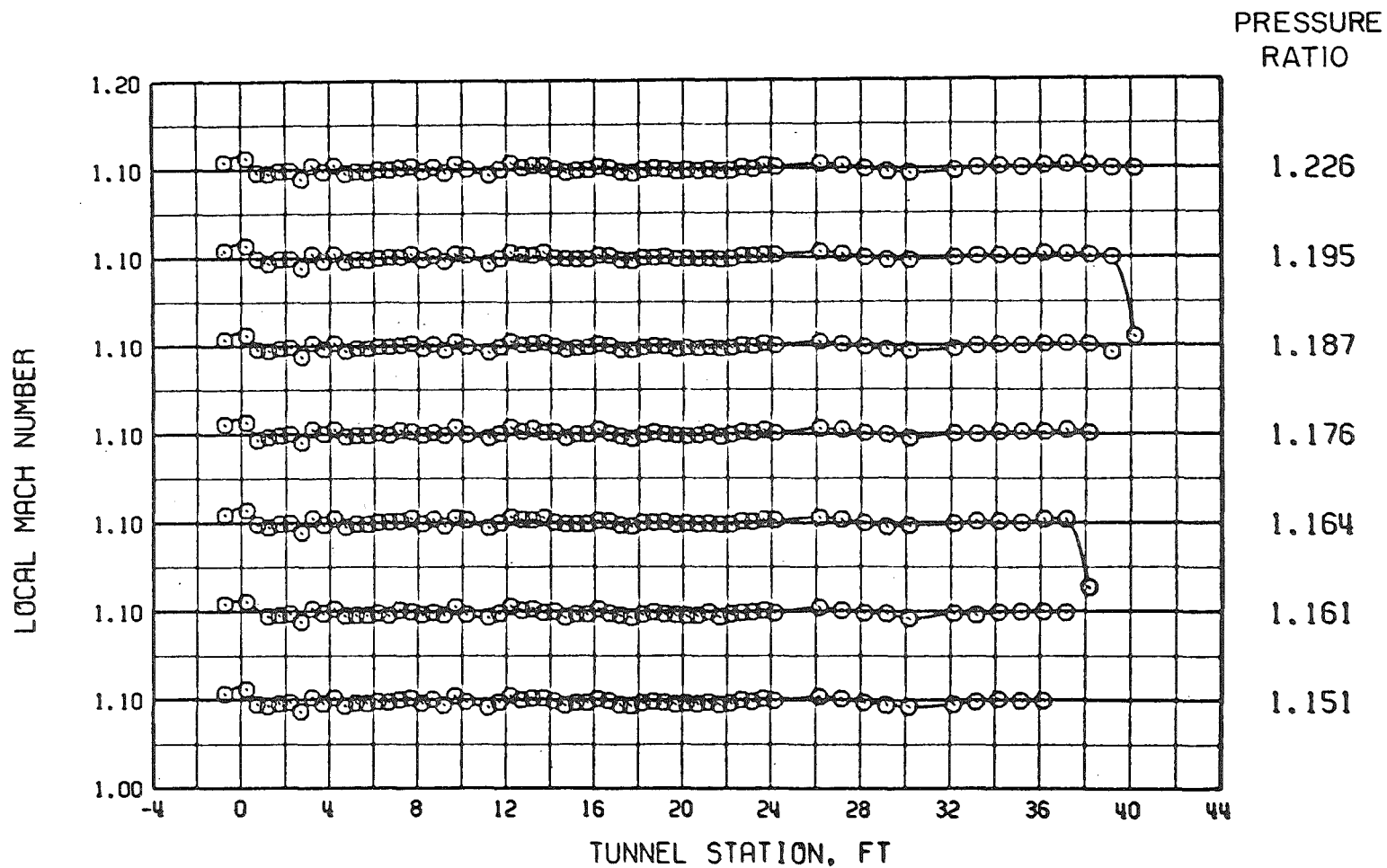
d. M = 1.1 , \theta_w = 0 , and \tau = 6 Figure 10. Continued.
