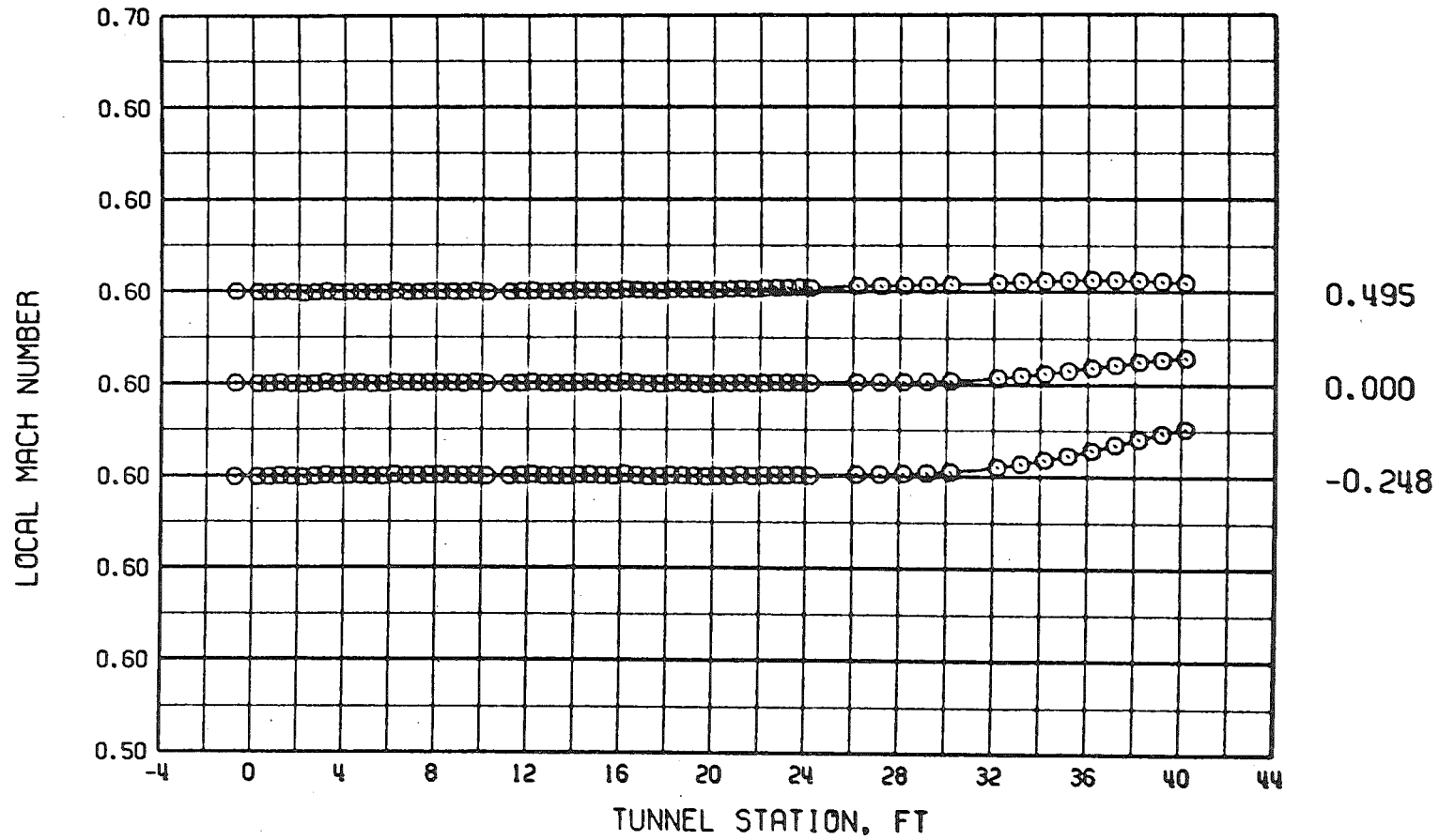
b. M = 0.6 , \lambda \cong 1.10 , and \tau = 6 Figure 15. Continued.
