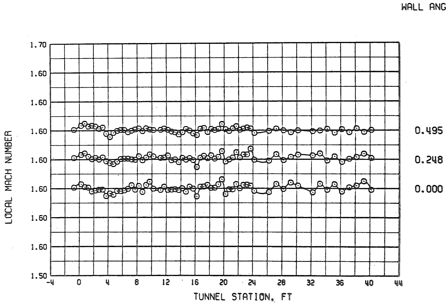
k. M = 1.6 , \lambda = 1.50 , and \tau = 2 Figure 17. Concluded.
