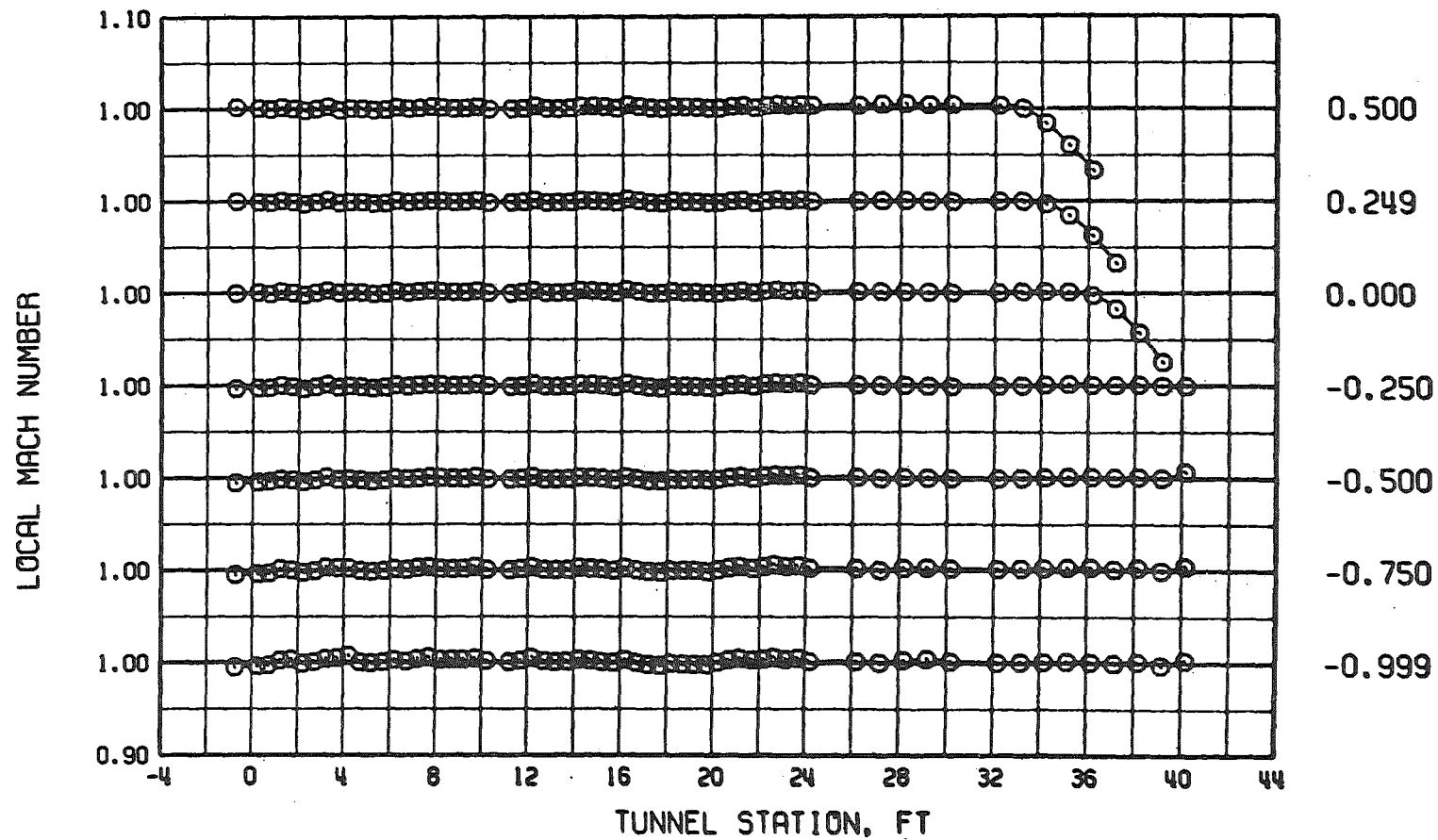
f. M = 1.0 , \lambda = 1.17 , and \tau = 6 Figure 15. Continued.
