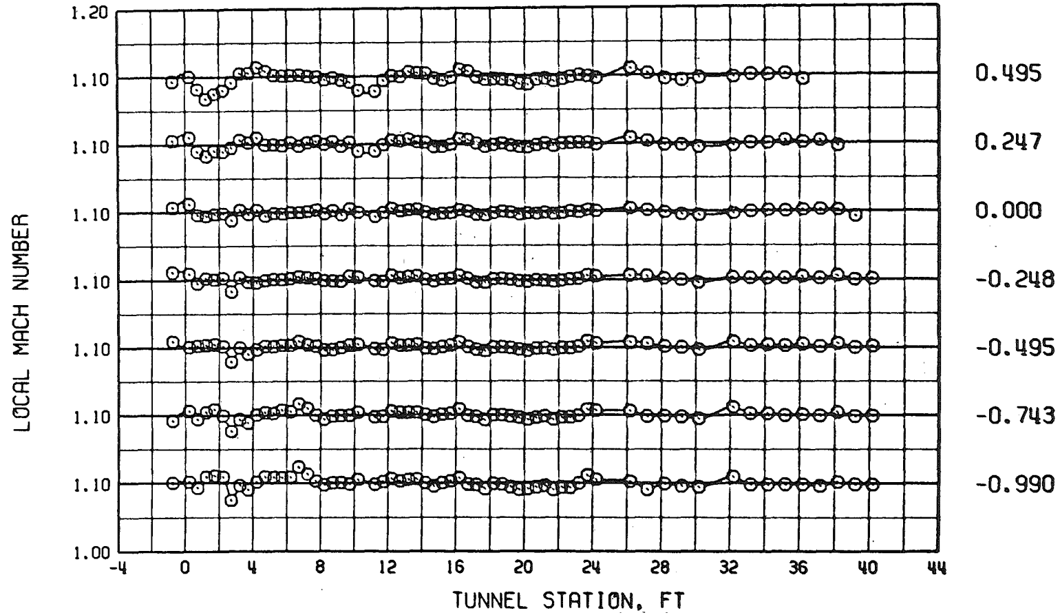
g. M = 1.1 , \lambda = 1.19 , and \tau = 6 Figure 15. Continued.
