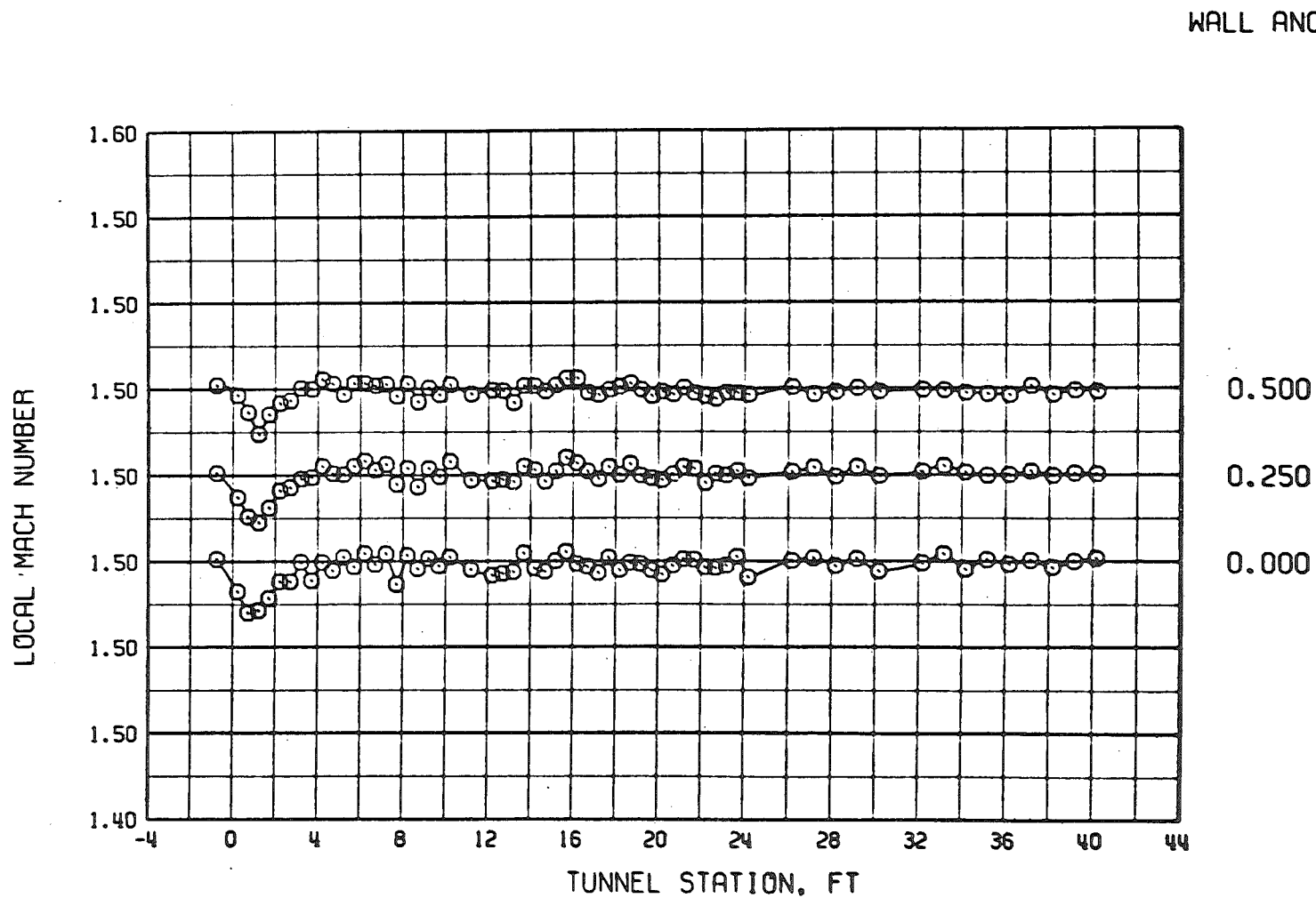
k. M = 1.5 , \lambda = 1.40 , and \tau = 4 Figure 16. Continued.
