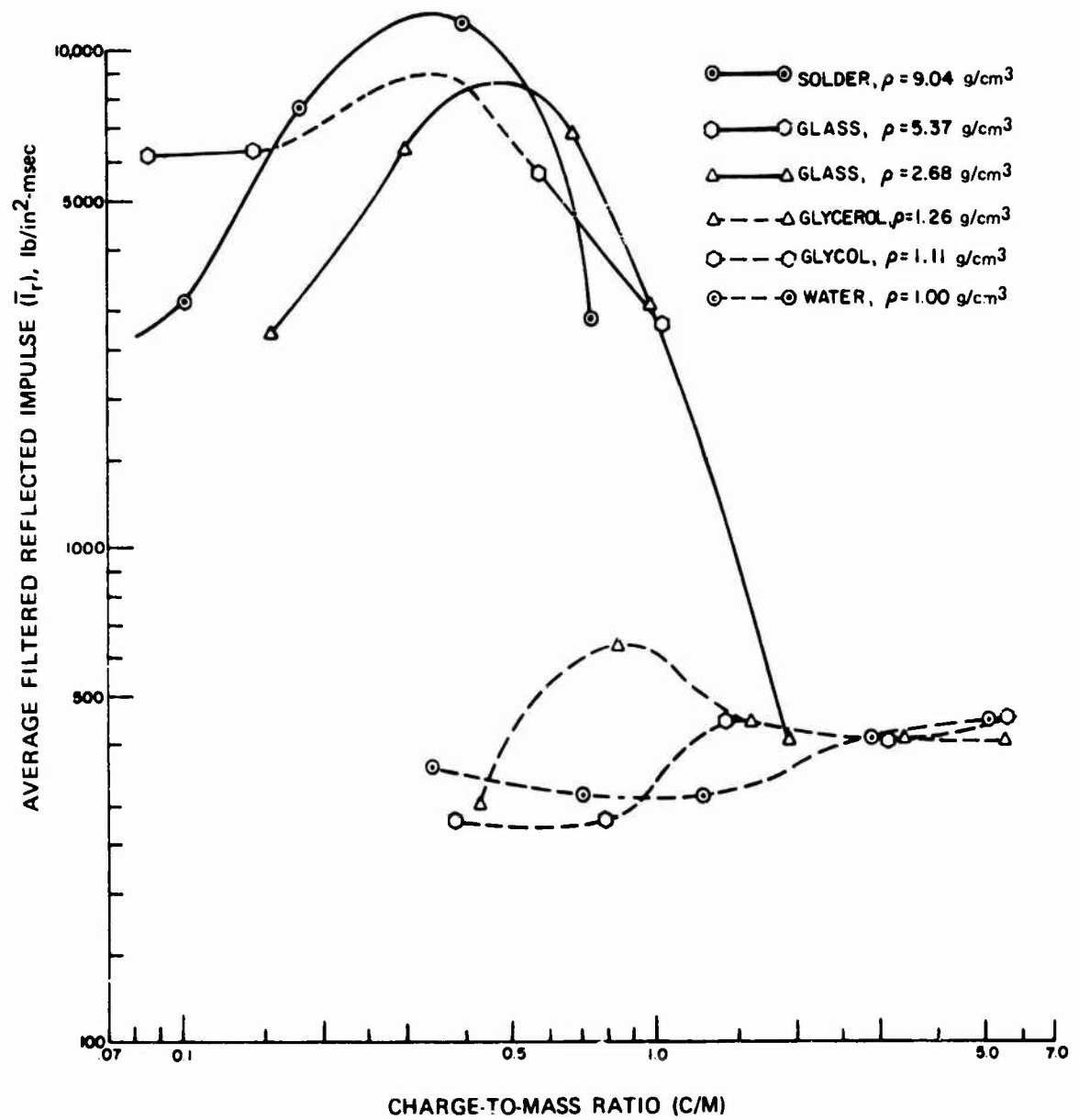
FIGURE 34. Average Filtered Reflected Impulse Versus Charge-to-Mass Ratio (Atmospheric Pressure ( P_r ) of 11.867 \text{lb/in}^2 ).
