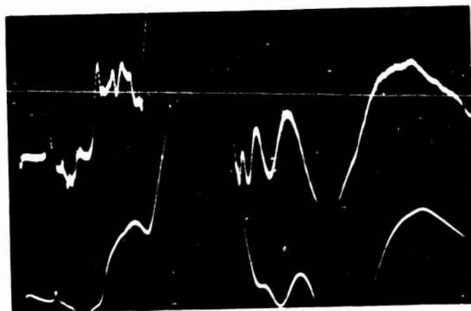
FIGURE B-20. Pressure-Time Data from a 120-Series Glycerol/Lucite Surround. Charge-to-Mass Ratio 5.06. Sweep Rate 100 \mu sec/div.
