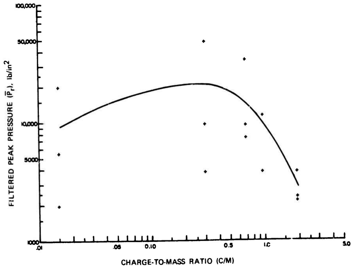
FIGURE 32. Filtered Reflected Peak Pressure Versus Charge-to-Mass Ratio for Glass Surround.
