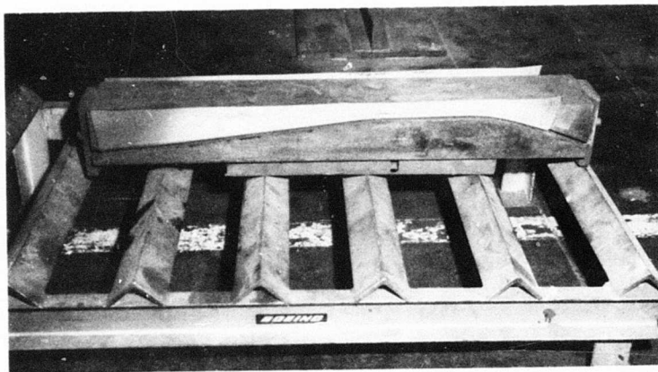
Figure 18: UPPER DUCT HALF LOADED INTO SECOND STAGE CONTOUR DIES.
