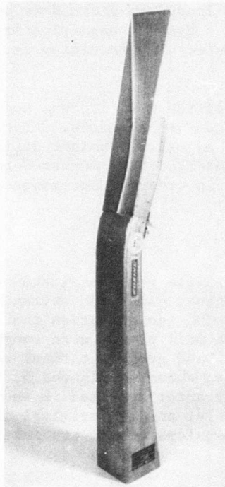
Figure 2: COMPLETED TITANIUM DUCT PORTION OF "PRODUCTION SIMULATION" INLET.
