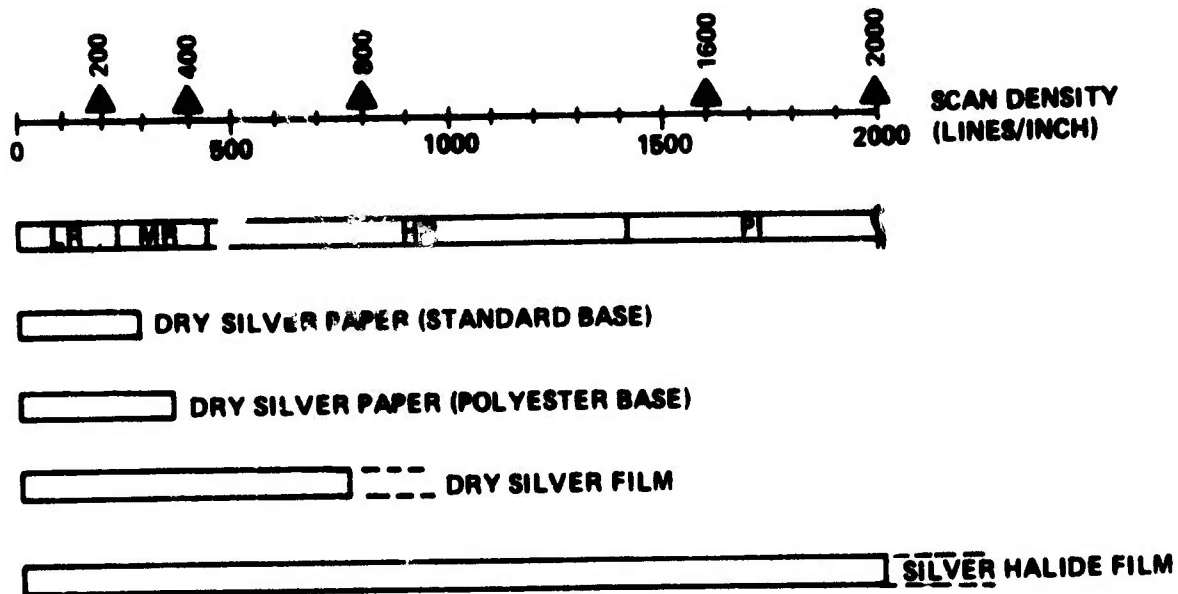
Figure 3.8. Application Range for Recording Data
