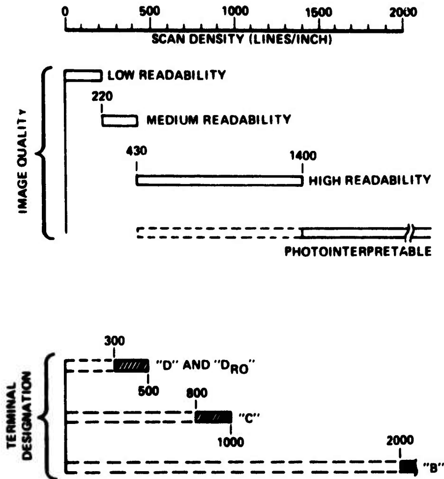
Figure 2.1. Image Quality and Terminal Operating Ranges for Scan Density
