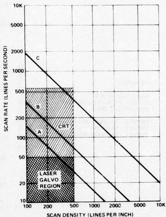
Figure 3.5. Laser-Galvanometer and CRT Performance Limitation
