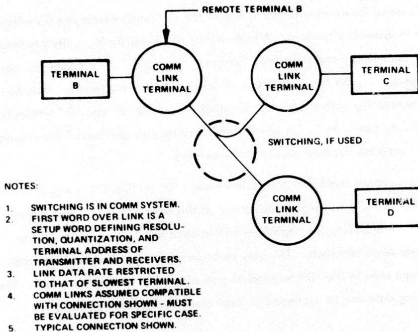
Figure 3.14 Terminal Multidrop Arrangement
