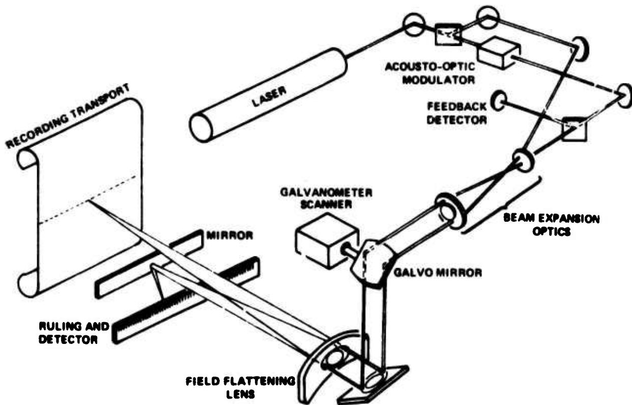
Figure 3.11. Improved Laser-Galvanometer Implementation
