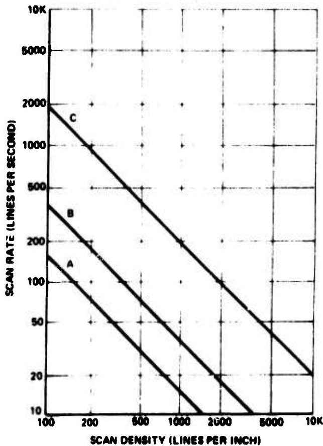
Figure 3.3. Recorder/Scanner Scan Rate Versus Scan Density
