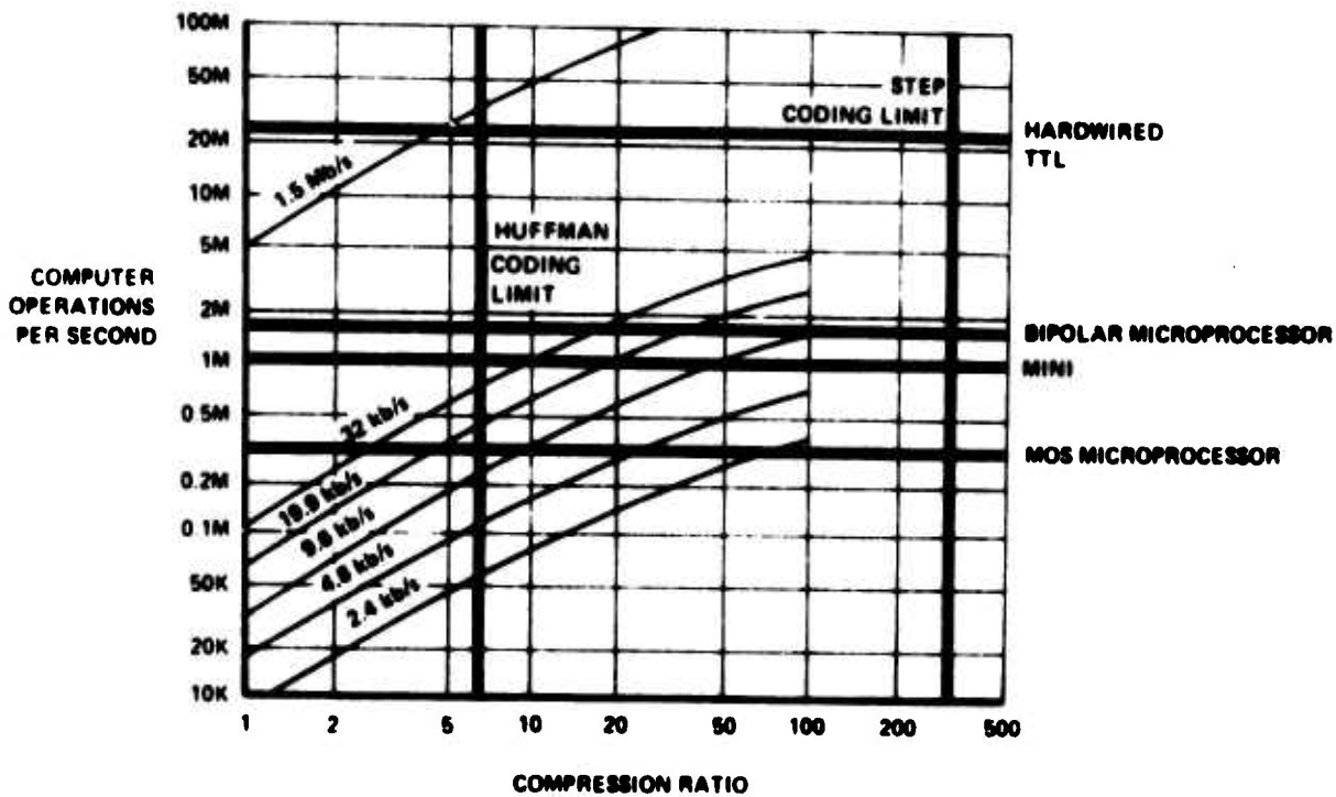
Figure 3.20. Data Compression Processing Limitations
