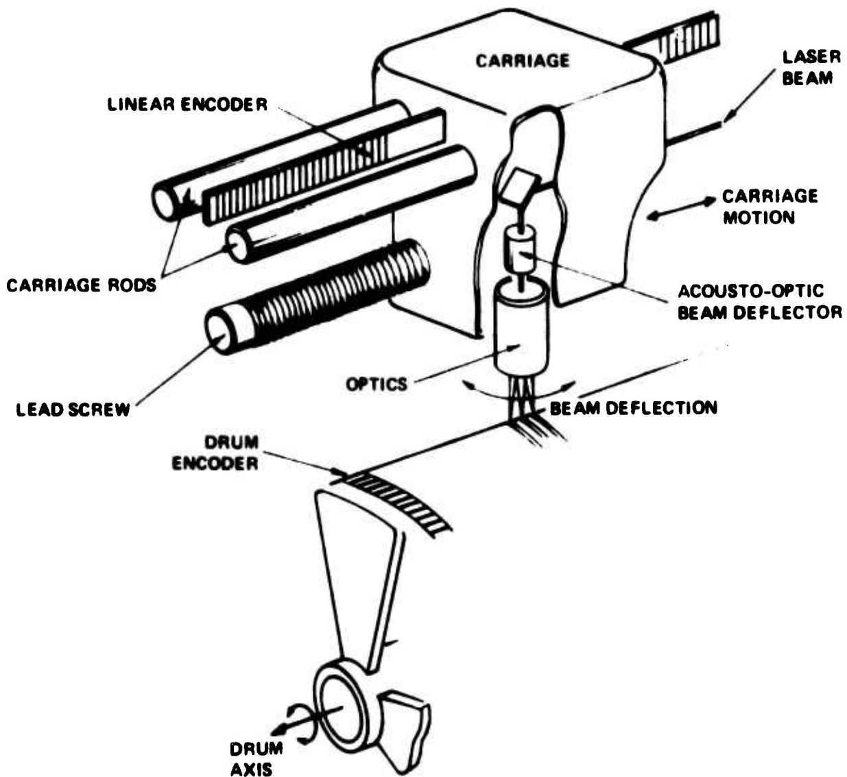
Figure 3.12. Acousto-Optically Controlled Down Recorder/Scanner
