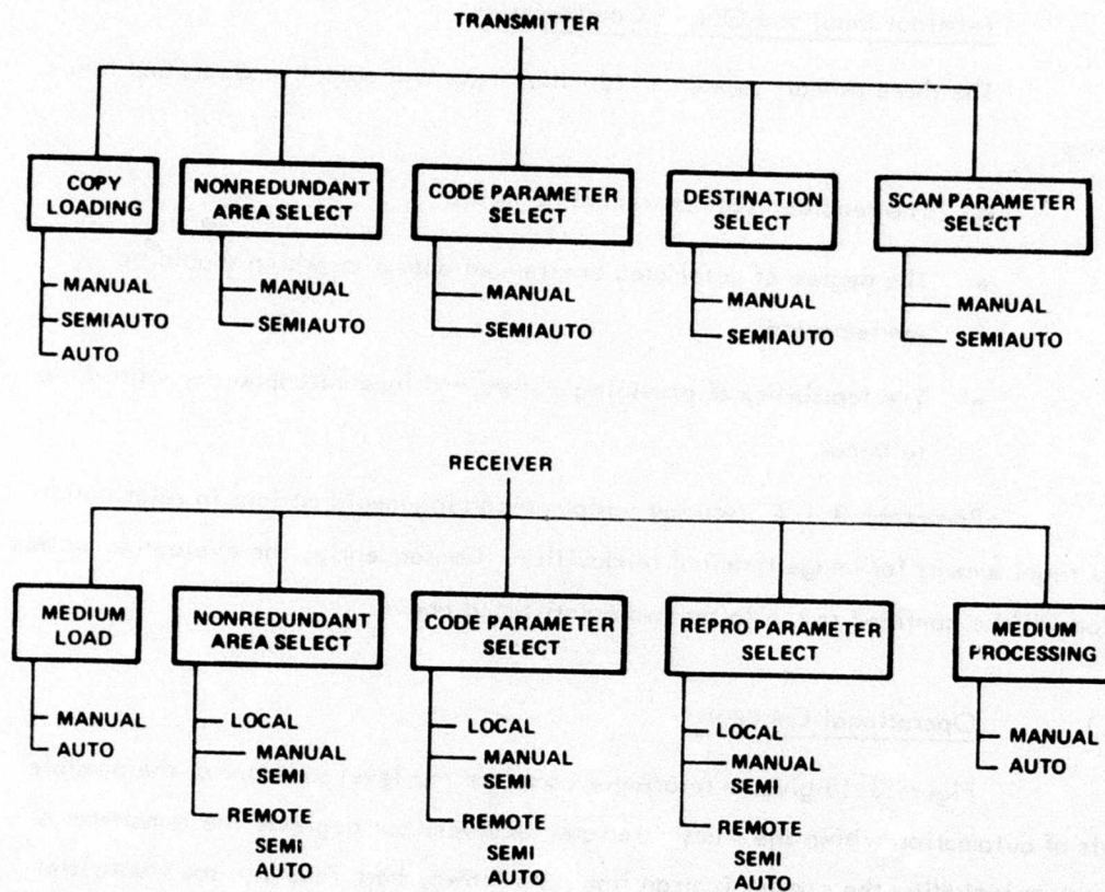
Figure 3.13. Terminal Automation Options
