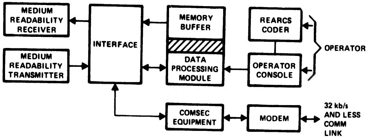
Figure 4.1. "D" Terminal Block Diagram
