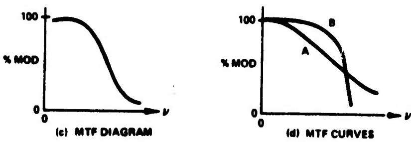
Figure 3.1. Image Spatial Frequency and MTF
