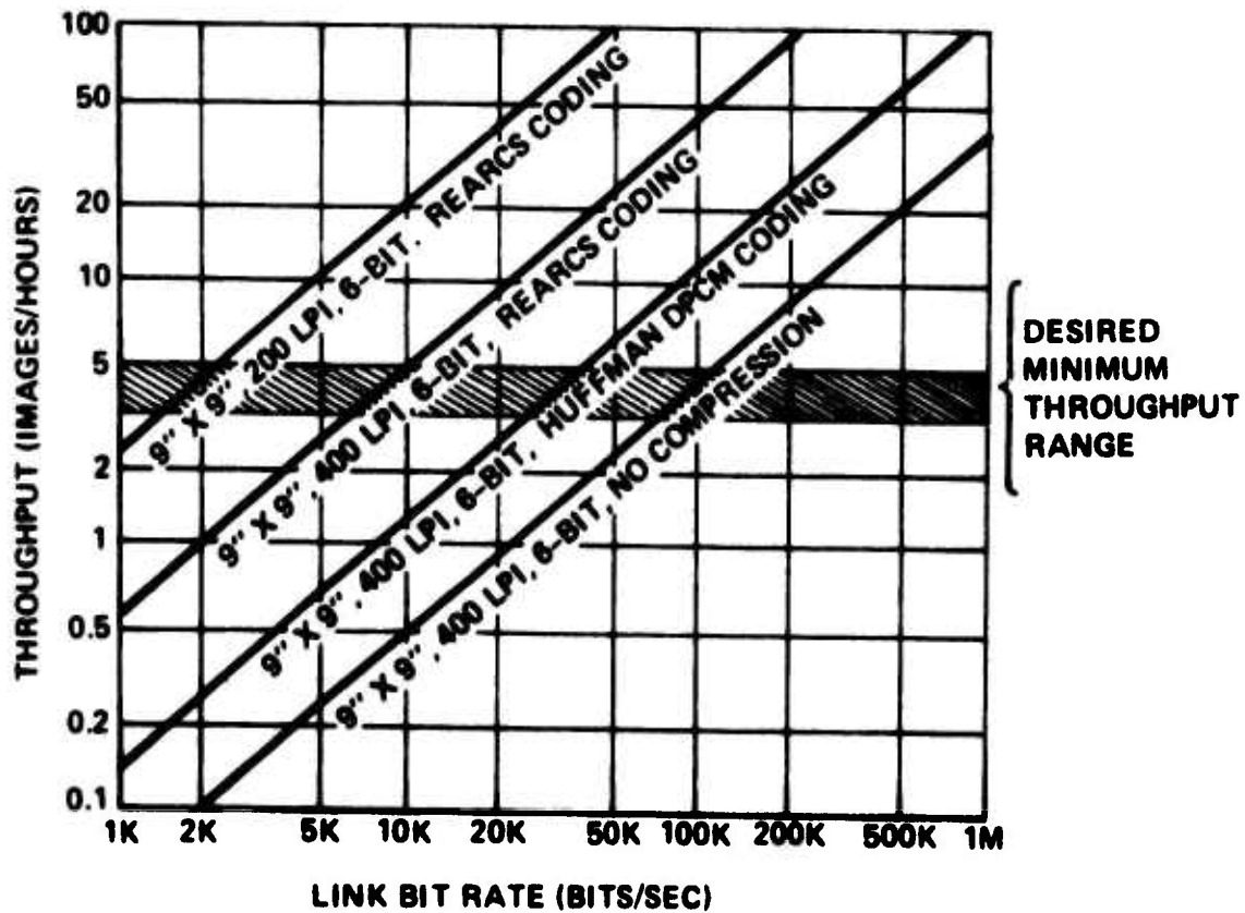
Figure 2.4. Image Throughput Versus Link Bit Rate For Link Limited Operation (No Overhead)
