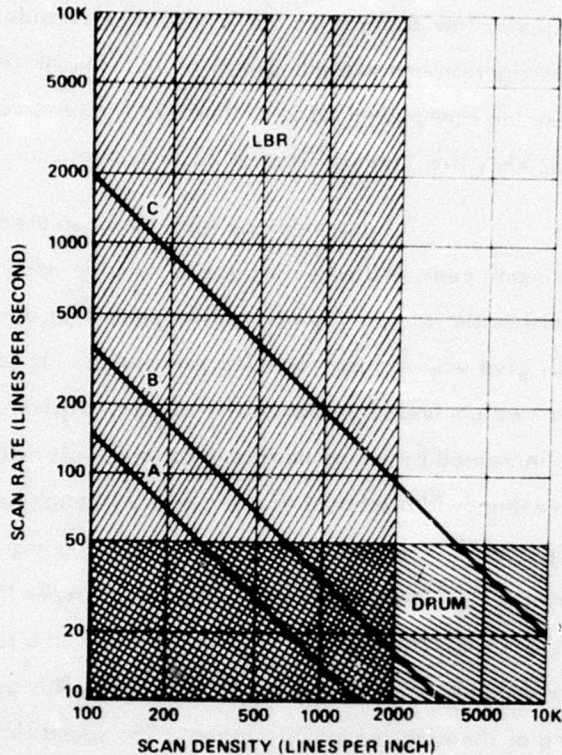
Figure 3.6. Drum and LBR Performance Limitations
