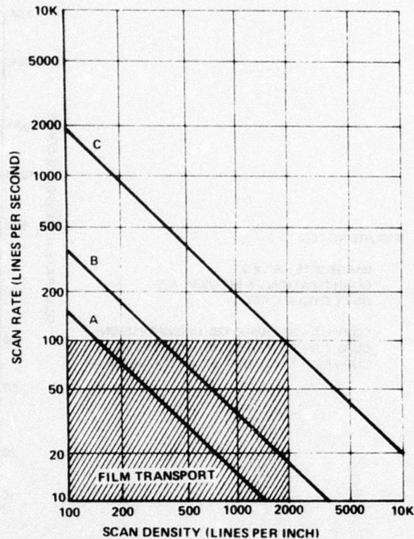
Figure 3.4. Film Transport Limitations
