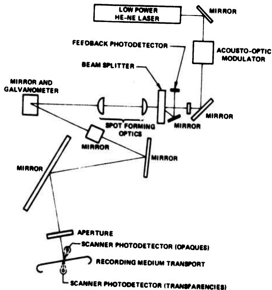
Figure 3.10. Laser-Galvanometer Recorder/Scanner Components
