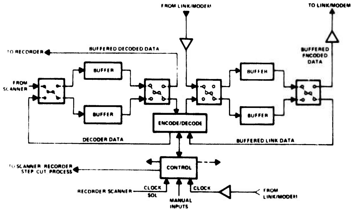
Figure 3.15. Basic Data Processing Function Diagram
