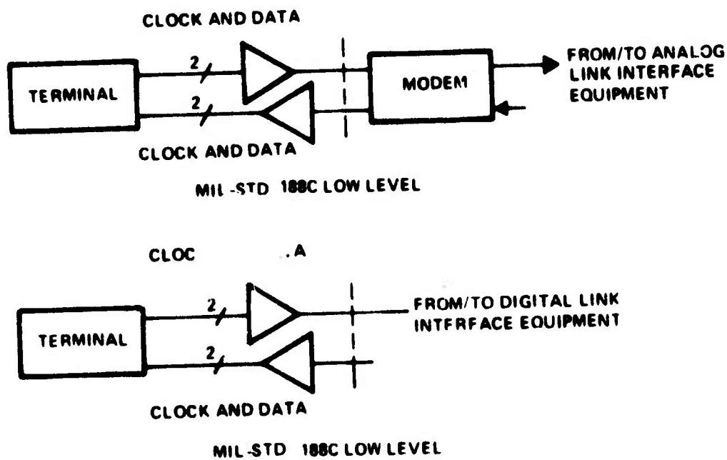
Figure 3.17. Terminal Interface Through MIL-STD-188C
