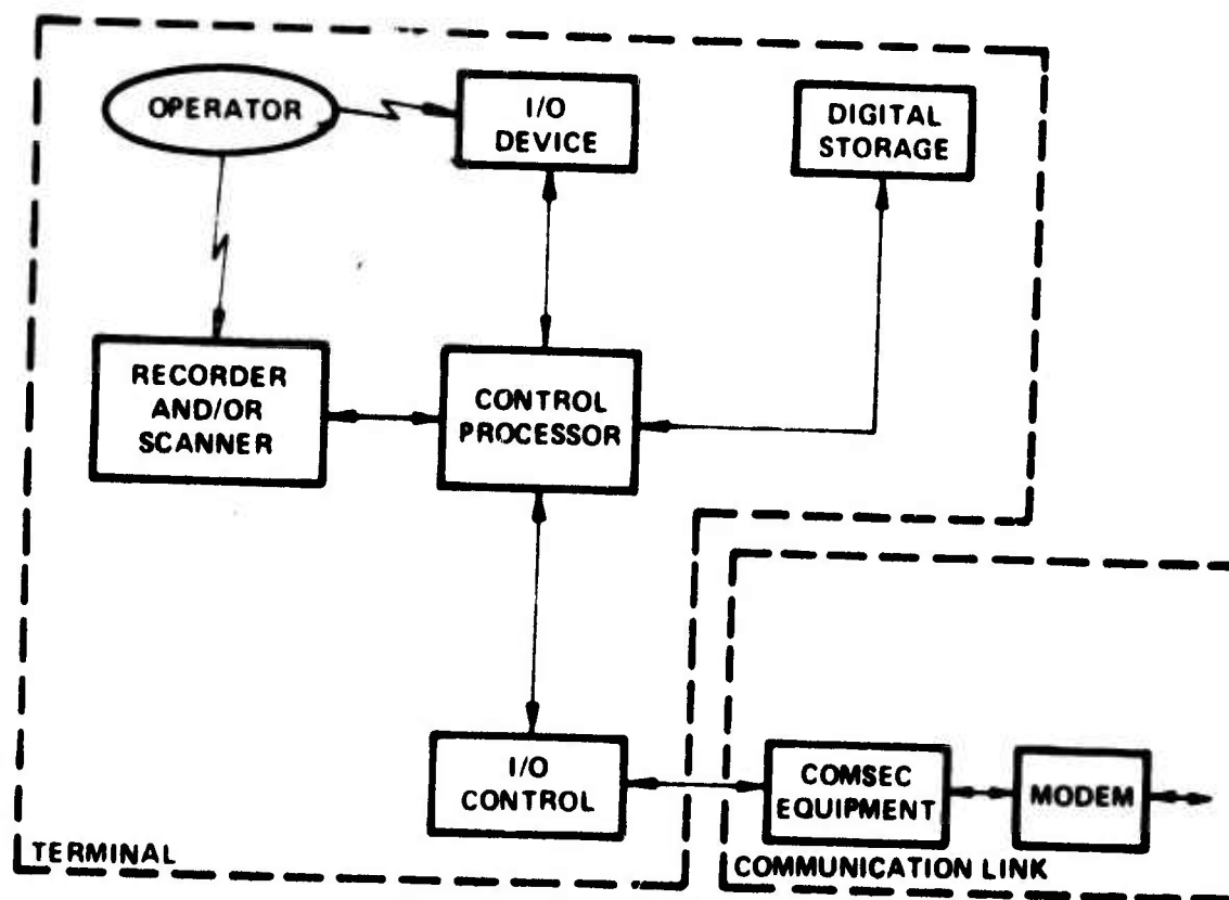
Figure 2.2. General Block Diagram of Terminal
