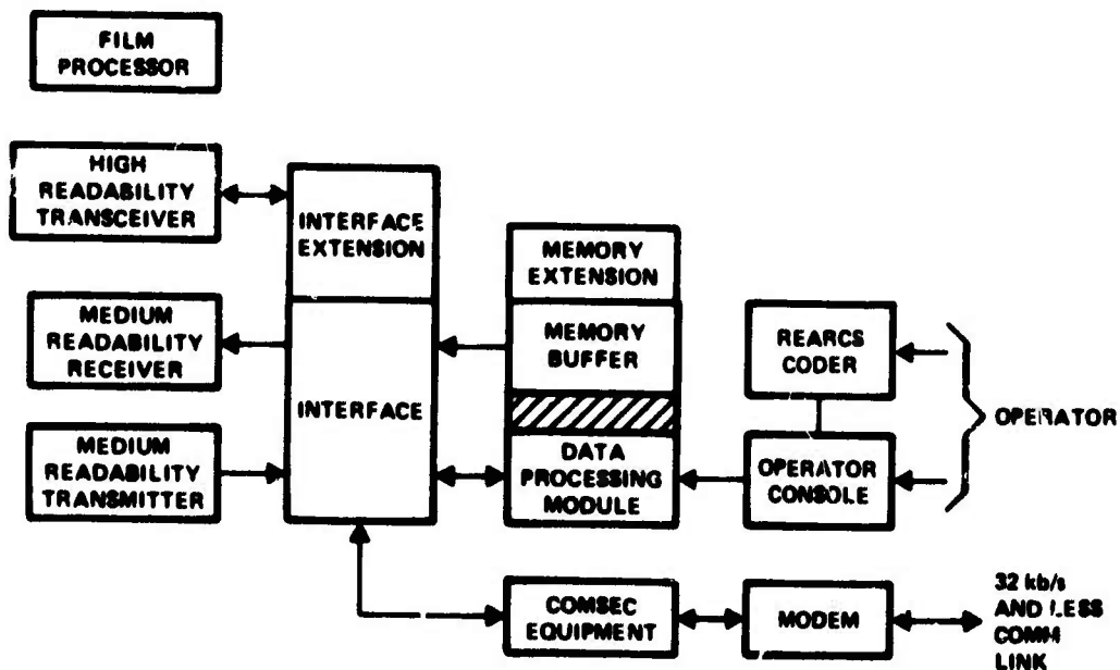
Figure 4.4. "C" Terminal Block Diagram
