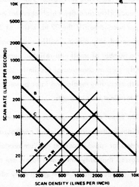
Figure 3.9. Recorder Laser Power Requirements
