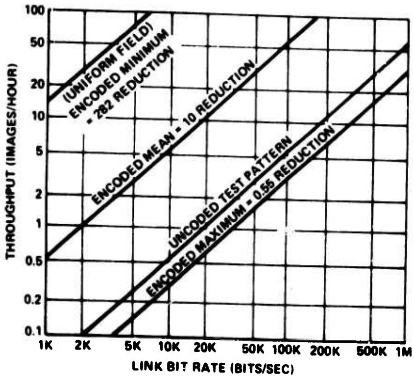
Figure 2.5. Throughput Versus Link Rate As A Function of Step-Coding Reduction
