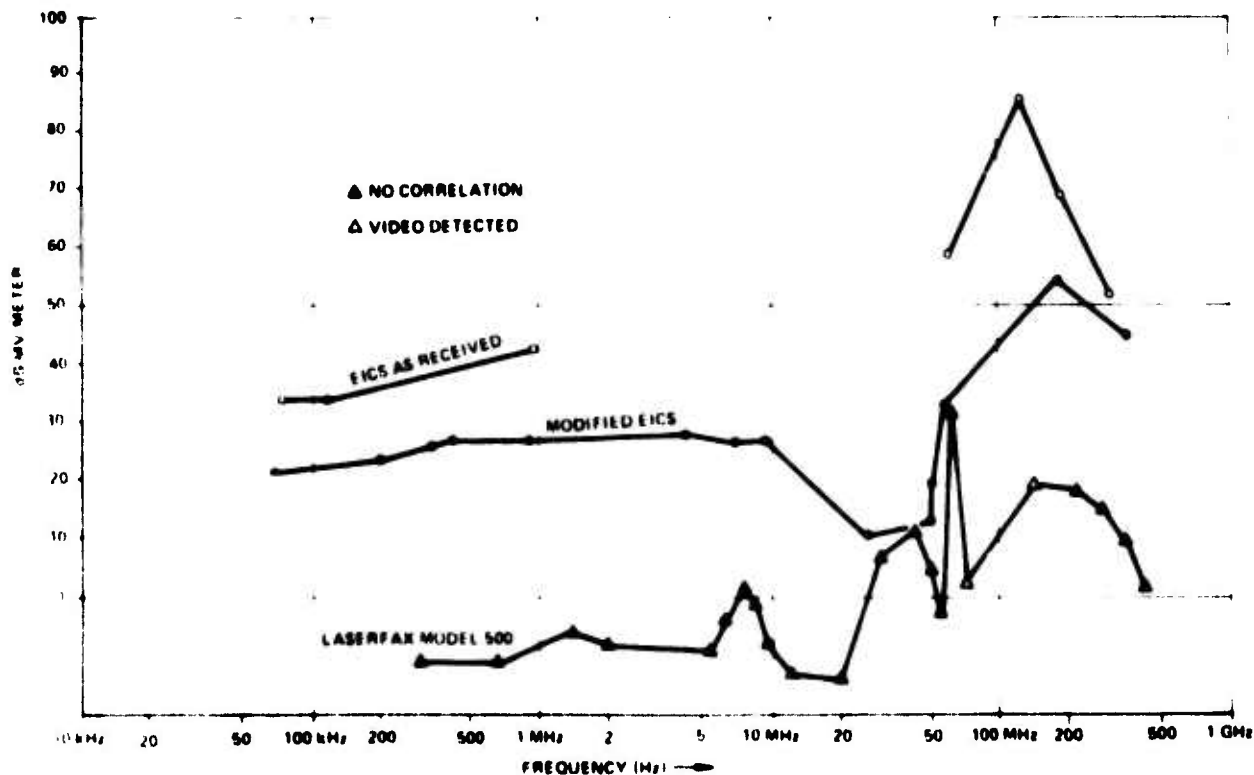
Figure 3.16. EICS and Laserfax TEMPEST Tests
