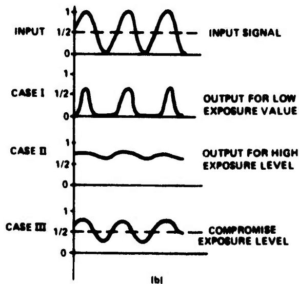
Figure 3.2. Image Scanning Input/Output Responses
