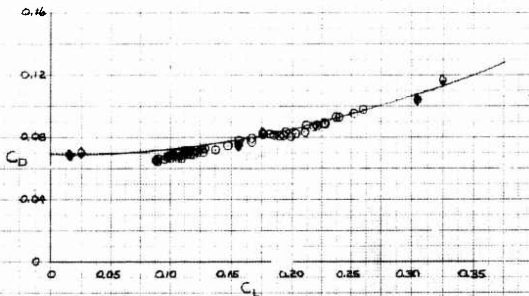
Figure A1. Trim Performance Data For \delta_{up} = -40 degrees, \delta_{RB} = 0 degrees, \delta_{AB} = 7 degrees.
