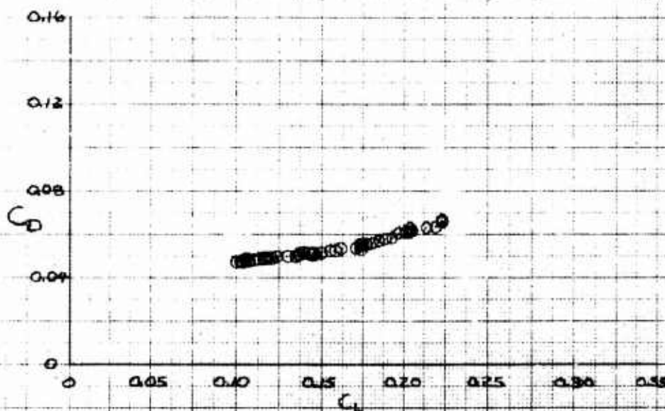
Figure A21. Trim Performance Data for \delta_{UB} = -28 degrees \delta_{AB} = -10 degrees, \delta_{AB} = 7 degrees
