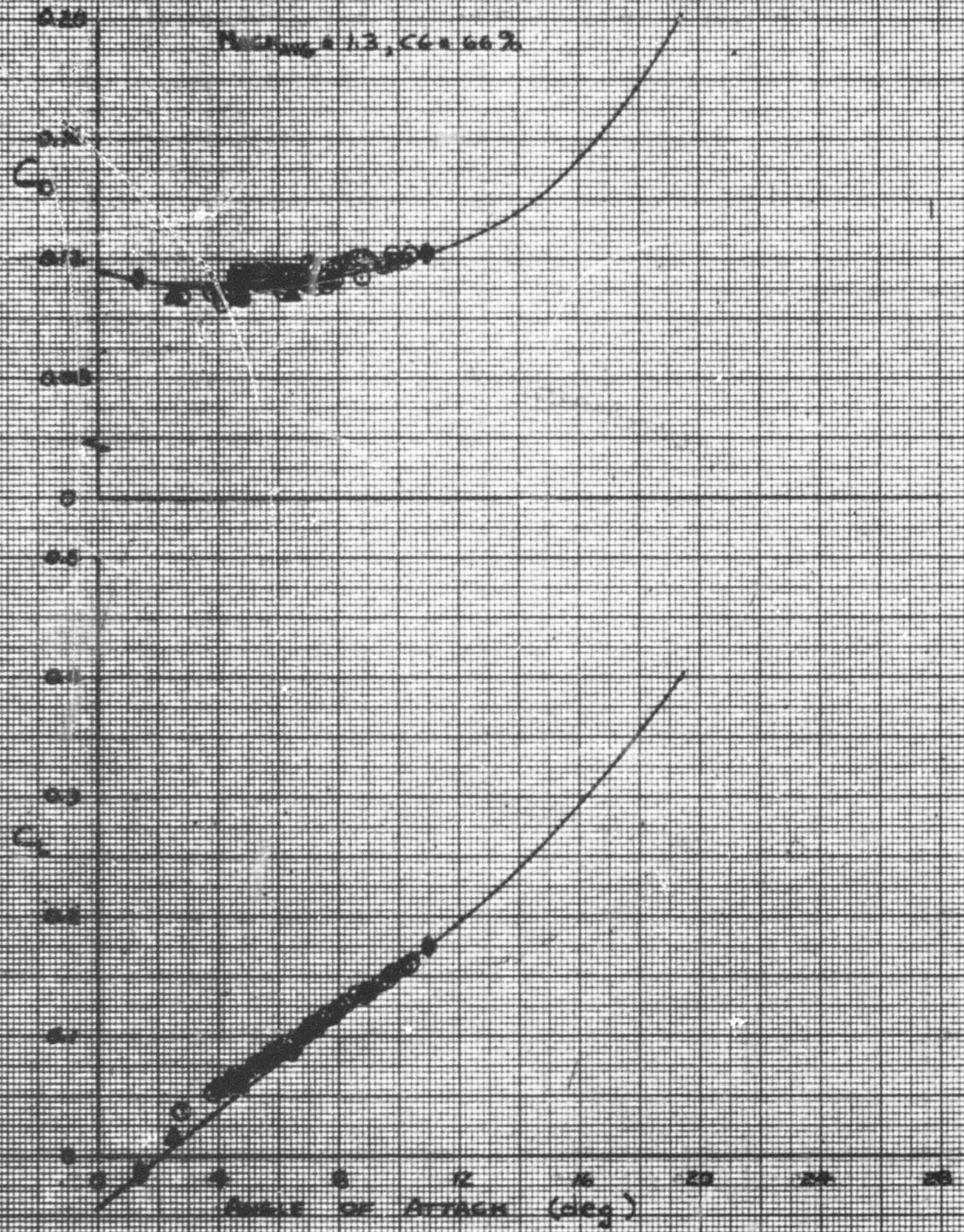
Figure A9 Concluded
