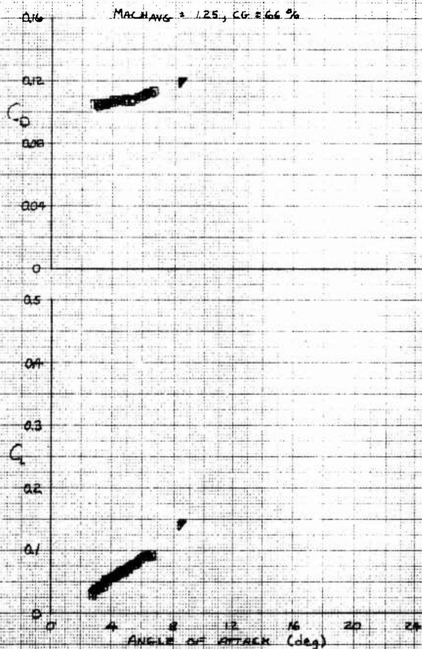
Figure A32. Concluded
