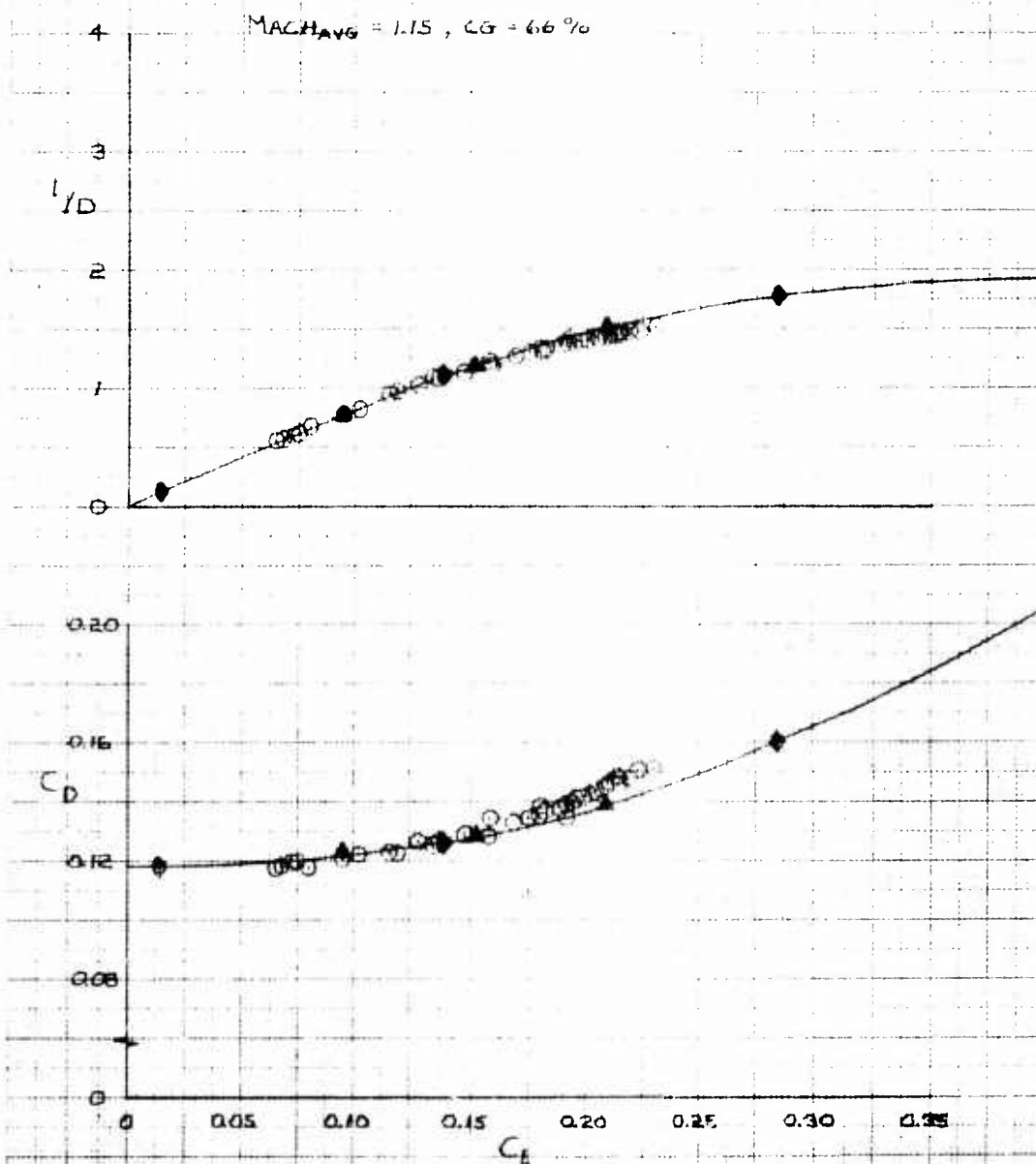
Figure AB Trim Performance Data for \alpha_{LB} = -40 degrees, \alpha_{RB} = 0 degrees, \alpha_{MB} = 7 degrees
