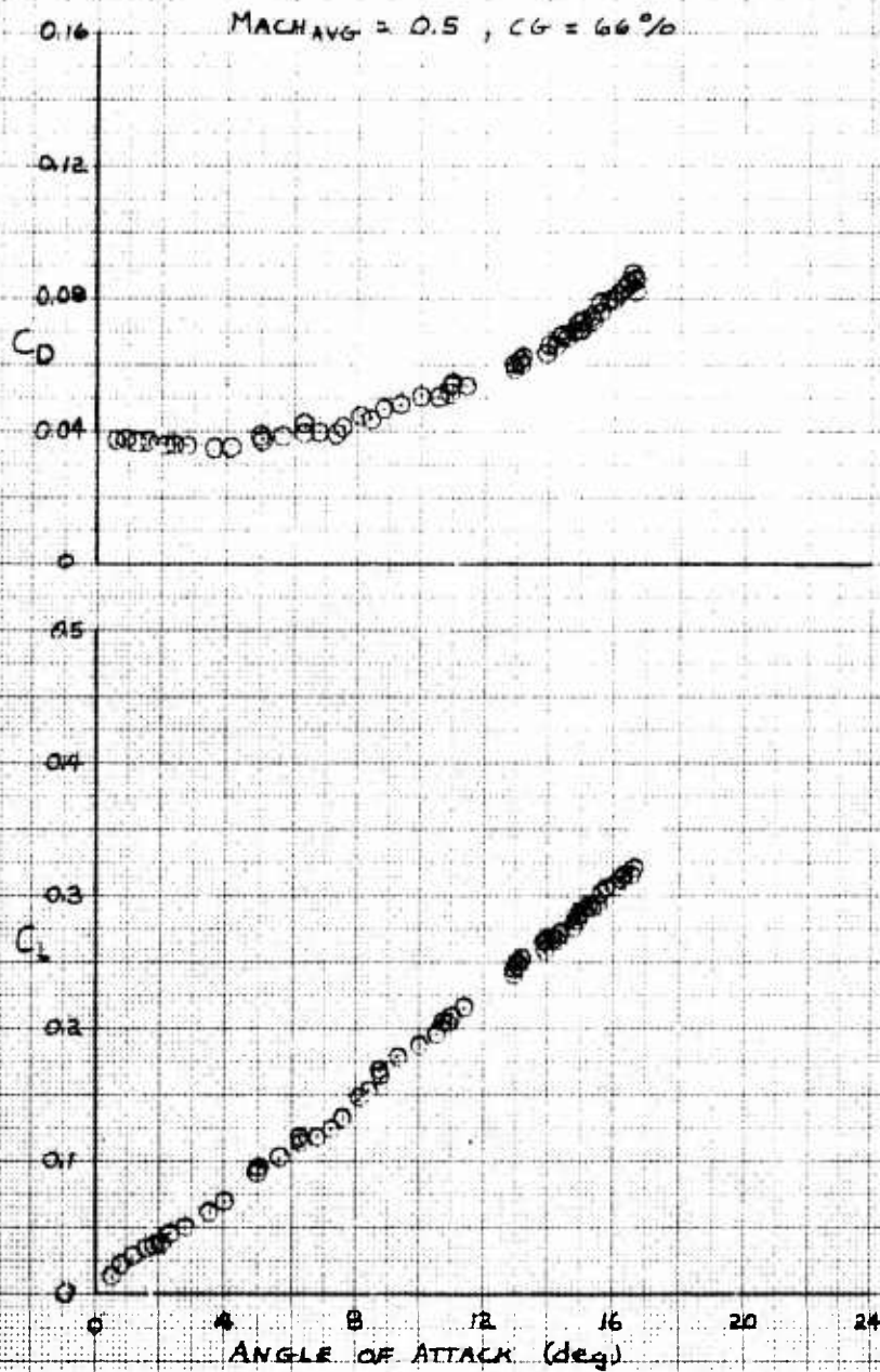
Figure A22 Concluded
