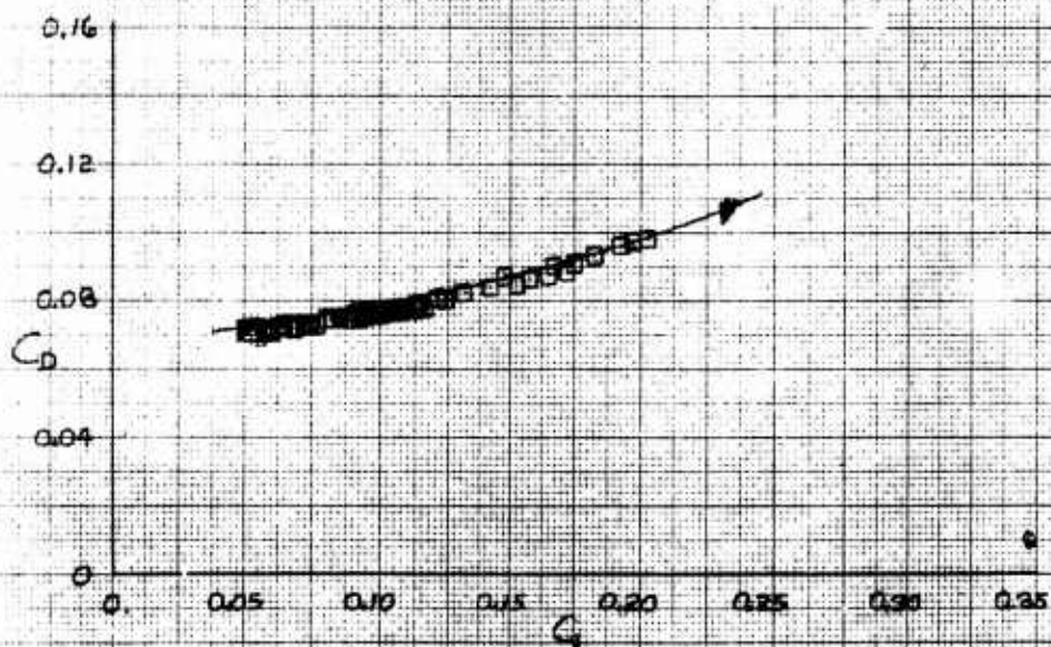
Figure A31 Trim Performance Data for \delta_{uB} = +40 degrees, \delta_{eL} = 24 degrees, \delta_{rB} = 0 degrees
