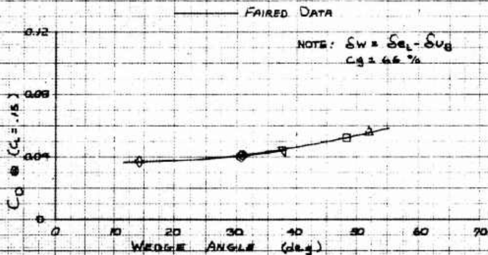
Figure 14. Drag Coefficient versus Wedge Angle
