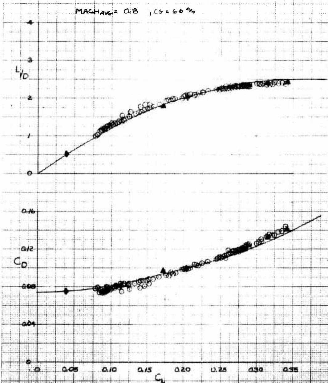
Figure A4: Trim Performance Data for \delta_{UB} = -40 degrees, \delta_{RB} = 0 degrees, \delta_{AB} = 7 degrees
