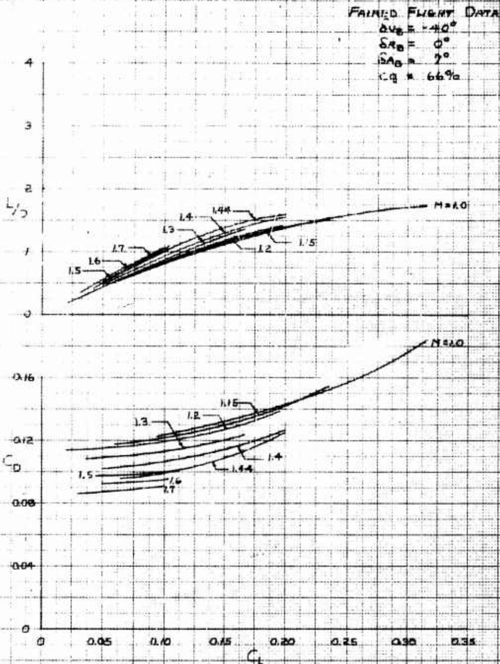
Figure 7. Mach Number Effects for the Transonic Configuration - M \geq 1.0
