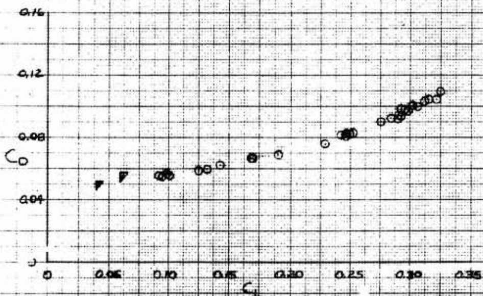
Figure A17. Trim Performance Data for \delta_{1/2} = -30 degrees, \delta_{2/2} = 0 degrees, \delta_{3/2} = 7 degrees
