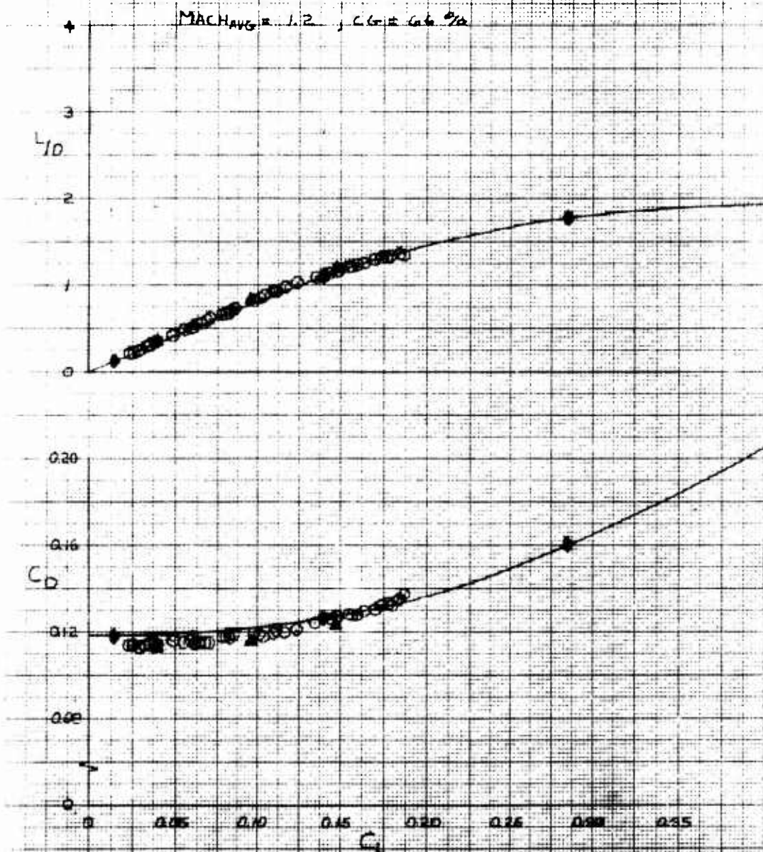
Figure A9. Thin Airfoil Performance Data for \delta_{UB} = -40 degrees, \delta_{RB} = 0 degrees, \delta_{AB} = 7 degrees.
