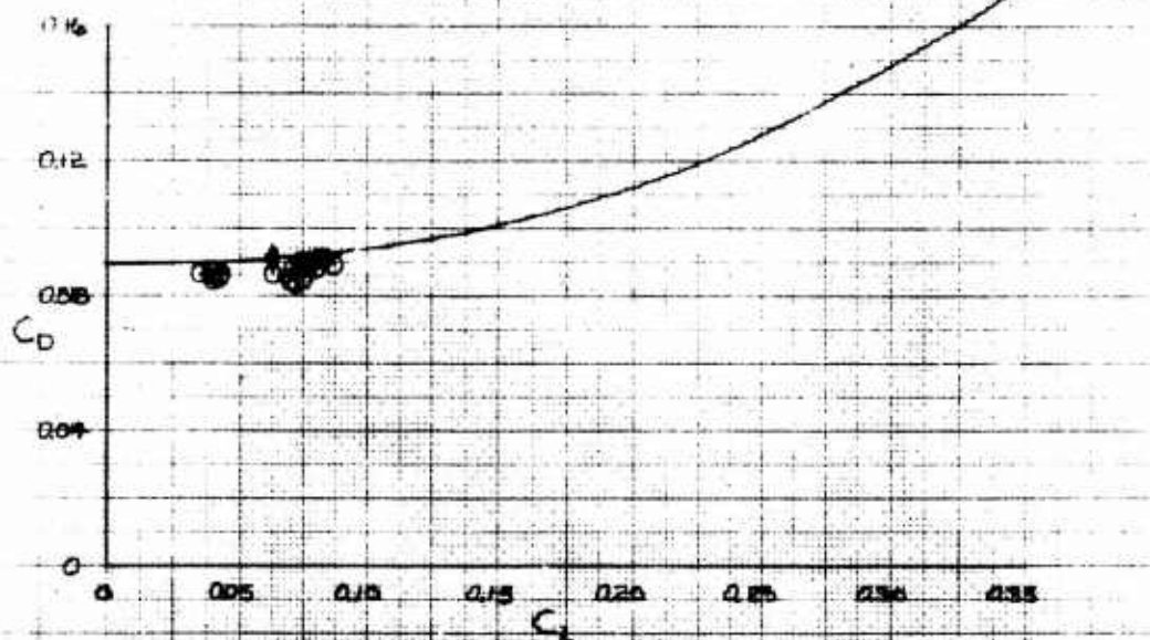
Figure A15 Trim Performance Data for \delta_{1/2} = -40 degrees, \delta_{R_0} = 0 degrees, \delta_{A_0} = 7 degrees
