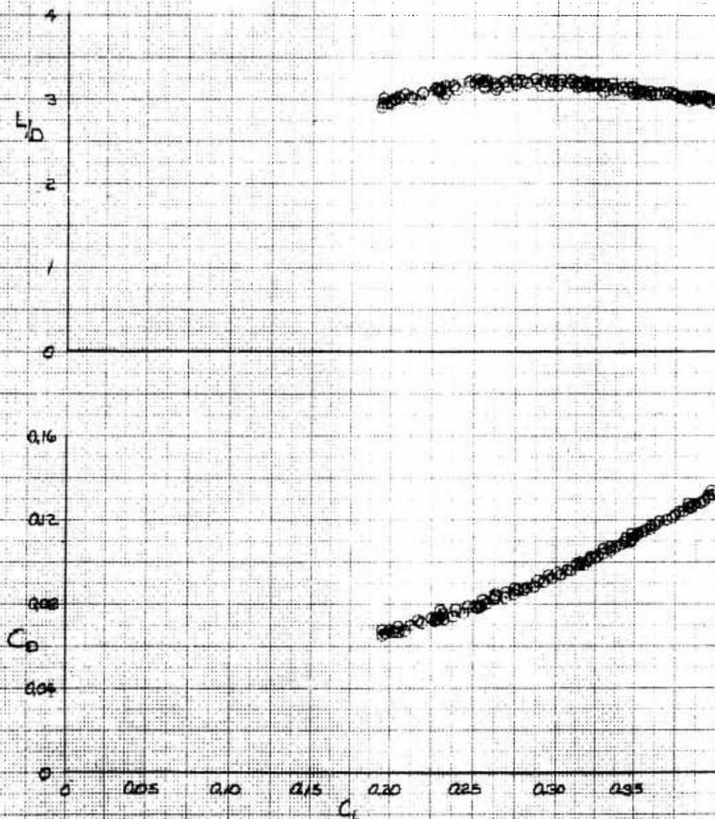
Figure A20 Trim Performance Data for \delta_{UG} = -29 degrees, \delta_{RG} = 0 degrees, \delta_{AG} = 7 degrees
