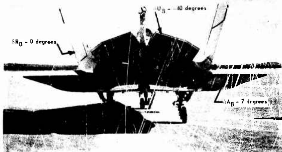
Transonic Configuration
