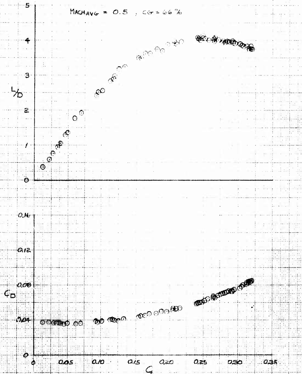
Figure A22 Trim Performance Data for \delta_{uB} = -23 degrees, \delta_{wB} = -10 degrees , \delta_{\theta B} = 7 degrees
