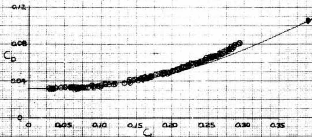
Figure A24 Trim Performance Data for S_{u_0} = +20 degrees, S_{R_0} = -10 degrees, S_{A_0} = 7 degrees
