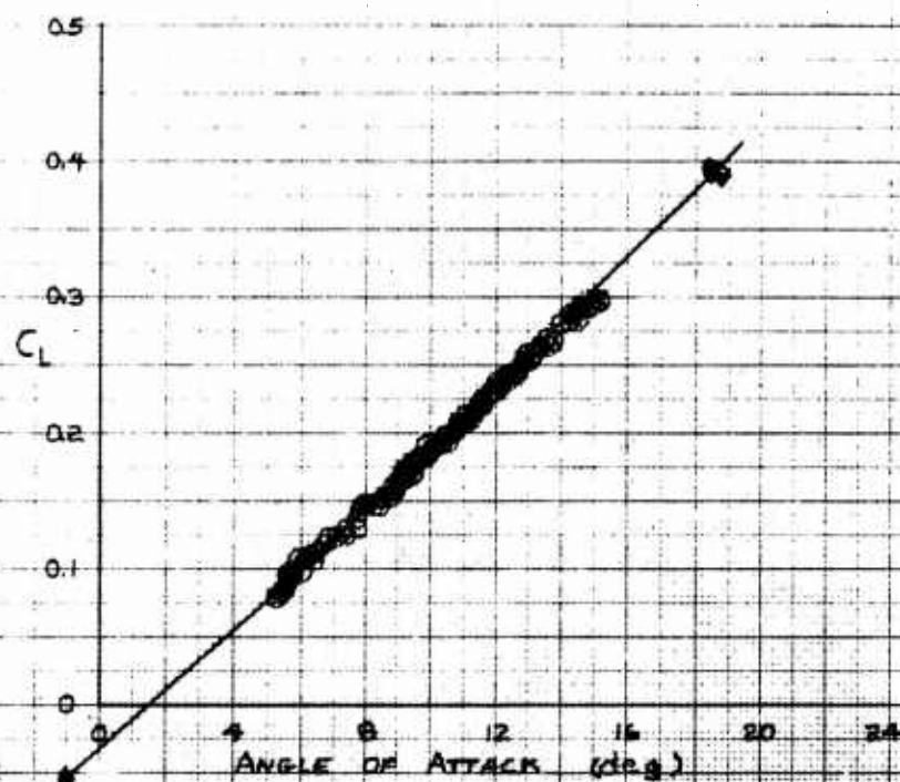
Figure A23. Concluded
