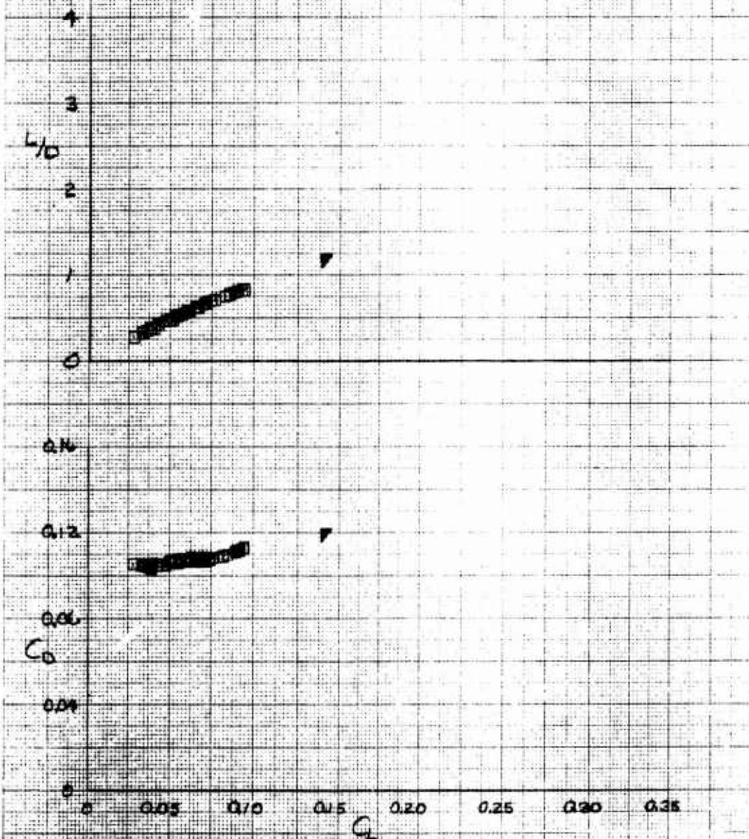
Figure A32 Trim Performance Data for \delta_{UB} = -40 degrees, \delta_{CL} = 20 degrees, \delta_{RE} = 0 degrees
