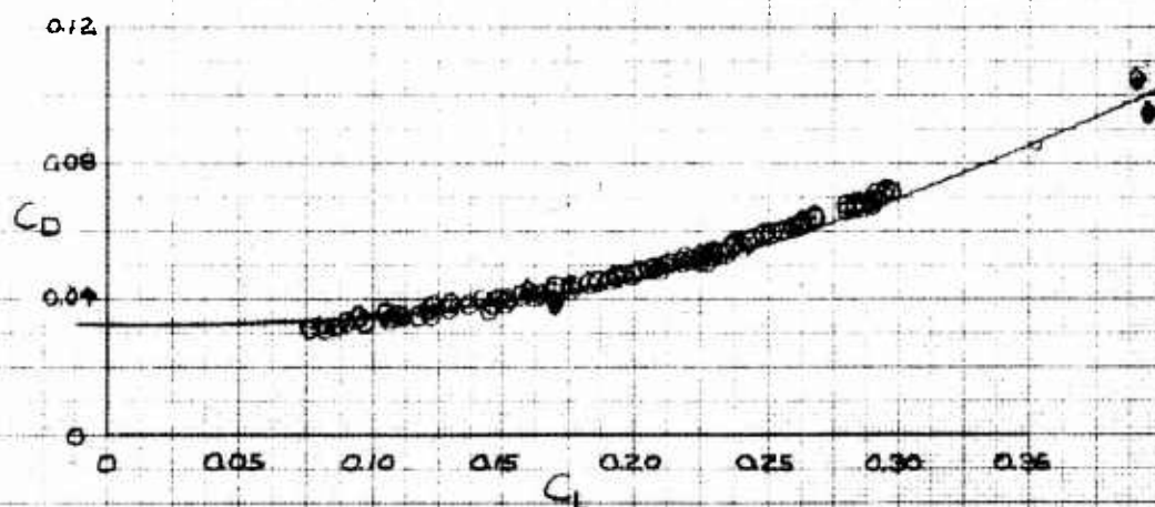
Figure A23 Trim Performance Data for \delta_{UG} = -20 degrees, \delta_{LG} = -10 degrees, \delta_{AG} = 7 degrees
