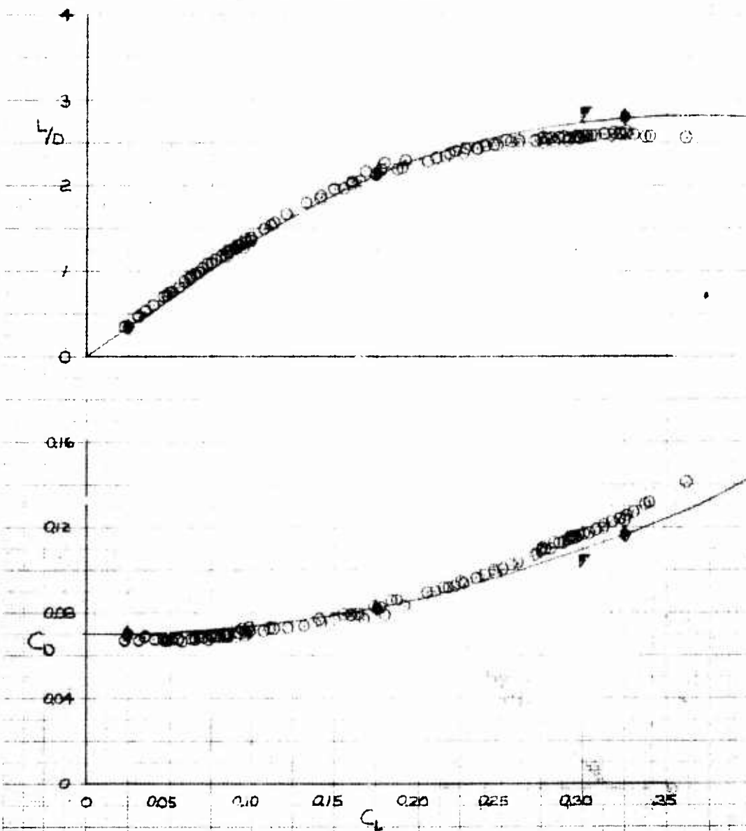
Figure A2 Trim Performance Data For \delta_{UB} = -40 degrees, \delta_{PL} = 0 degrees , \delta_{AB} = 7 degrees
