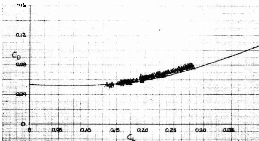
Figure A30 Gear-Down Trim Performance Data for S_{\alpha_B} = -20 degrees, S_{\alpha_L} = -10 degrees, S_{\alpha_B} = 7 degrees
