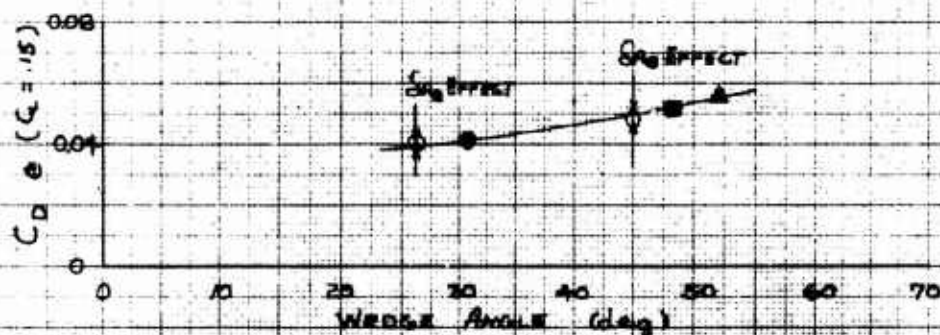
Figure 17. Effect of Wedge Angle and Aileron Bias on Performance
