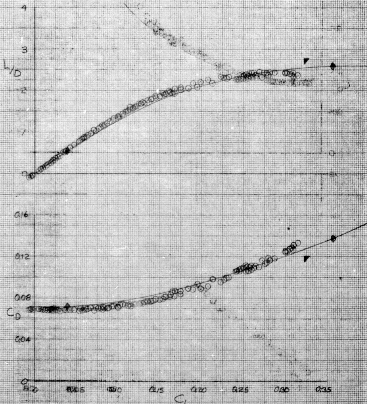
Figure A3. Trim Performance: Data for \delta_{UB} = -10 degrees, SR_B = 0 degrees, SA_B = 7 degrees
