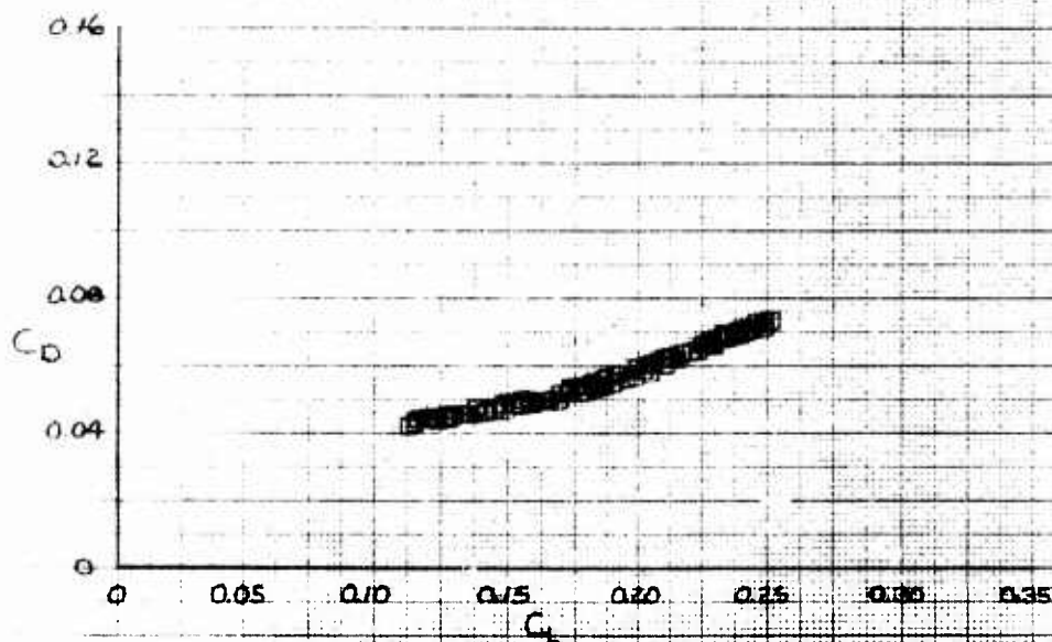
Figure A33 Trim Performance Data for \delta_{u3} = -29 degrees, \delta_{e1} = 16 degrees, \delta_{a3} = -10 degrees
