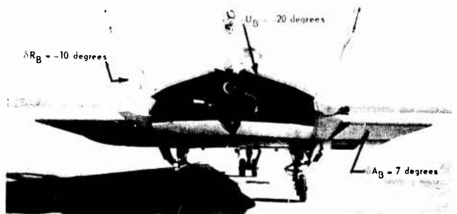
Subsonic Configuration
