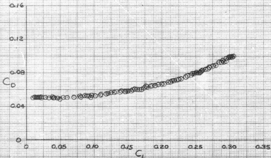
Figure A19. Trim Performance Data for \delta_{UB} = -30 degrees, \delta_{RB} = -10 degrees, \delta_{AB} = 7 degrees
