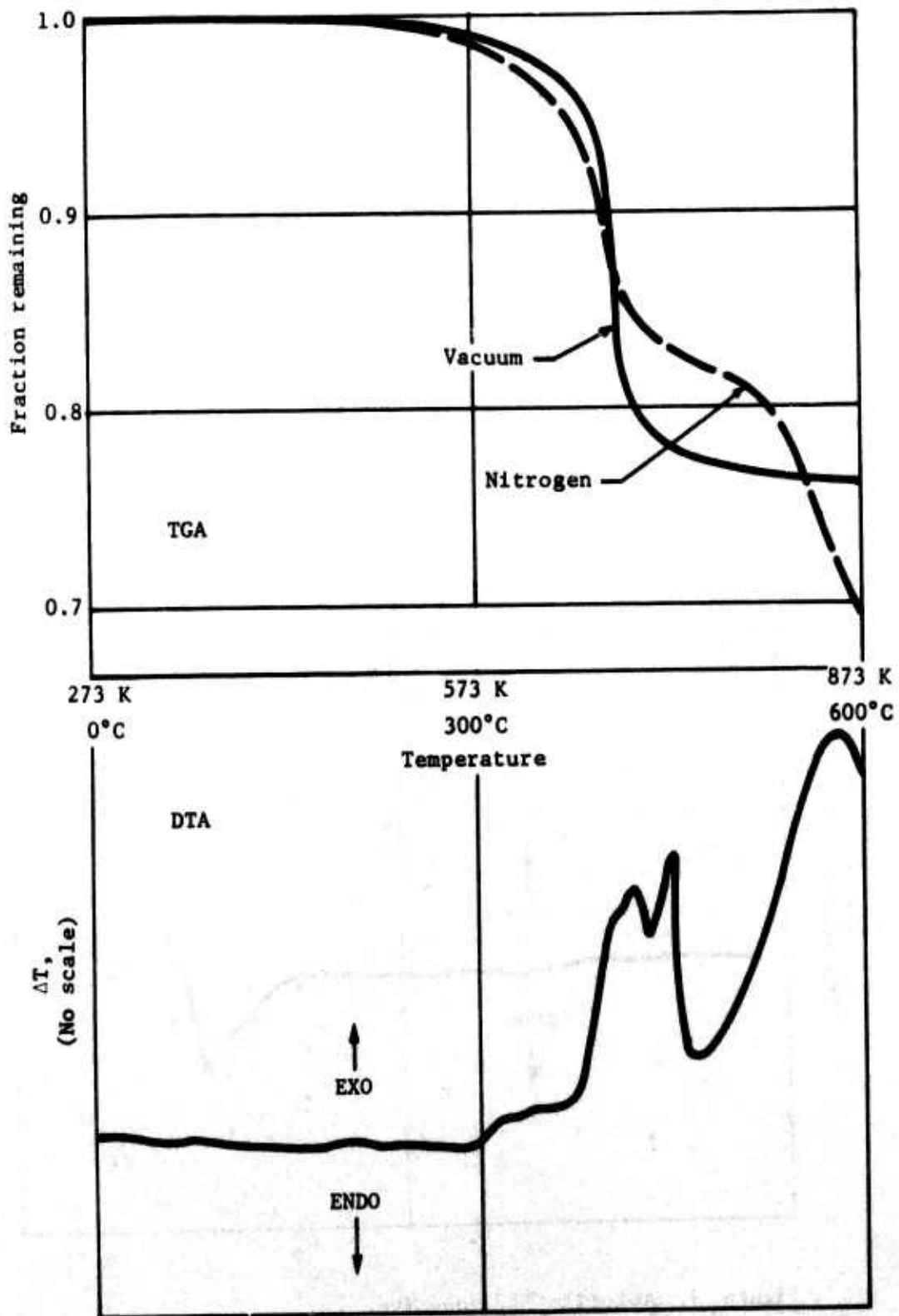
Figure 4. Epotek H-31 adhesive.
