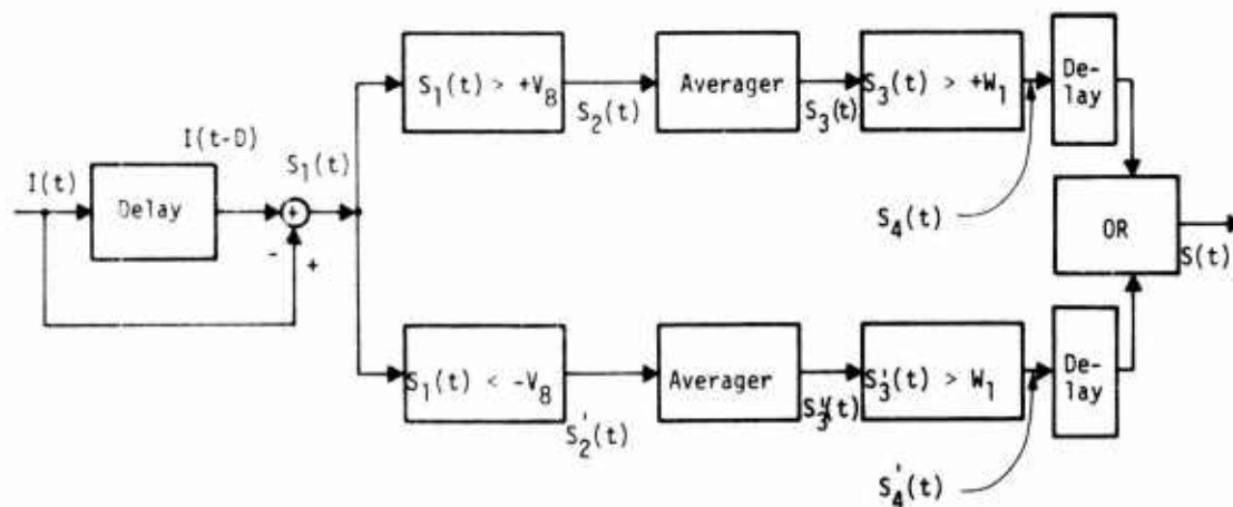
Figure 7. Step Filter
