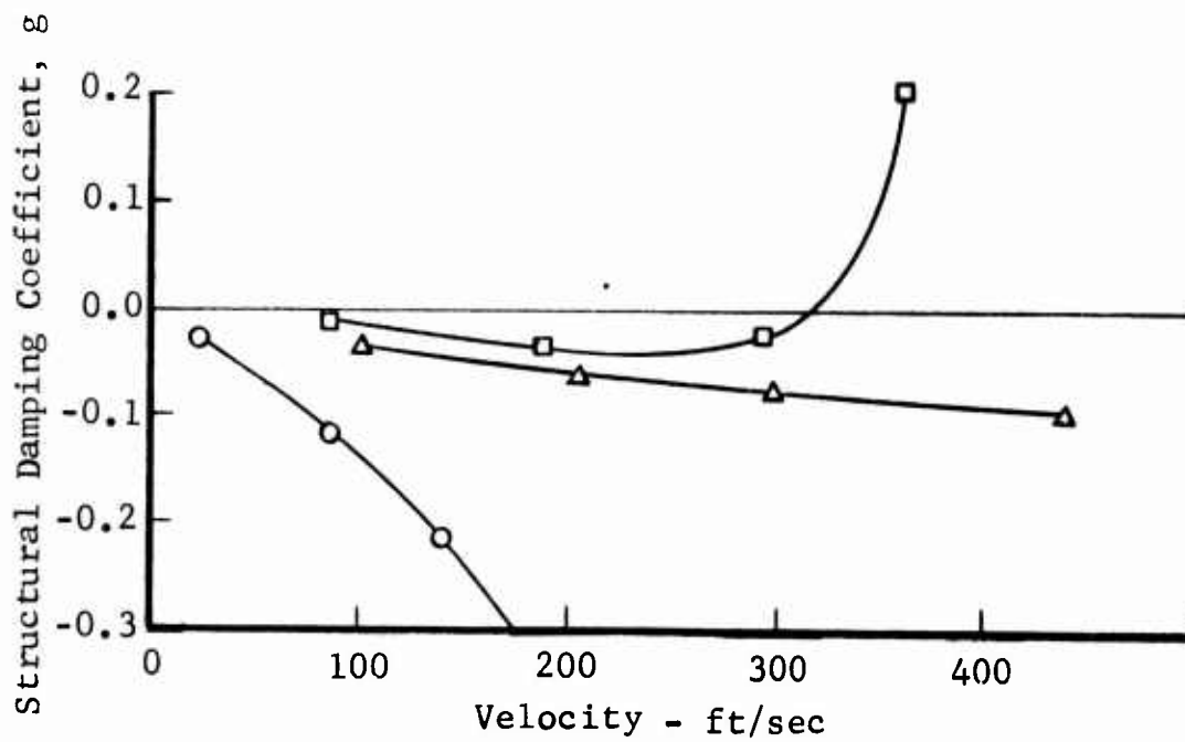
Figure 18 Structural Damping Coefficient and Frequency Versus Velocity for Cantilever Model
