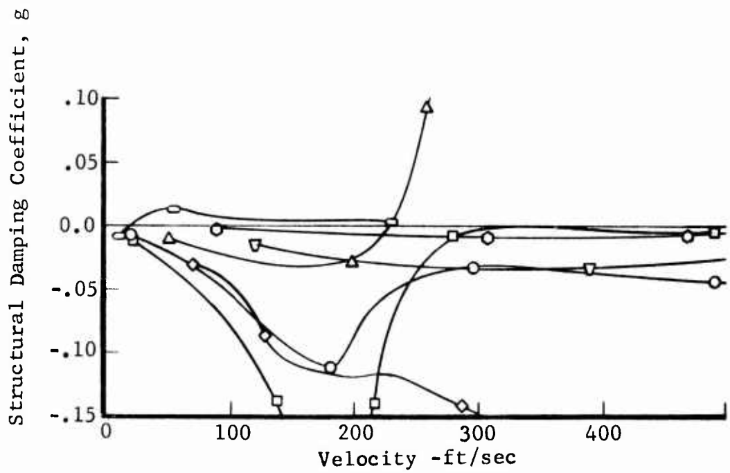
Figure 23 Structural Damping Coefficient and Frequency Versus Velocity for TFW Trim Surface Aft Model (Doublet-Lattice)
