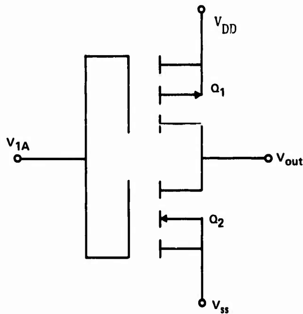
FIG. 14 INVERTER DIAGRAM
