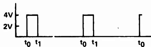
FIG. 13 VCO WAVEFORMS
