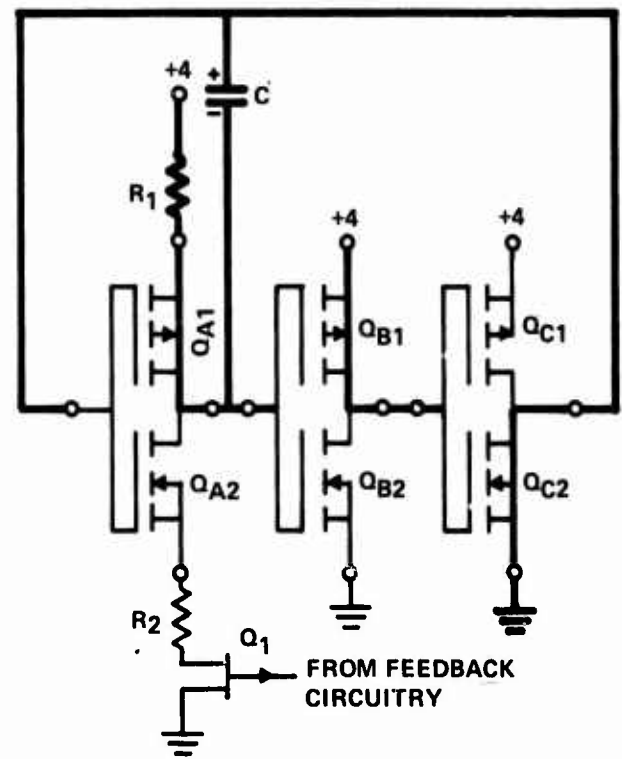
(b) INVERTER B OUTPUT HIGH
