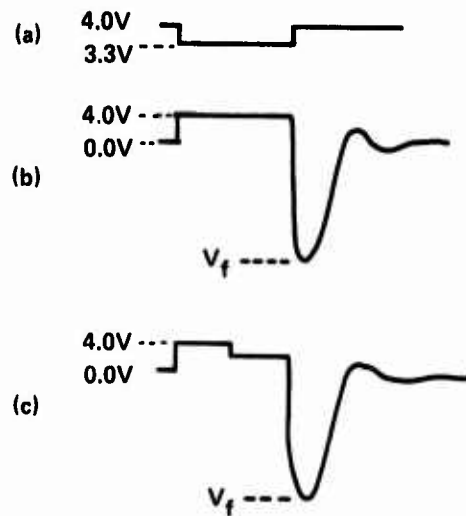
FIG. 11 CORE DRIVE CIRCUIT AND ASSOCIATED WAVEFORMS
