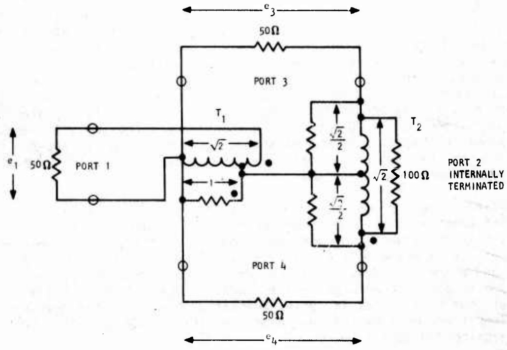
(b) 3-PORT, WITH EXTERNAL/INTERNAL TERMINATIONS
