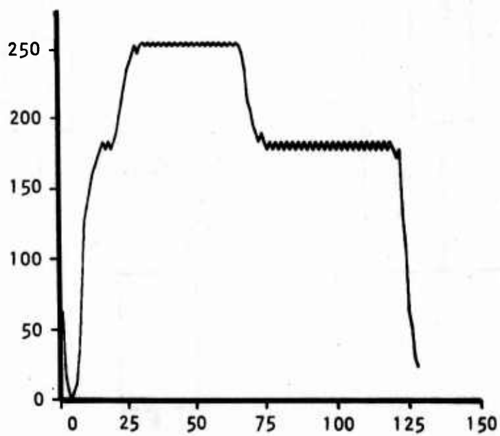
(b) CODED SYNC SIGNAL
