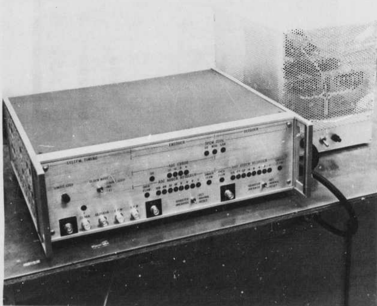
Figure 14. Video Encoder/Decoder Breadboard and Power Supply Unit
