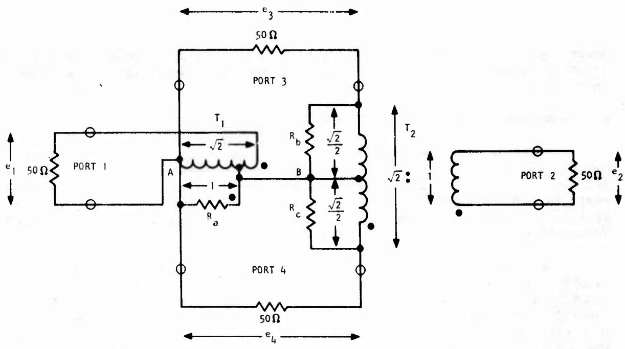
(a) 4-PORT, WITH EXTERNAL TERMINATIONS
