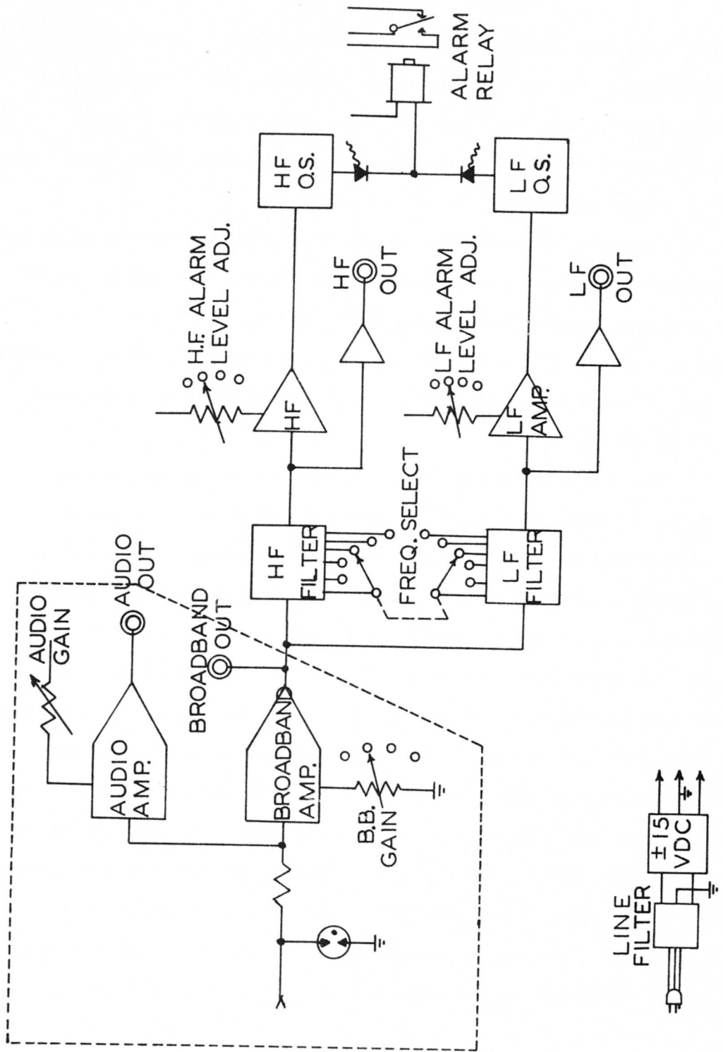
FIGURE 2-3. Block Diagram of Processor/Display Console
