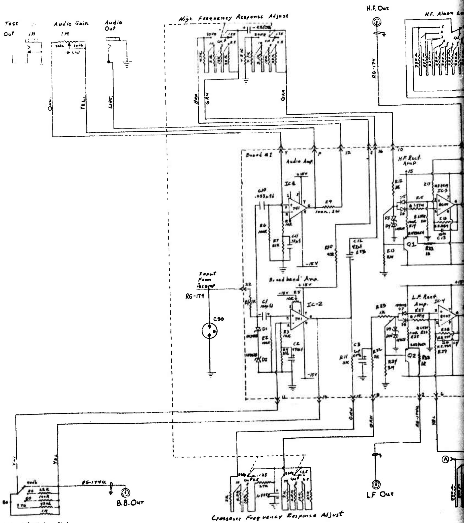
Figure A4- Schematic Diagram of Console.
