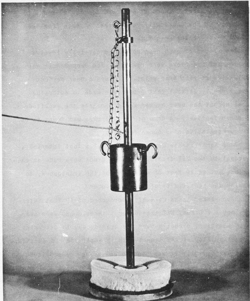
FIGURE 5-4. Drop Hammer
