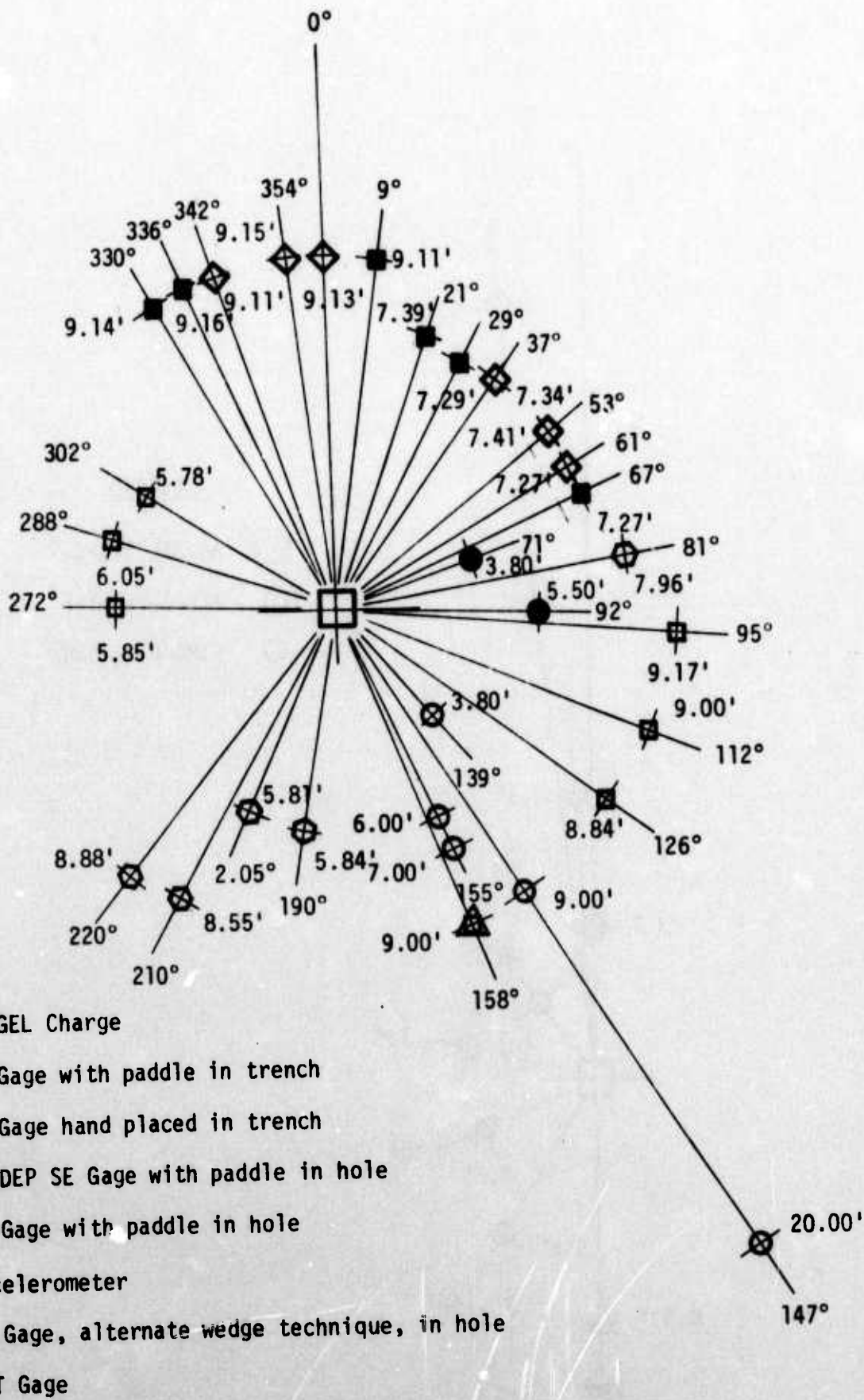
Figure P-15. SCAL III Instrumentation Layout
