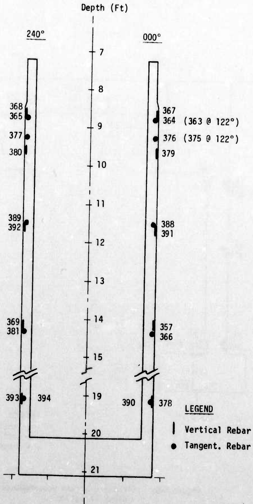
Figure P-5b. Structure Strain Measurements - Lower Structure
