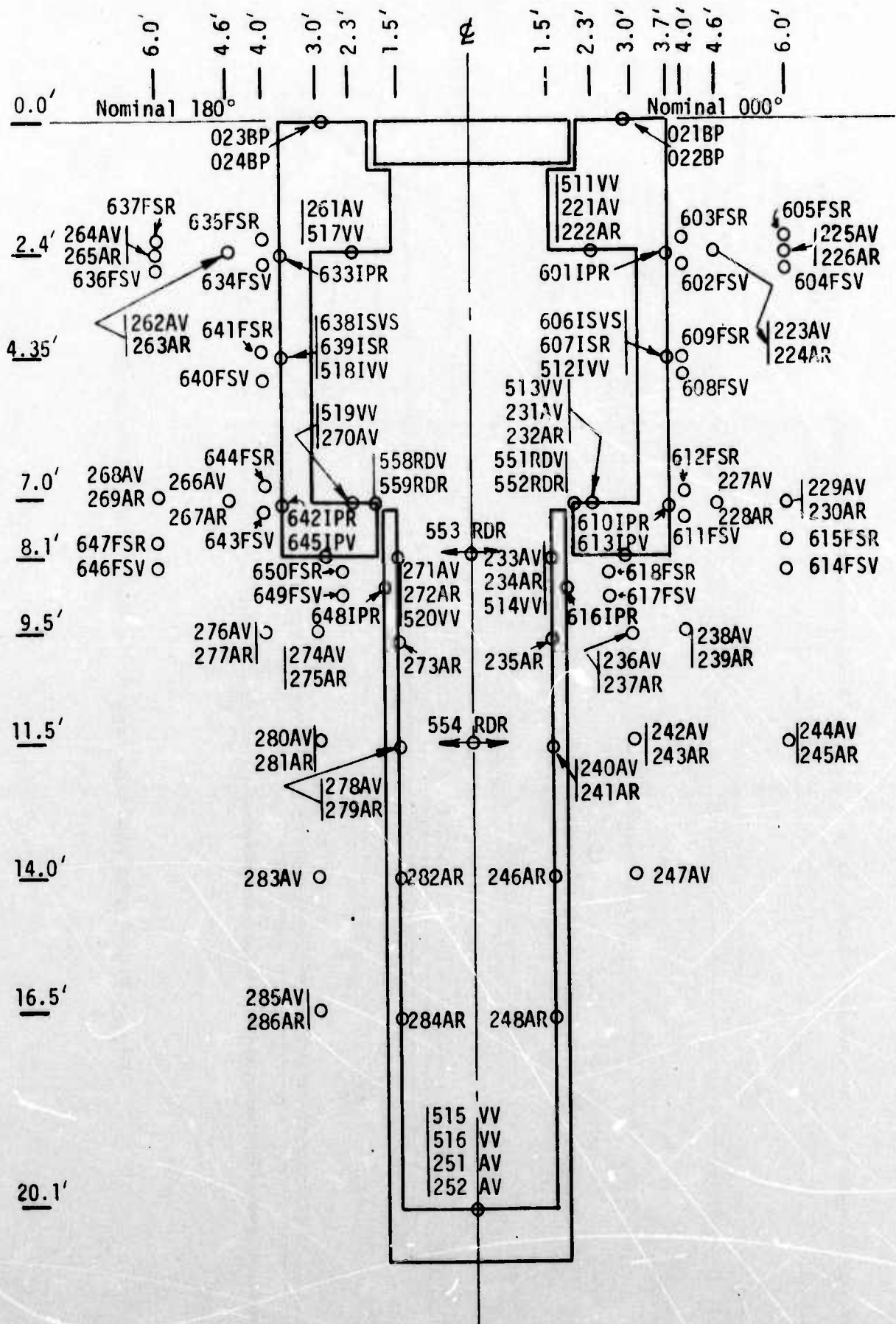
Figure P-10. Structure and Near Field Motion and Stress Measurements - HP I-2A (000° and 180° Radials)
