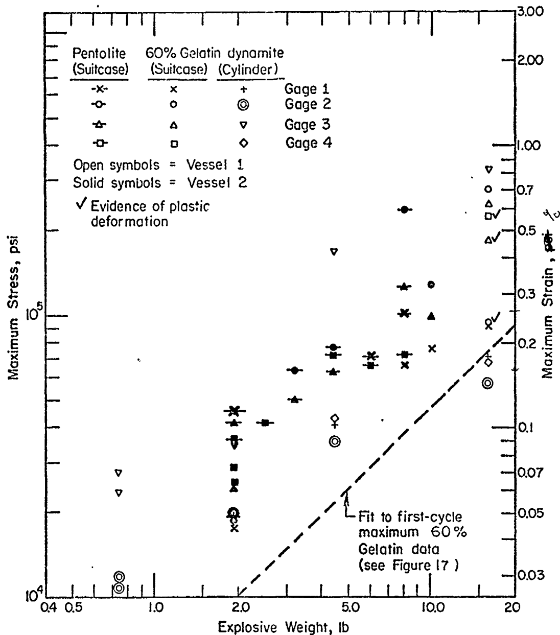
FIGURE 20. MAXIMUM STRAINS IN THE 4.5-FT-DIAMETER VESSELS FOR VARIOUS CHARGES
