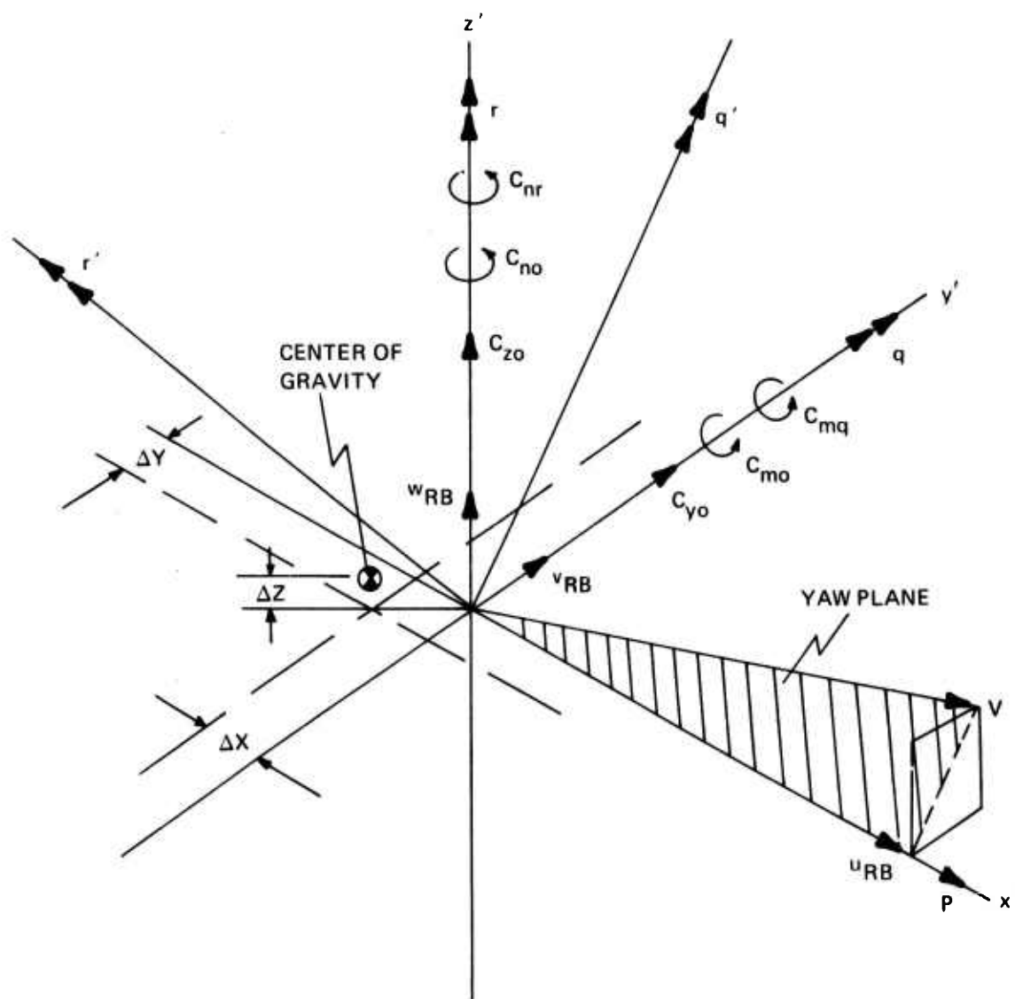
Figure 4. Damping Moment and Body-Fixed Force-Moment Definition
