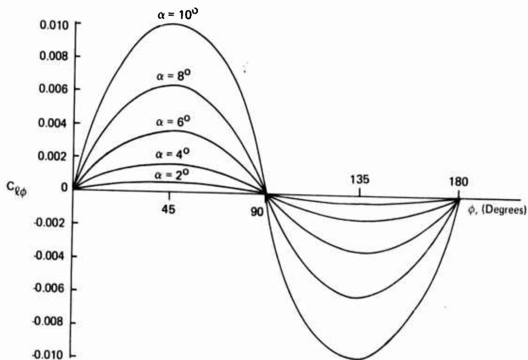
Figure 13. Induced Roll Moment Coefficient versus \phi
