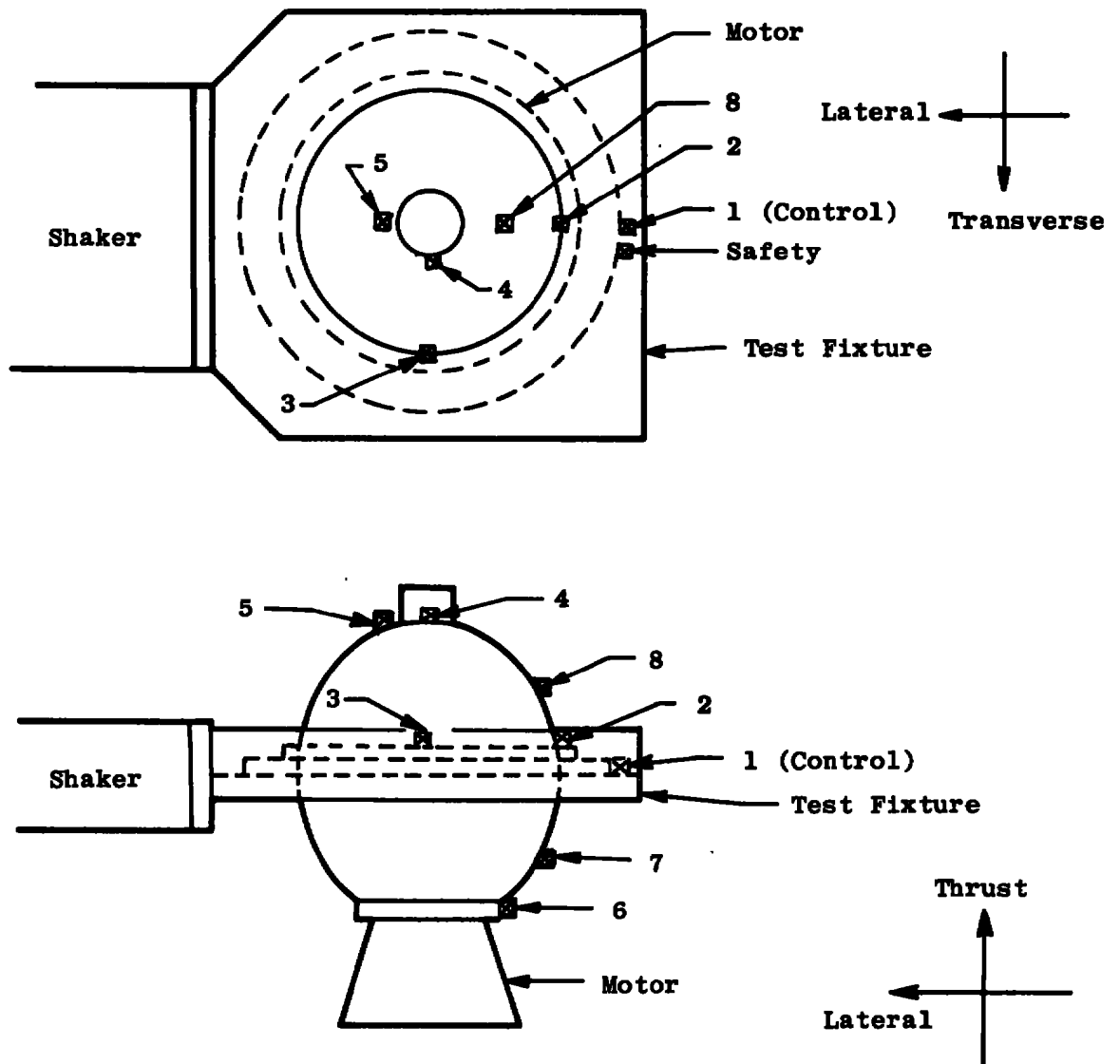
Figure 3. Accelerometer locations and designations.
