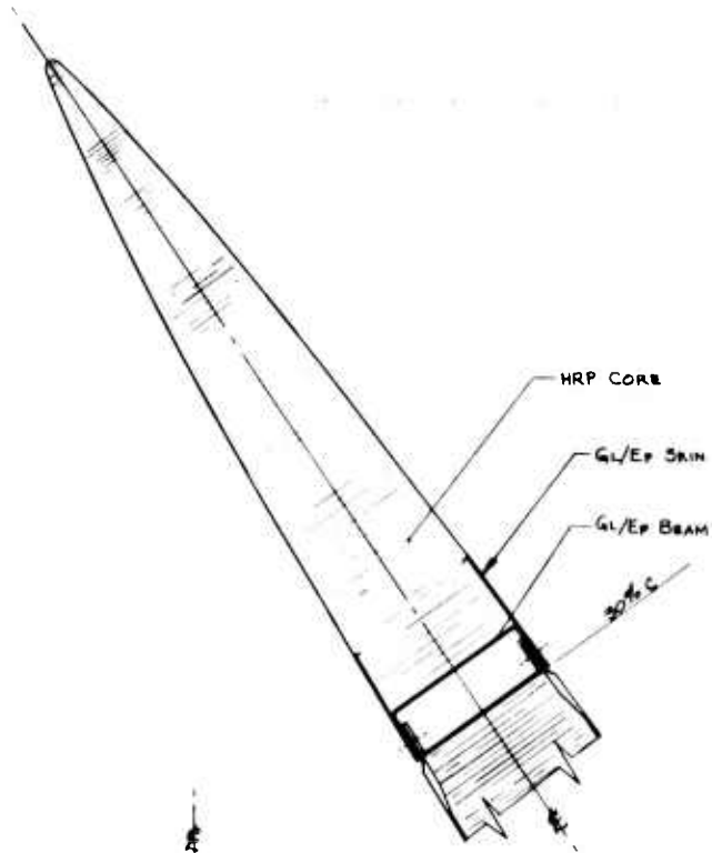
SECT. A-A HALF SCALE
