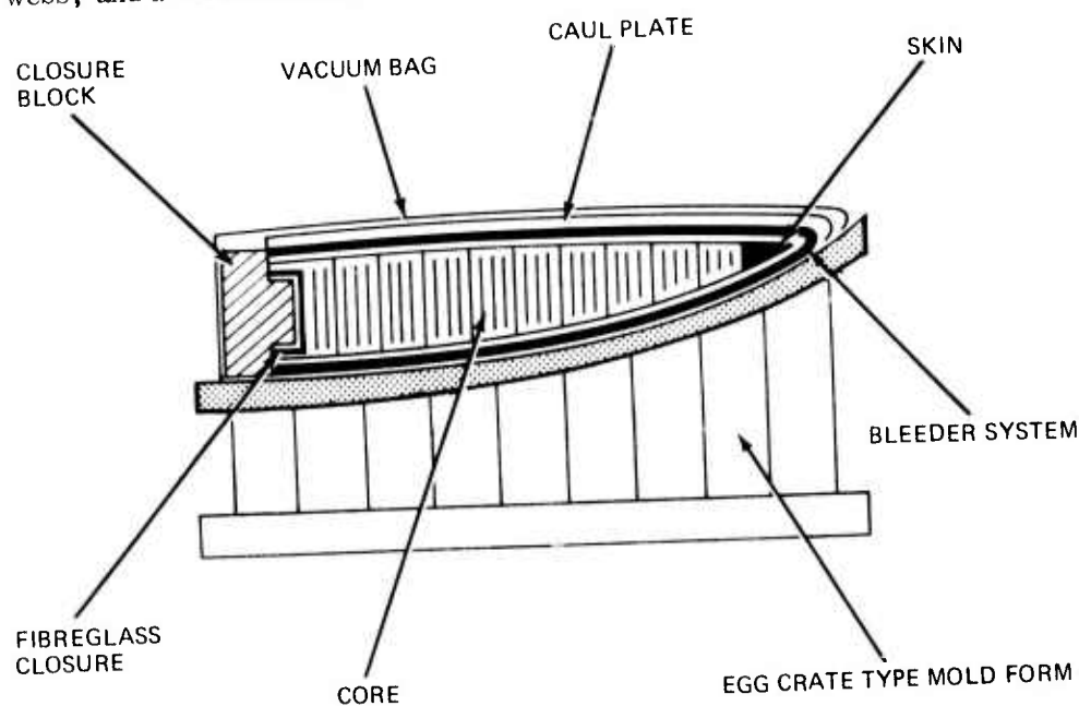
Figure 13. Layup and Tooling for Cocuring a Trailing Edge Assembly
