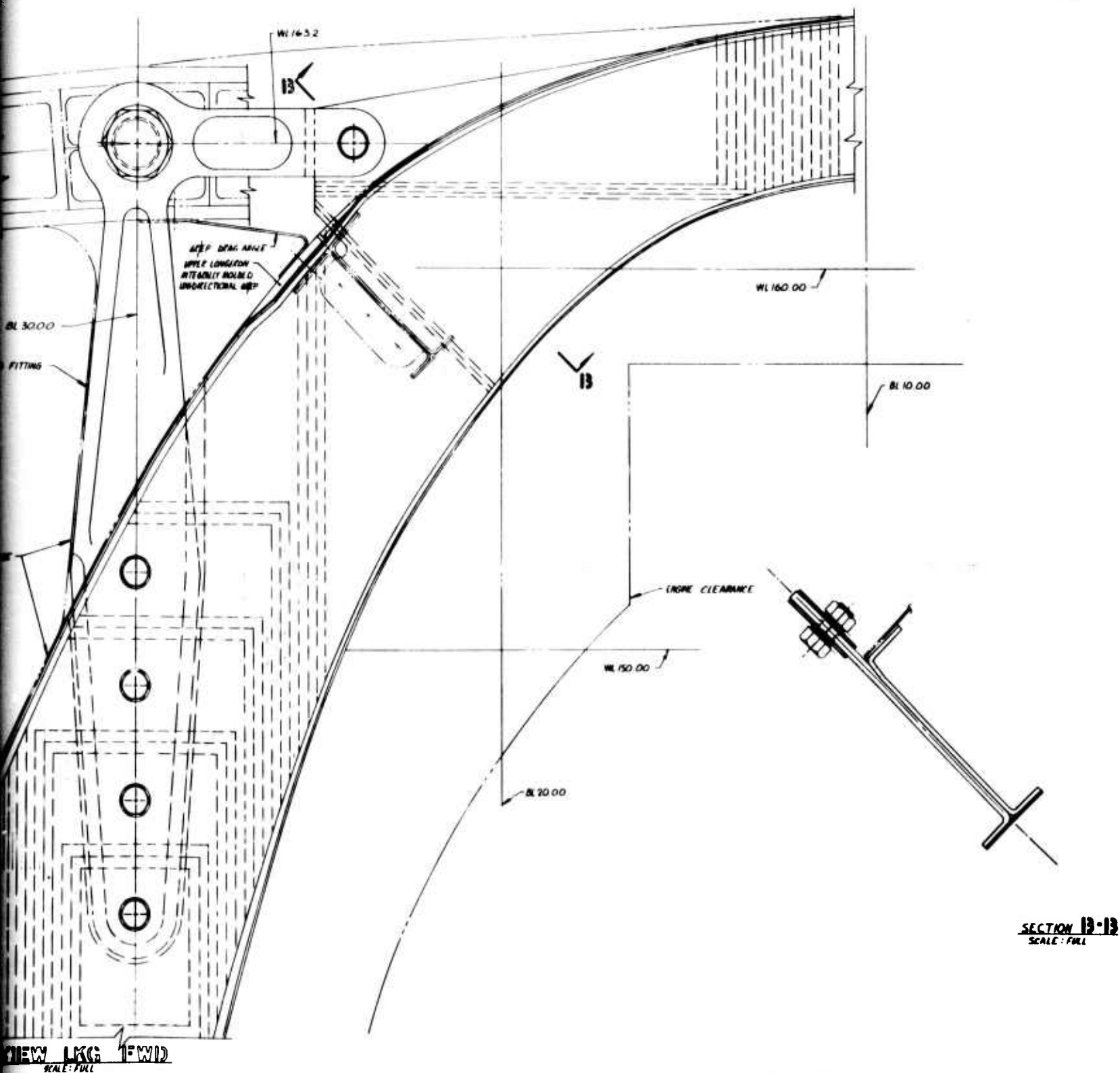
Figure 25. ADCA Wing/Fuselage Attachment (Sheet 1 of 2)
