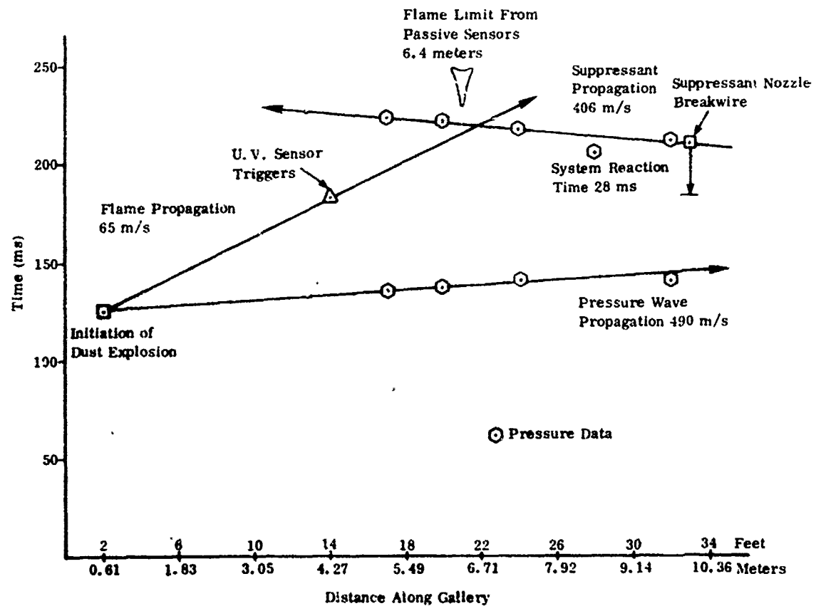
Figure 21. Test No. 41-5-01 Halon Suppressant
