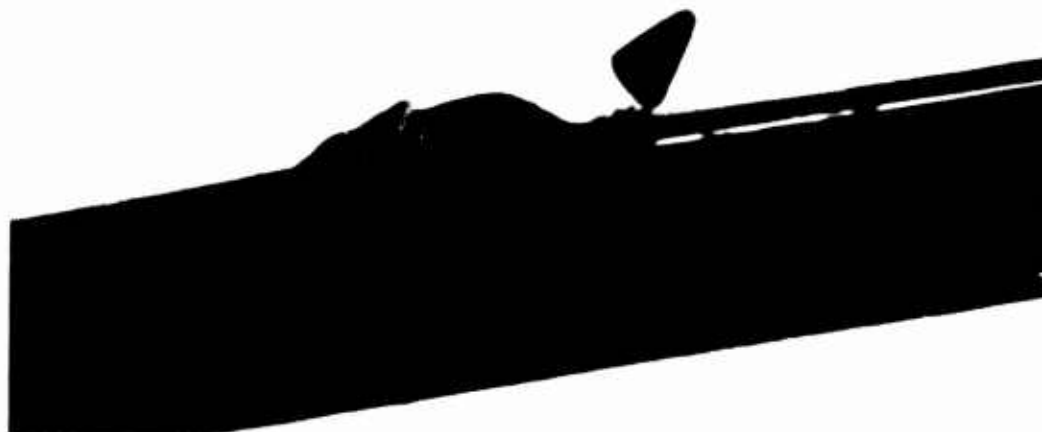
Figure B-8. Flash X-Ray - Mod III Fuze with 0.04-inch-Walled 17-4PH Ogive and HEI-Loaded Projectile Assembly 119 Microseconds (5.0-inch delay) after 3560-ft/s Impact with 0.09-inch Aluminum at 80-degree Obliquity (Note that the projectile is just beginning to detonate.)
