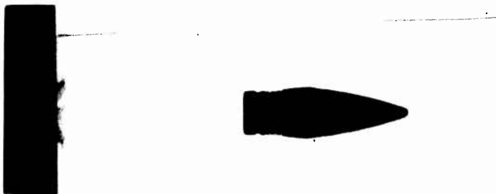
Figure B-9. Flash X-Ray - Mod III - Fuzed Projectile 6.8 Inches After 2584-ft/s Impact with 0.0625-inch Aluminum at 0-degree Obliquity (Note that the projectile has a slight bulge, indicating it is just beginning to function.)
