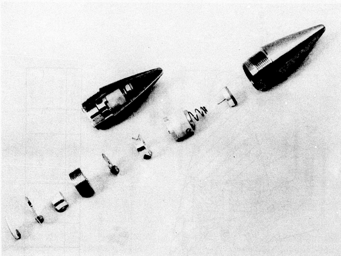
Figure B-5. XM714A3 Delay Function Fuze Exploded View
