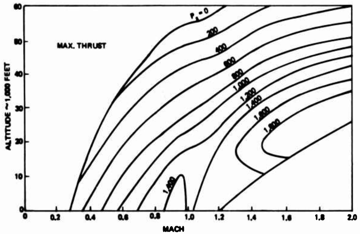
Figure E2. LES-202 (Canard) 1G \cdot P_s W/S = 120 PSF
