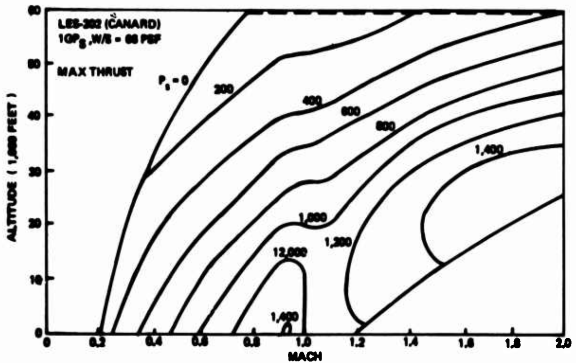
Figure E3. LES-202 (Canard) 1G \cdot P_s W/S = 66 PSF
