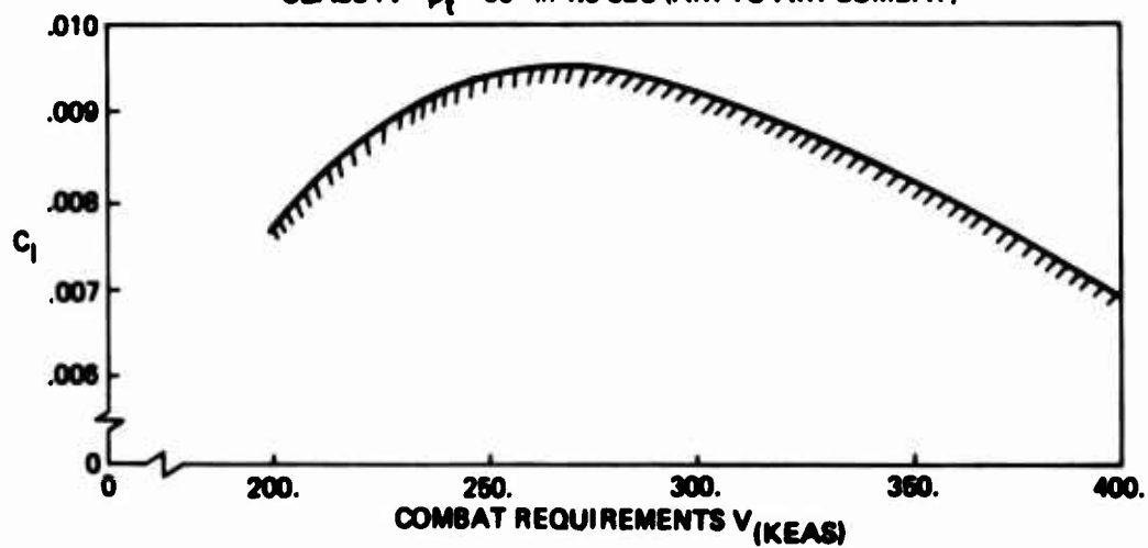
Figure 55. LES Roll Power Required
