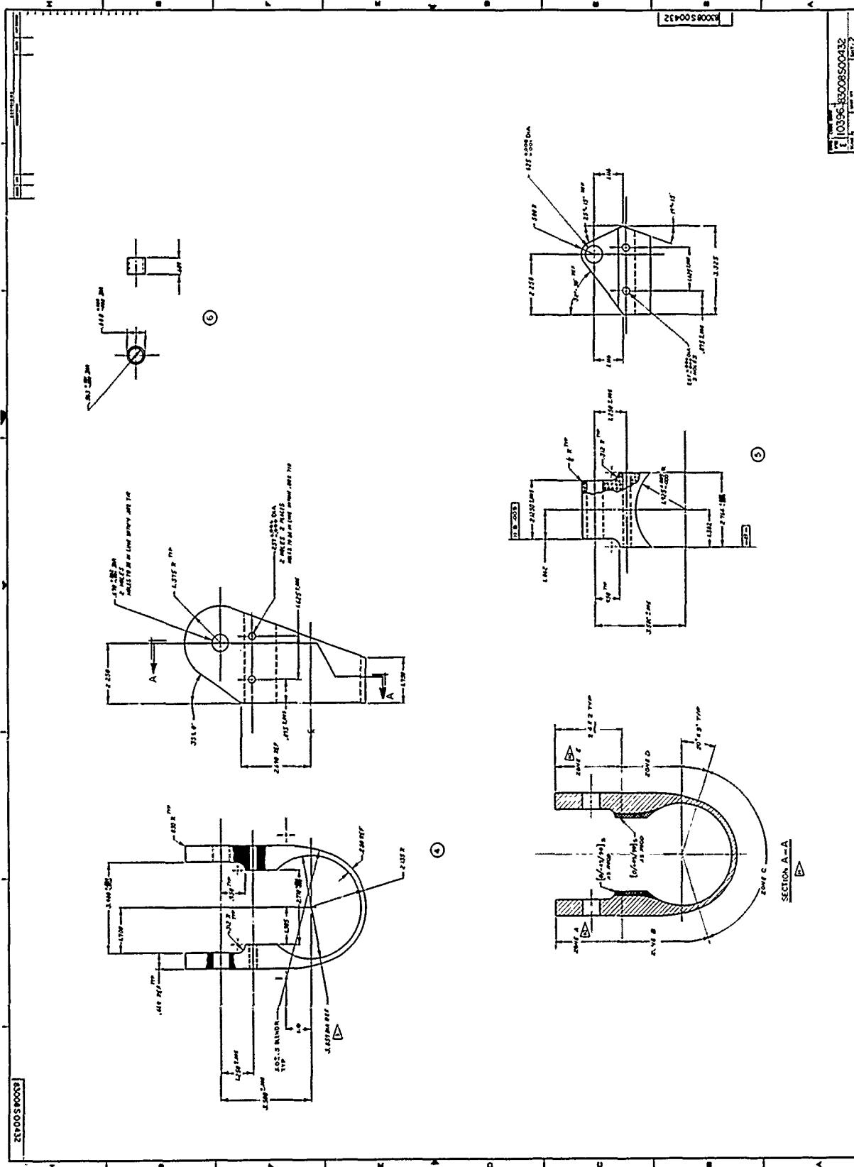
Figure 17. Torque Arm Attachment, Drawing 83008S00432 (Sheet 2 of 2)
