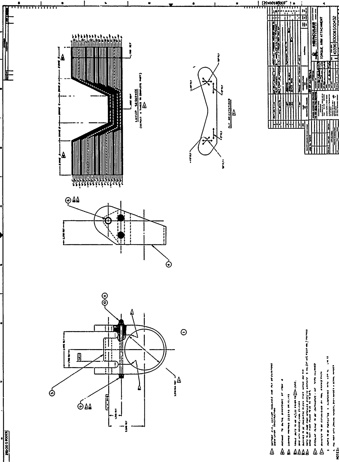
Figure 23. Torque Arm Attachment, Drawing 83008S00432, Sheet 1 of 2
