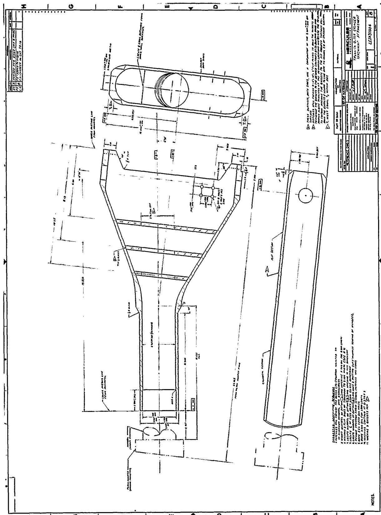
Figure 9. Design 2, A37B Graphite Composite Outer Cylinder/Trunion
