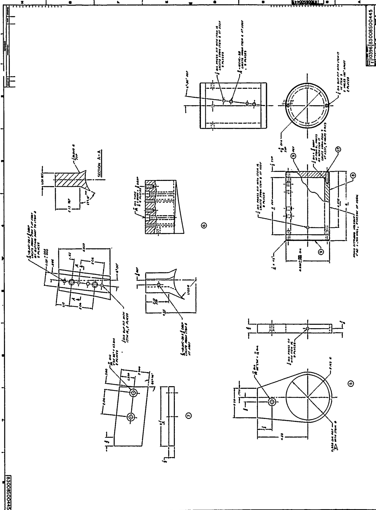
Figure 33. Layup Tool, Side Brace Attachment, Drawing 83008S00445, Sheet 2 of 2
