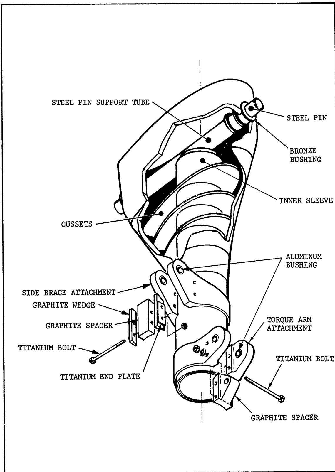
Figure 3. Outer Cylinder/Trunnion
