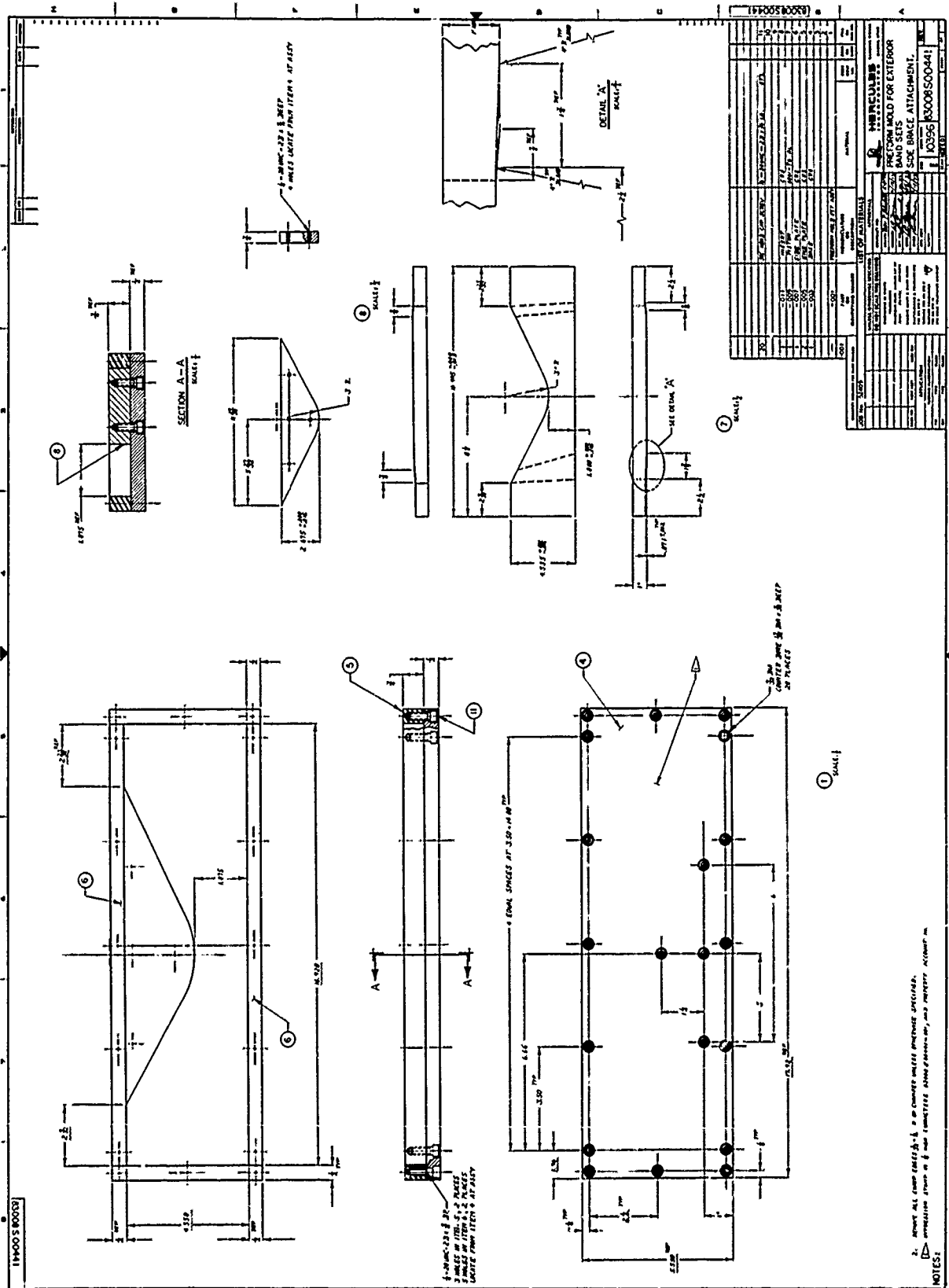
Figure 31. Exterior Band Set Mold, Side Brace Attachment, Drawing 83008S00441
