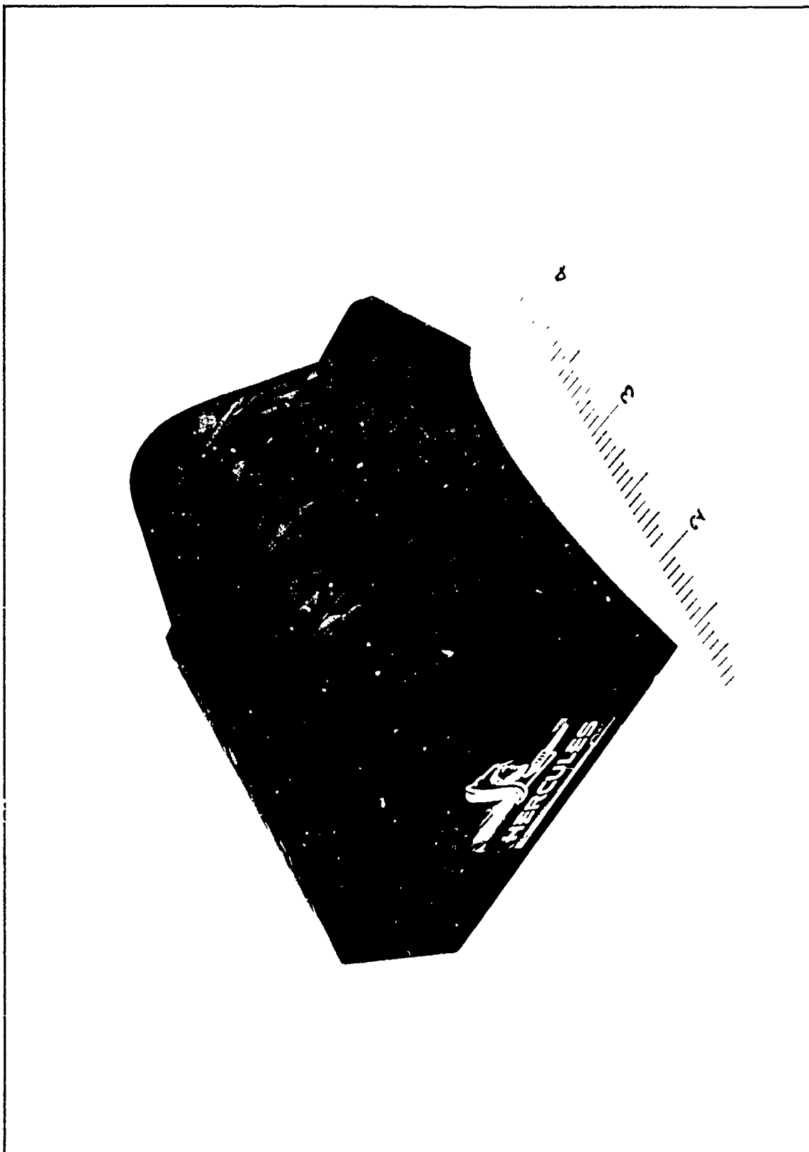
Figure 19. Torque Arm Attachment Spacer Block made from Random Chopped Graphite Composite
