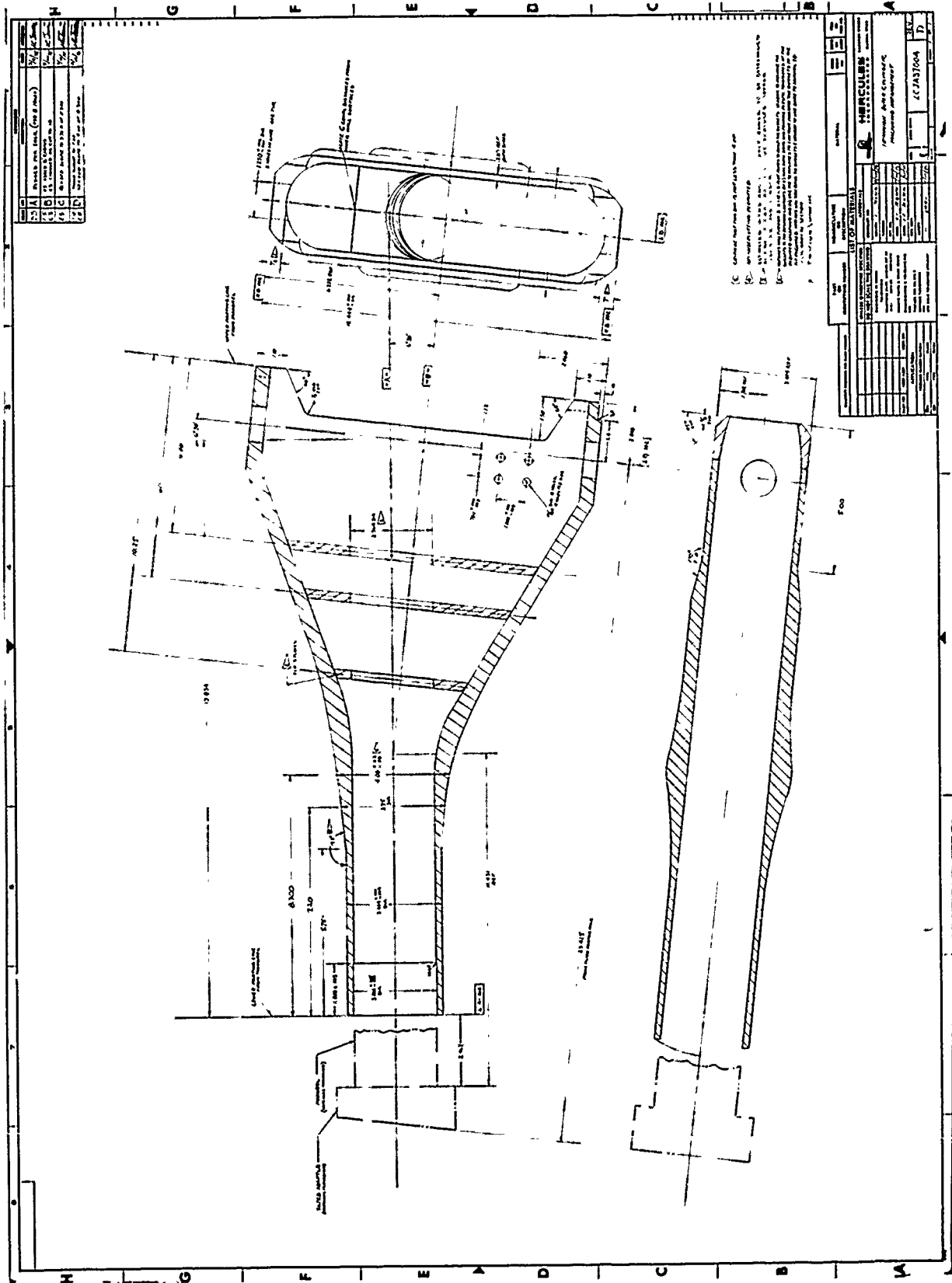
Figure 12. Third Design of A37B Graphite Composite Outer Cylinder/Trunnion
