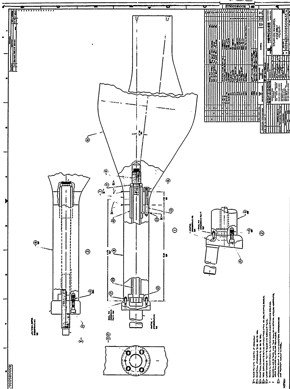
Figure 37. Second Trunnion Mandrel Assembly (Drawing 83008S00633) (Sheet 1 of 2)
