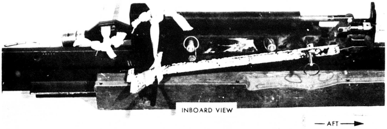
Figure 3. 35K Force Transfer Device (Actuator Only Shown).
