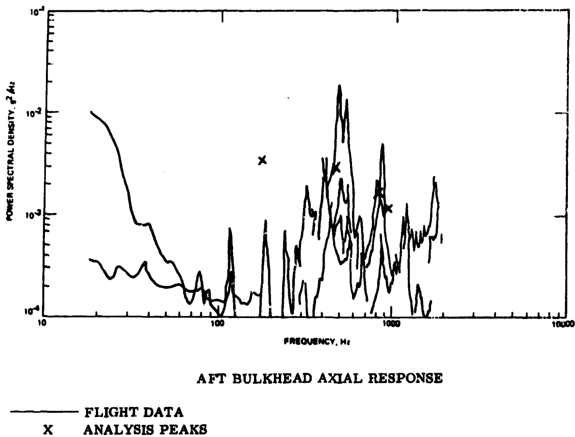
FIGURE A-3. COMPARISON OF ANALYSIS WITH BALLISTIC RE-ENTRY FLIGHT DATA (TBL)
