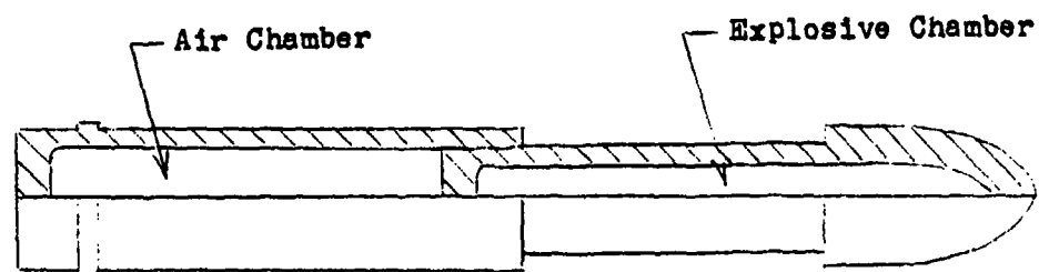
Before Firing (Half Section)
