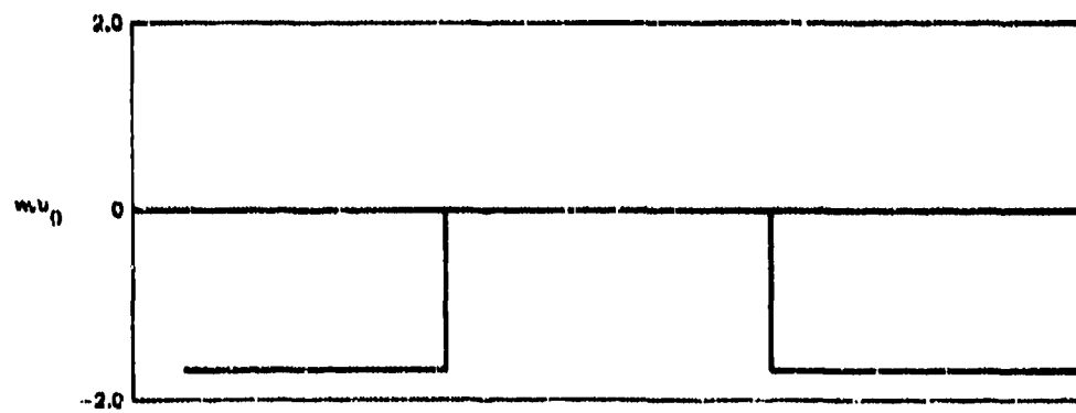
FIGURE 23. Perturbation Velocity on Circle \gamma' .
