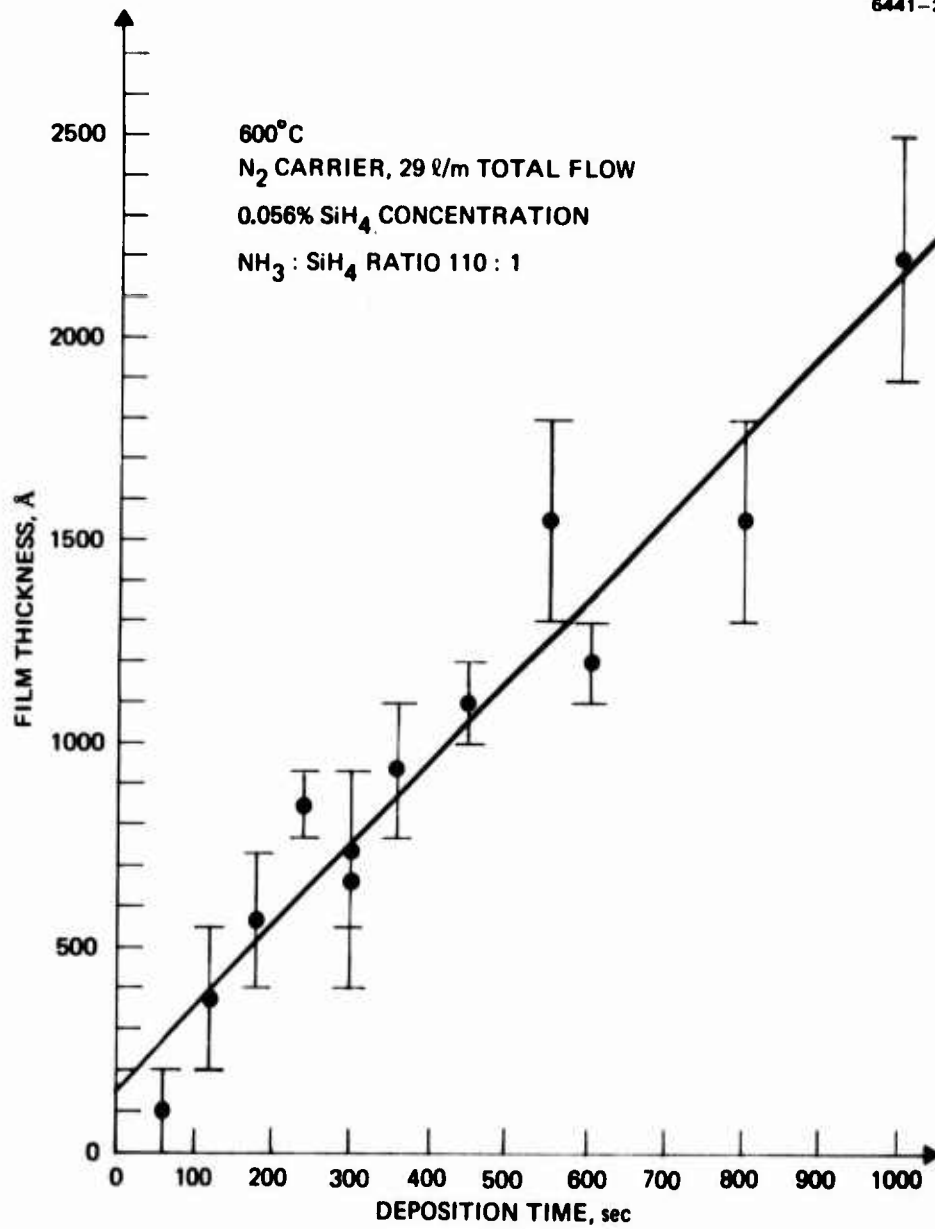
Figure 3. Film thickness as a function of deposition time for 600°C pyrolytic Si 3 N 4 ; N 2 carrier, 29 liters/min total flow, 0.056% SiH 4 concentration, NH 3 :SiH 4 ratio 110:1.
