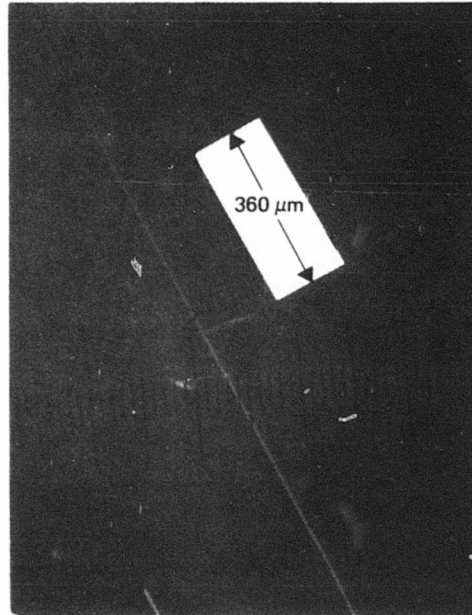
NOMARSKI PHOTOMICROGRAPH 75X, 22.42 \mu\text{m} /SMALL DIVISION
