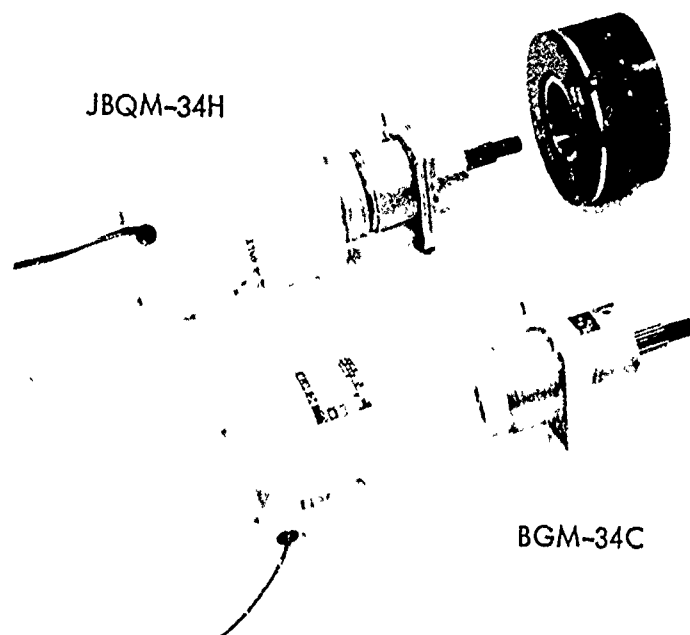
Figure 4-6. Electromechanical Actuator
