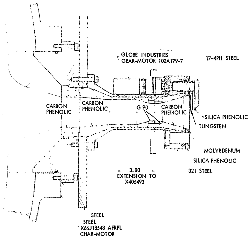
Figure 3-3. Char Motor TVC System for High Aluminum Content Propellant Tests
