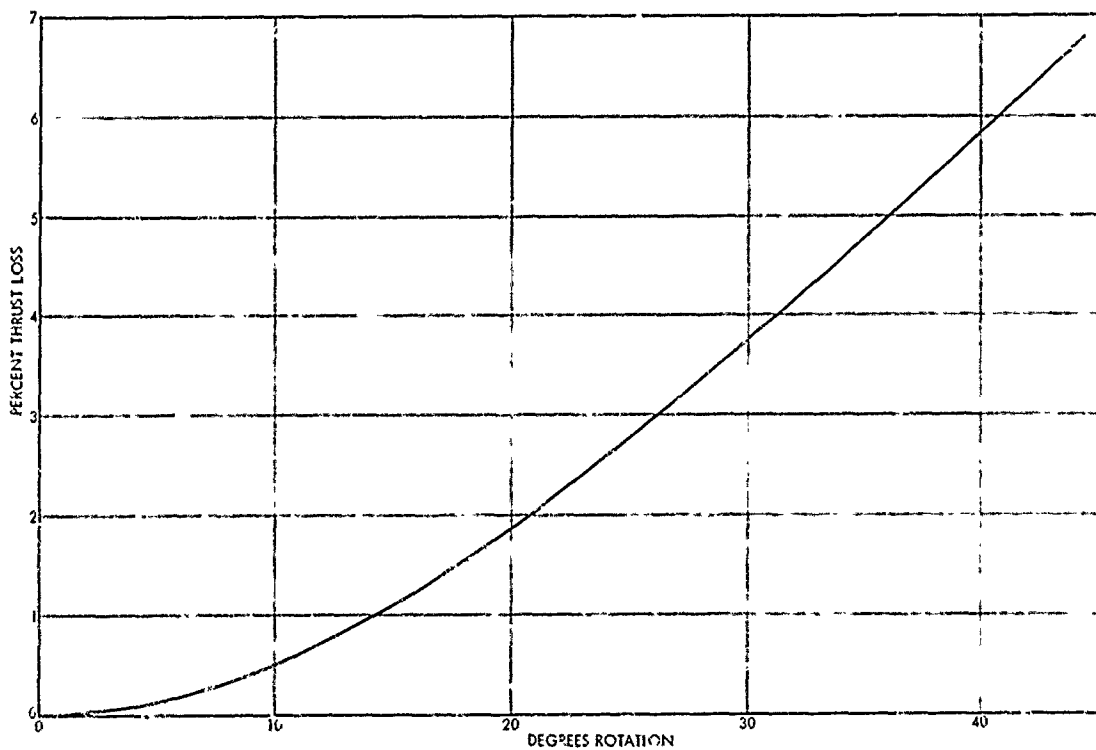
Figure 7-4. Thrust Loss as a Function of Shaft Rotation
