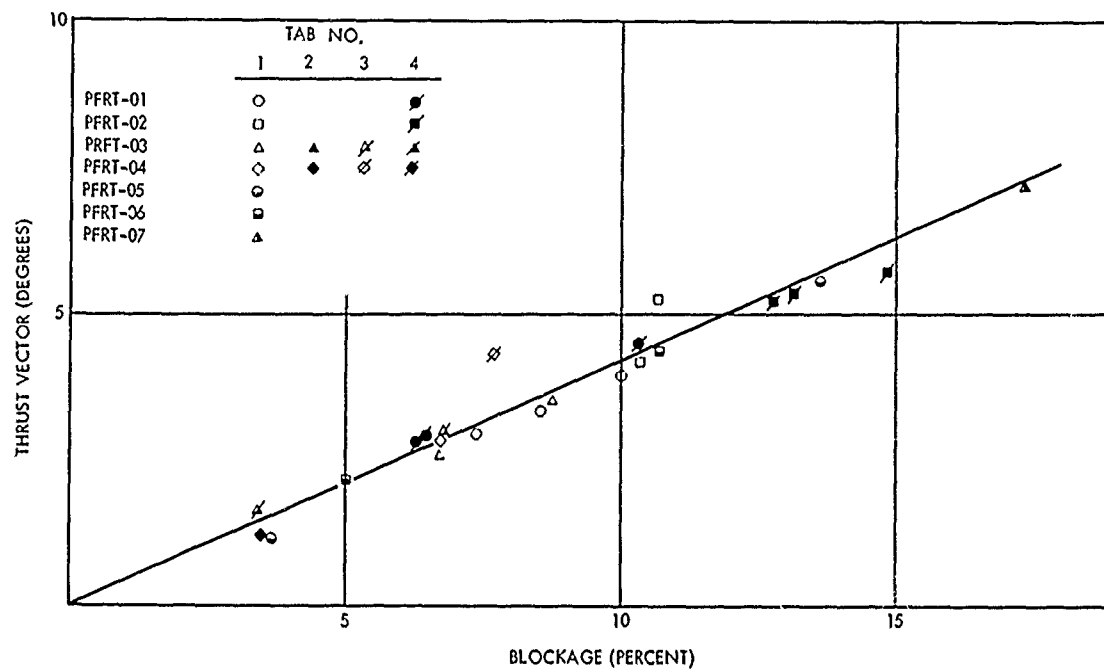
Figure 7-1. Thrust Vector Angle vs. Nozzle Exit Area Blockage
