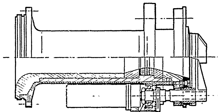
Figure 3-5. Flightweight Quickturn Test Nozzle
