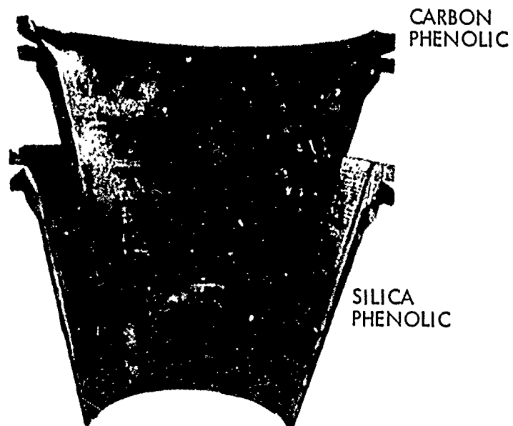
Figure 5-20. Nozzle Exit Liner Erosion Comparison
