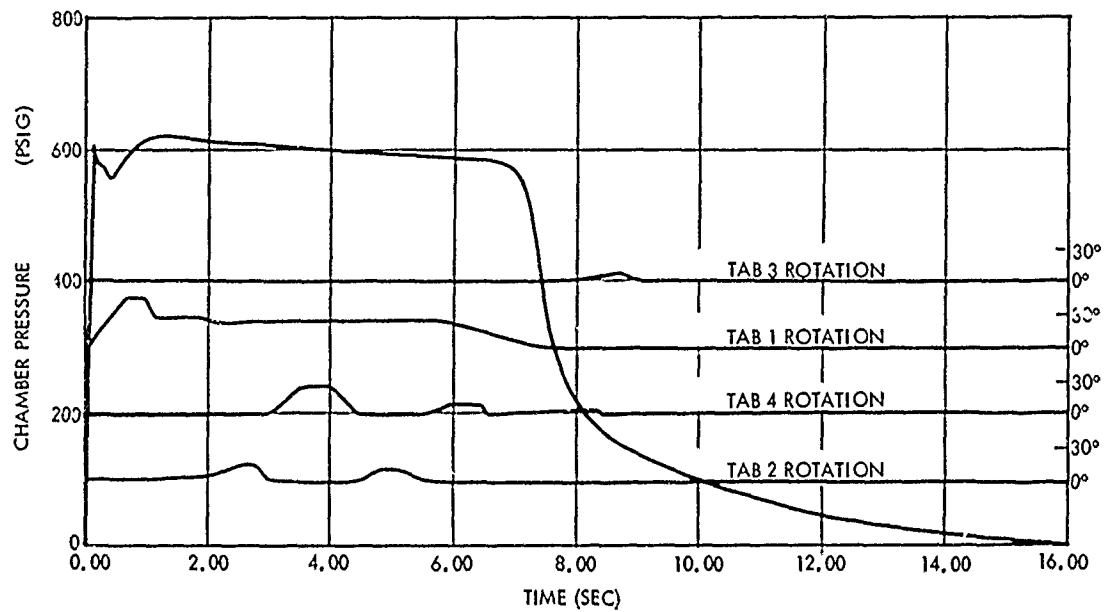
Figure 5-32. Tab Actuation and Motor Chamber Pressure, PFRT-05
