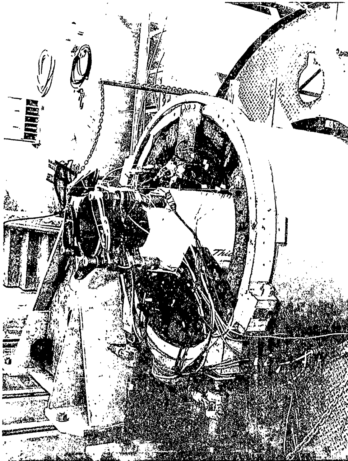
Figure 5-3. Test Unit PI-2 Installed on AFRPL Char Motor Stand
