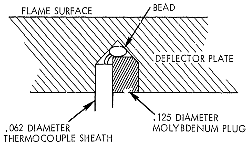
Figure 8-4. Buried Thermocouple
