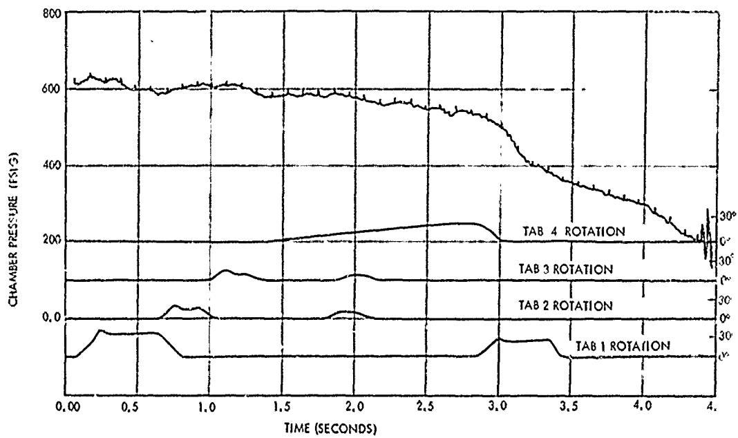
Figure 5-4. Motor Chamber Pressure and Tab Actuation, PI-1
