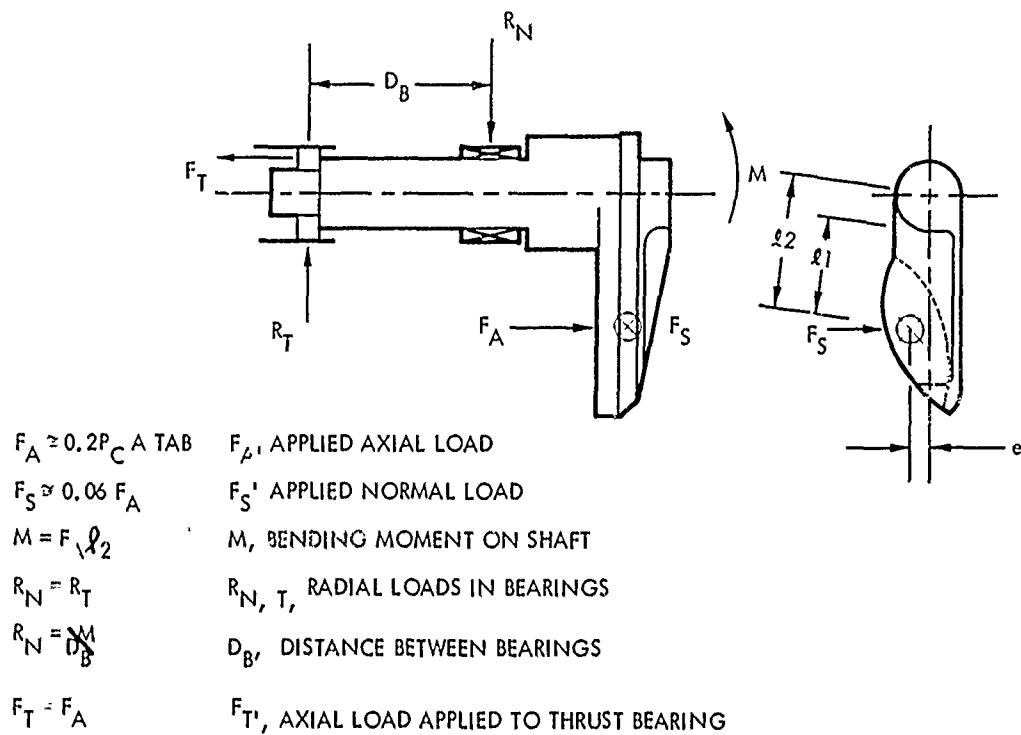
Figure 4-13. Free Body Force Diagram of the Tab Assembly
