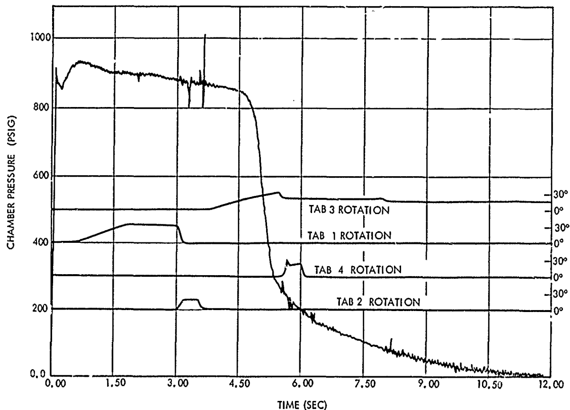
Figure 5-29 Tab Actuation and Motor Chamber Pressure PFRT-04
