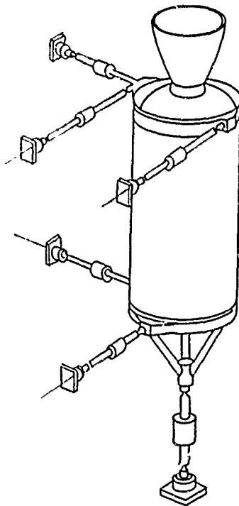
Figure 8-1. AFRPL Six-Component Char Motor Thrust Stand
