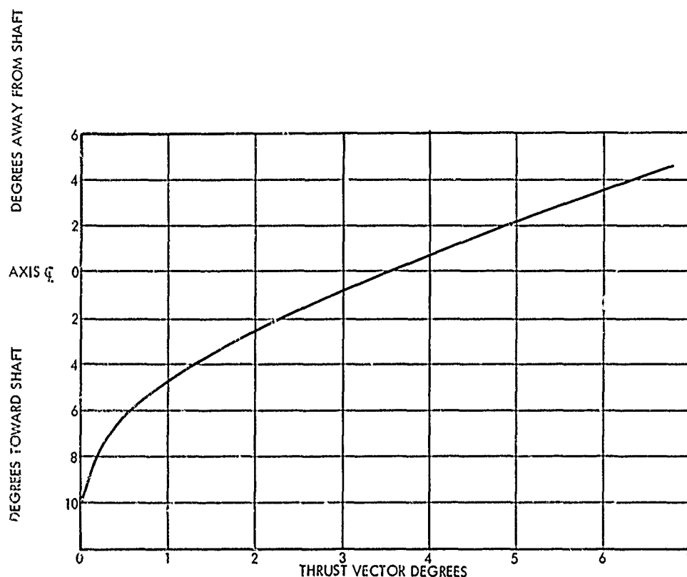
Figure 7-5. Thrust Vector Progression
