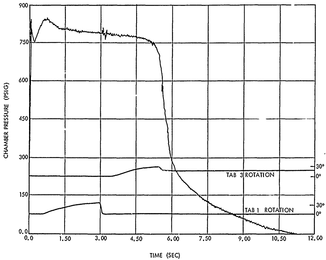
Figure 5-27. Tab Actuation and Motor Chamber Pressure, PFRT-03
