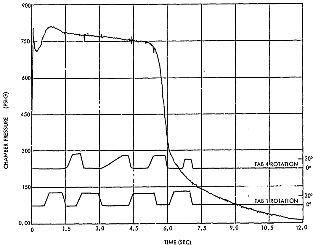
Figure 5-18. Tab Actuation and Motor Chamber Pressure, PFRT-01
