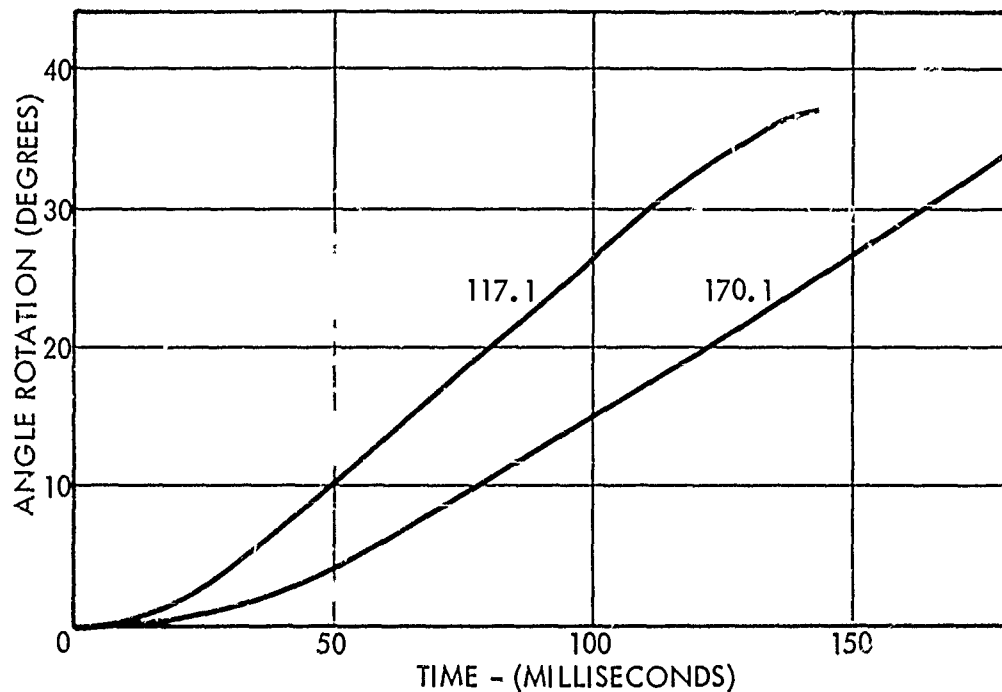
Figure 7-6. Actuation Responses
