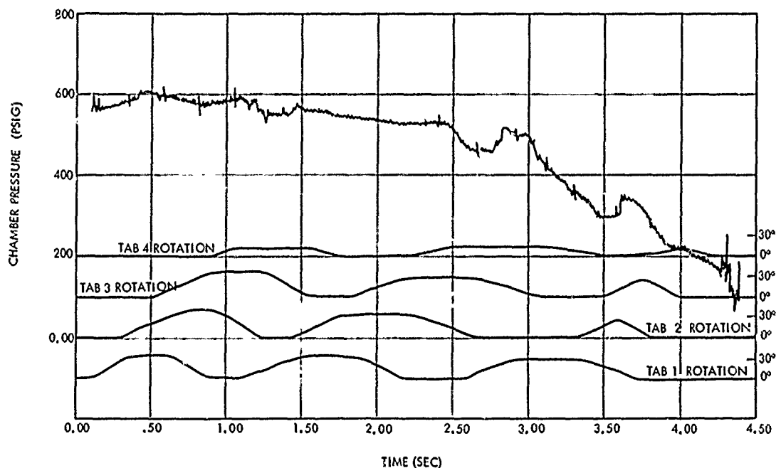
Figure 5-6. Motor Chamber Pressure and Tab Actuation, PI-2
