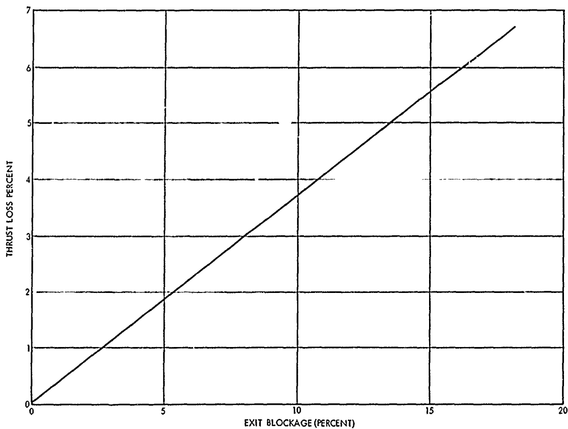
Figure 7-2. Thrust Loss as a Function of Nozzle Exit Area Blockage
