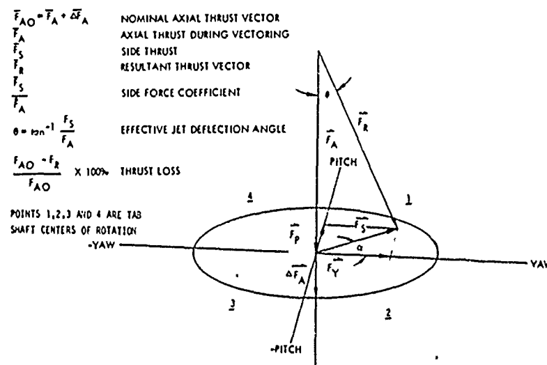
Figure 3.1. Force Relationships Used to Characterize the Performance of Jet Tab Thrust Vector Control
