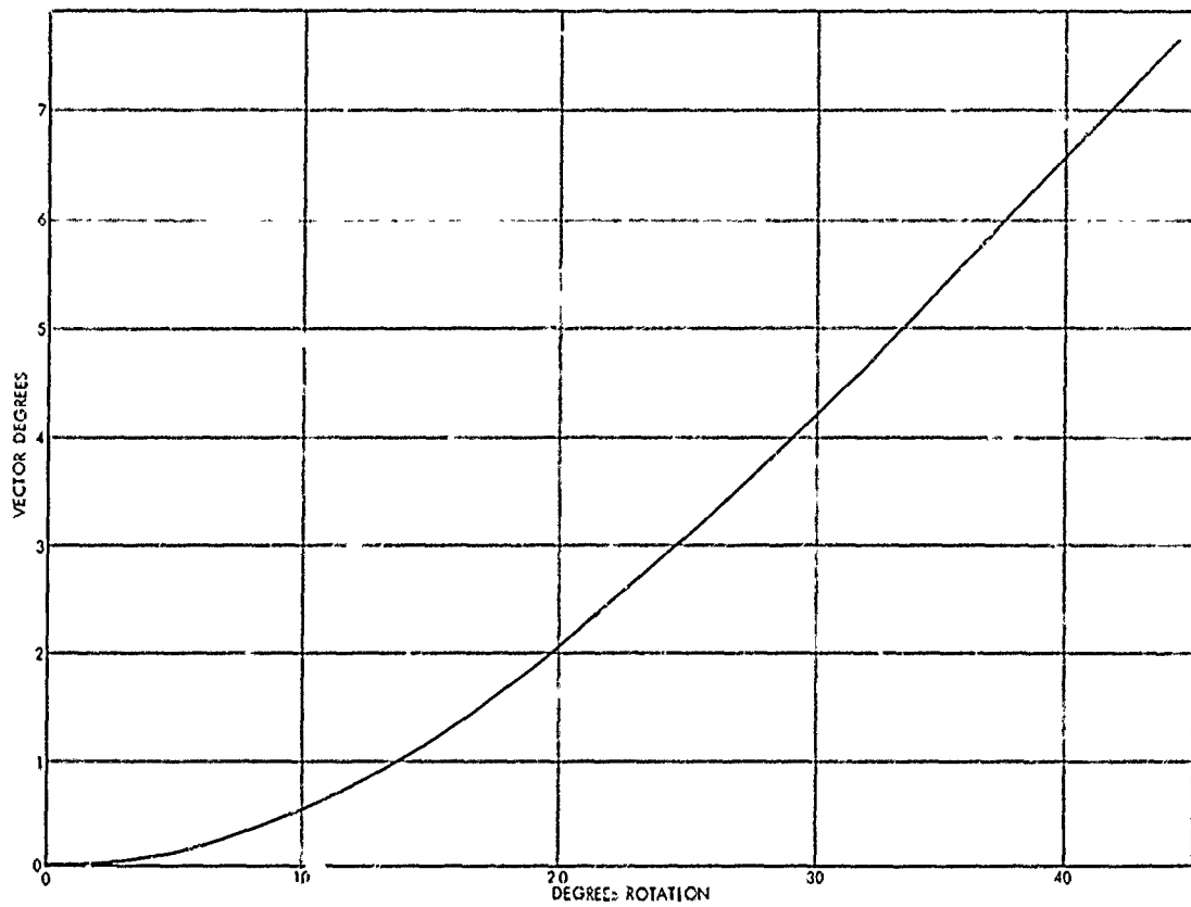
Figure 7-3. Thrust Vector vs. Shaft Rotation
