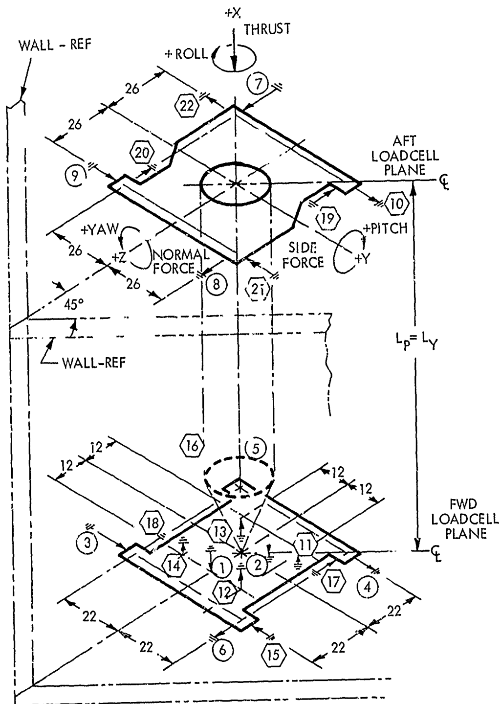
Figure 8-2. Test Stand Schematic
