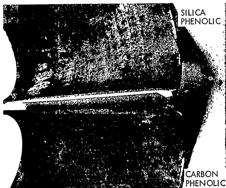
Figure 5-9. Nozzle Liner Erosion Comparison
