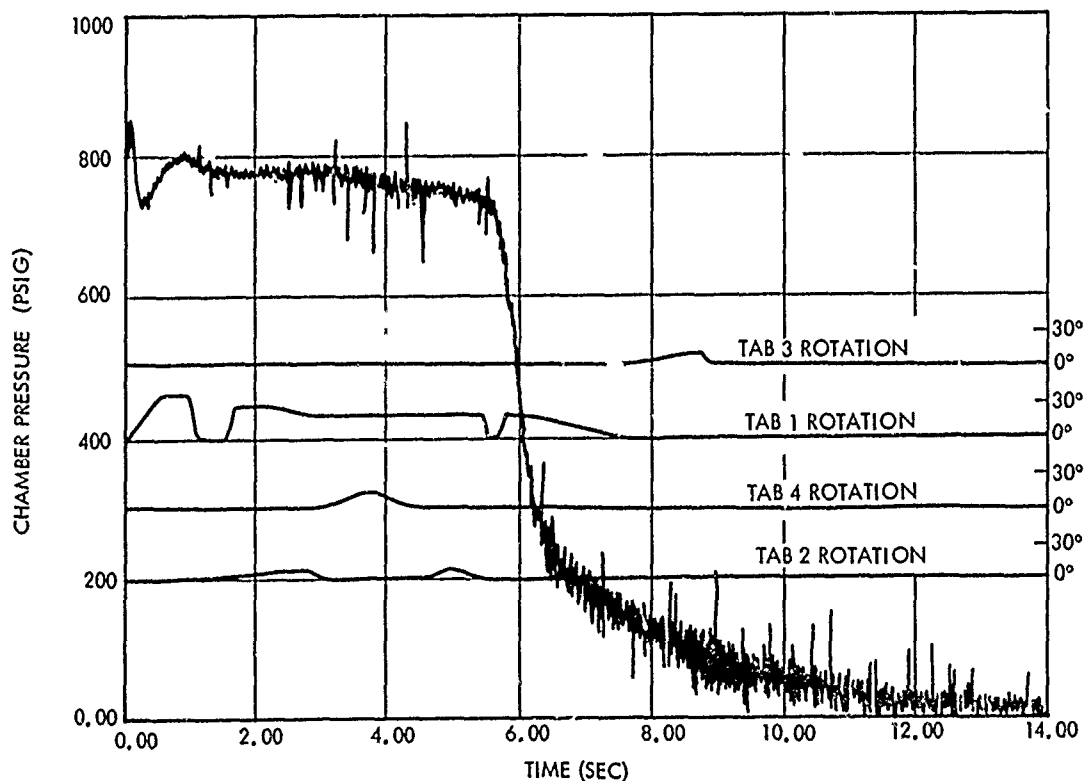
Figure 5-34. Tab Actuation and Motor Chamber Pressure, PFRT-06
