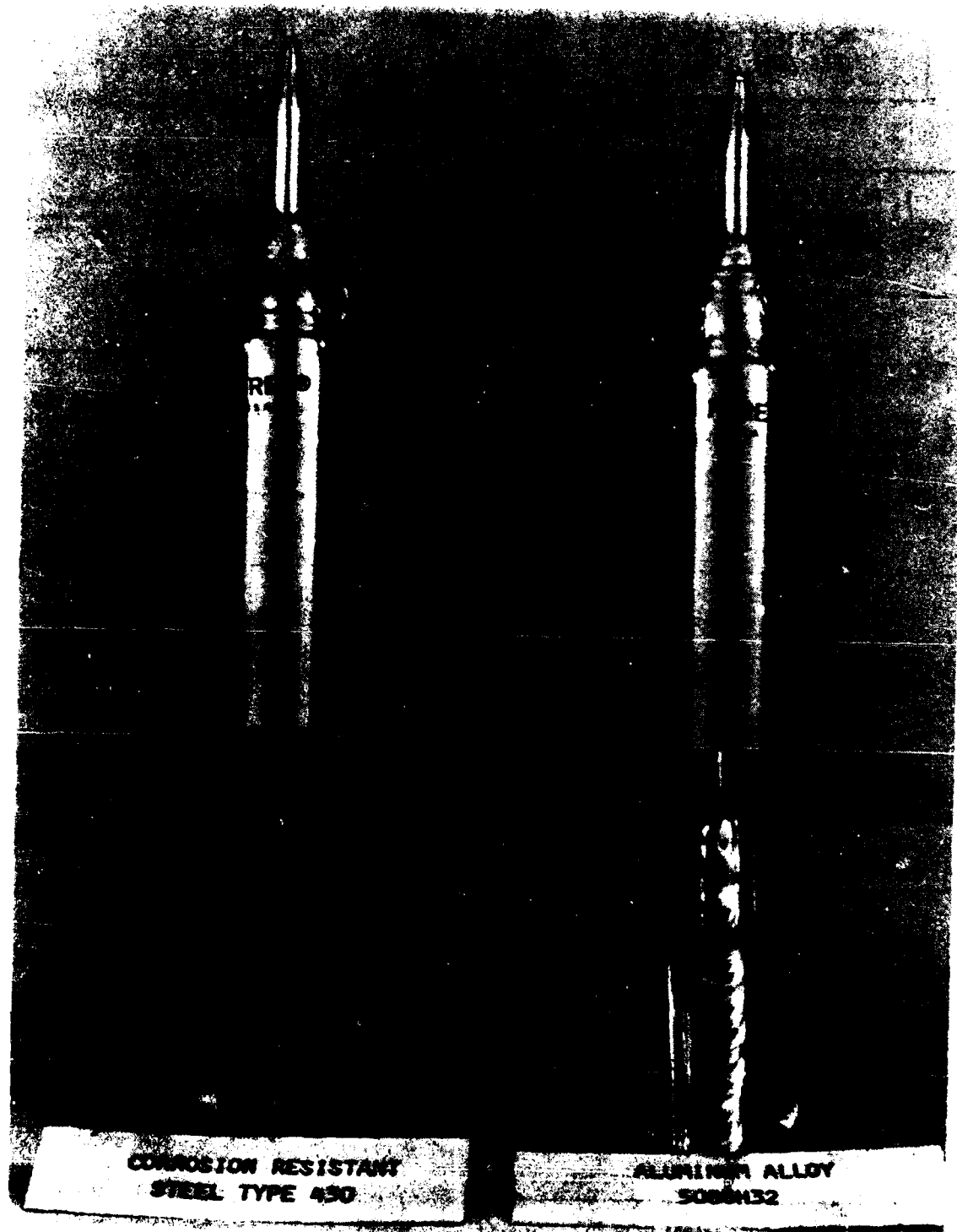
Figure 3. Test Specimen/Capsule
