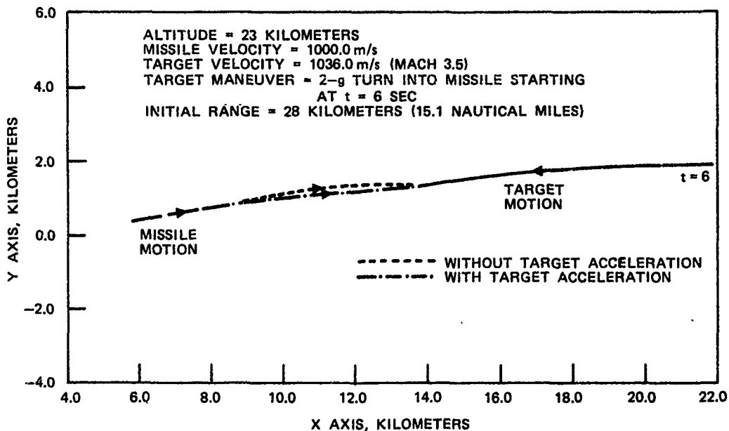
FIGURE 10. Missile and Target Trajectories in the Horizontal Plane for Example 2.
