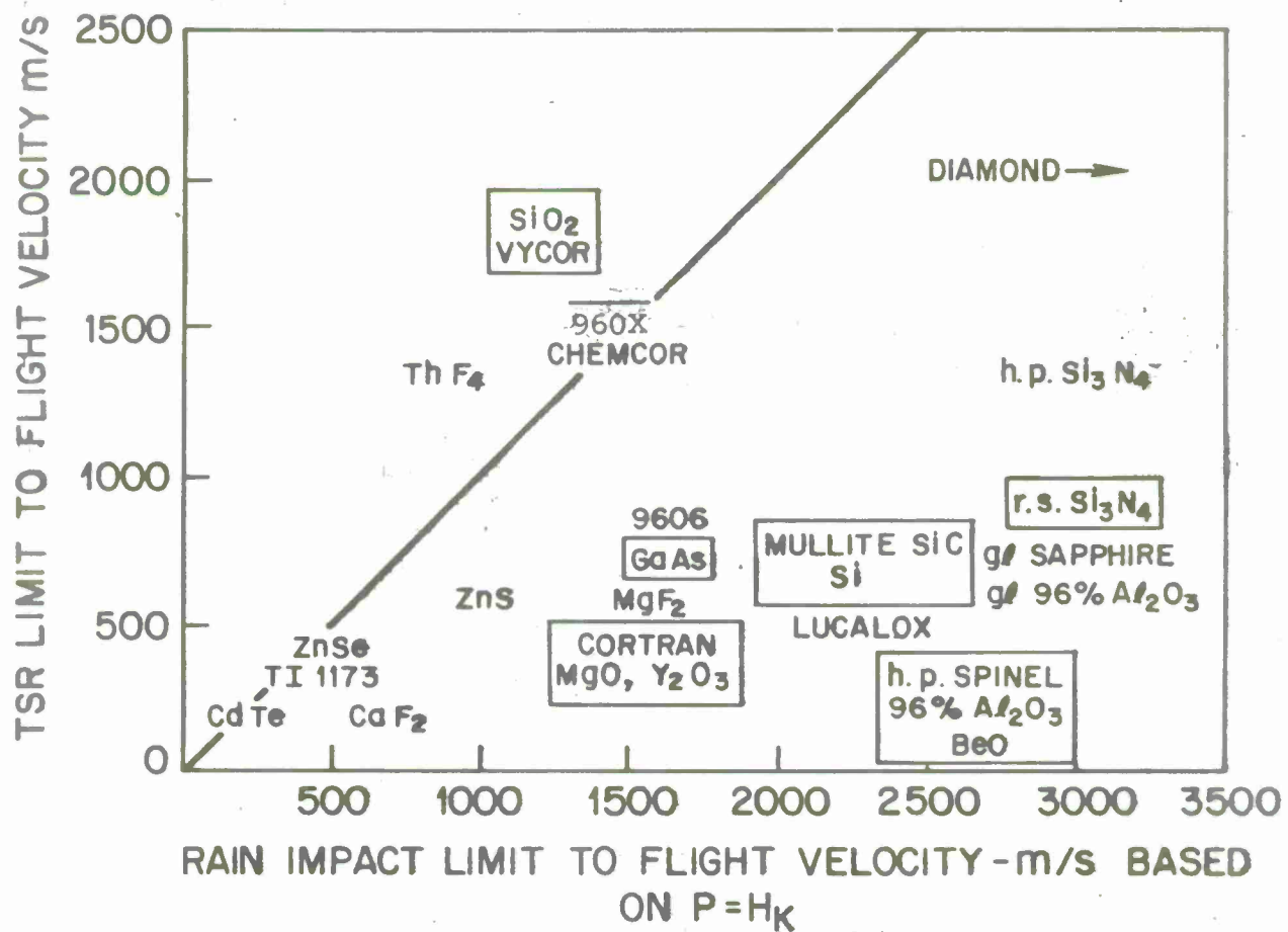
FIGURE VI. 4. Comparison of the Thermal Shock Limit to Flight Velocity to the Rain Impact Limit. The Boxed-in Values Fail Along the 1/(24 \times 3) Slope in Figure VI.2.
