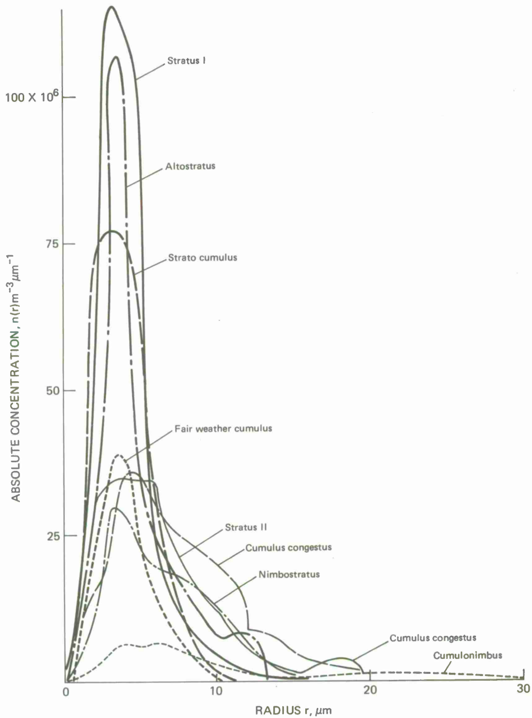
FIGURE III.1. Drop Size Distribution in Clouds.
