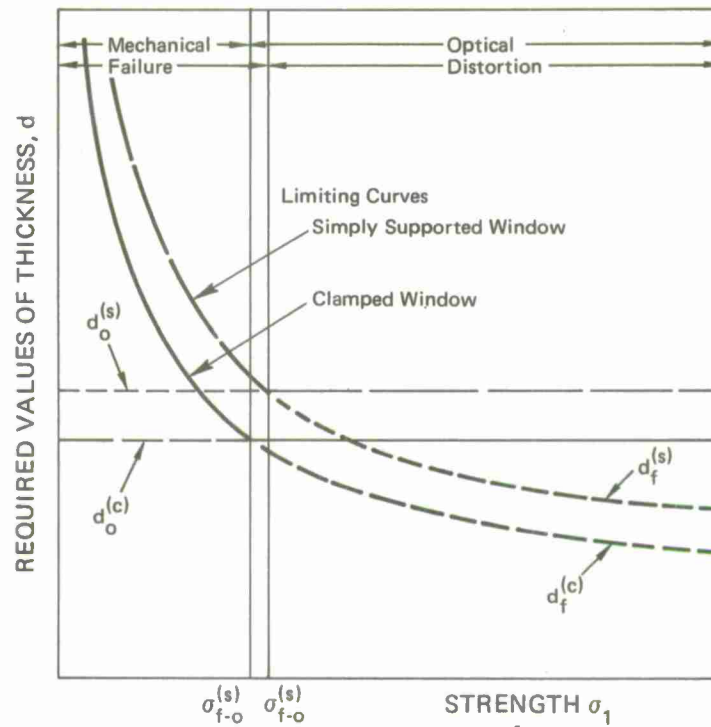
FIGURE III.6. Schematic Illustration of the Value of Window Thickness d required to Withstand Pressure p . The Minimum Value of d is the Larger of d^{(c)} and d^{(s)} (or d_o^{(s)} and d_f^{(s)} ), as Illustrated by the Heavy Lines in the Figure.
