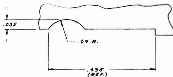
CRIMP GROOVE DETAIL SCALE: 10-1
