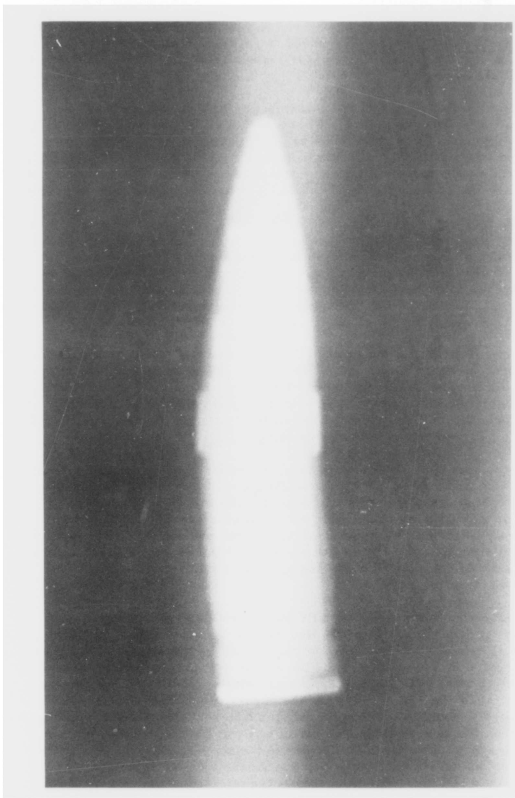
Figure 8. Flash X-Ray of I20876-128 Series Projectile at -65^{\circ}\text{F} and 3300 Ft/Sec
