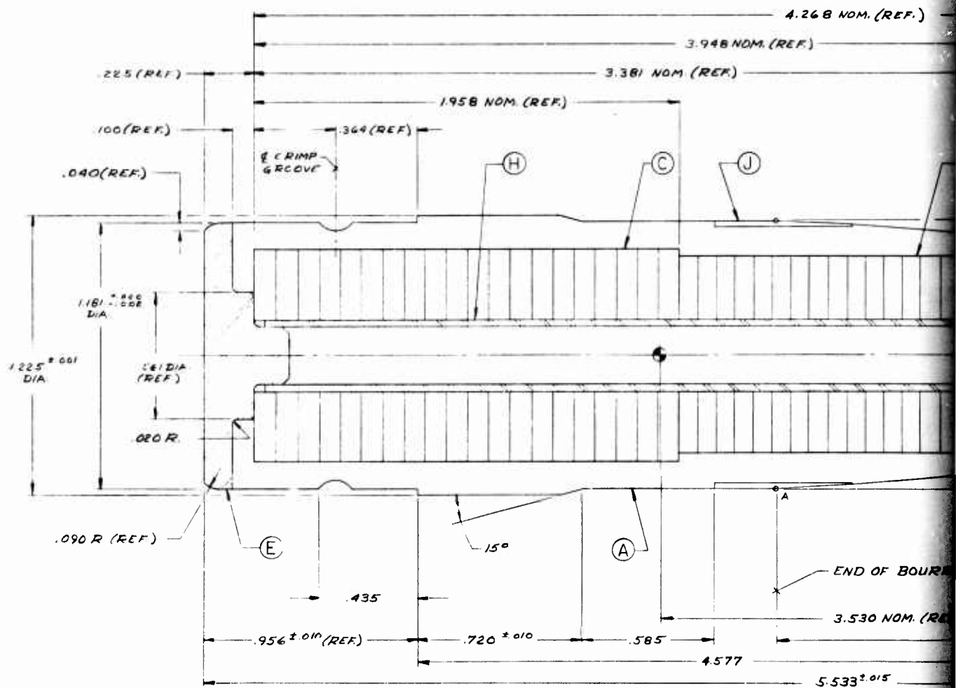
CRIMP GROOVE DETAIL SCALE: 10-1
