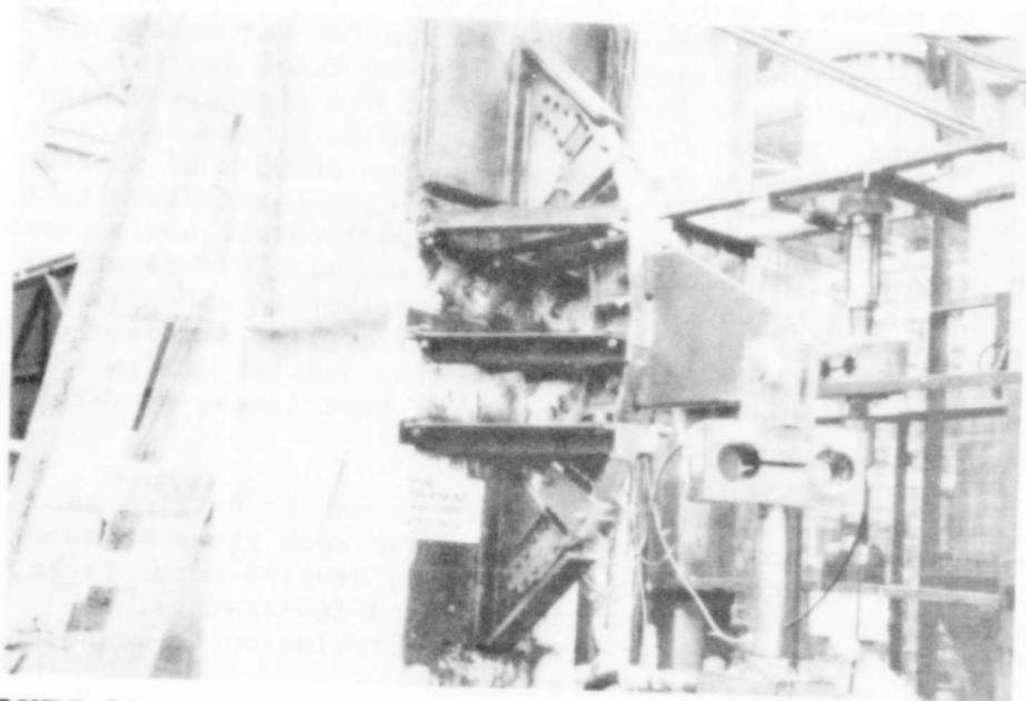
FIGURE 30 YF-16 TITANIUM FRAME IN FATIGUE TEST FIXTURE
