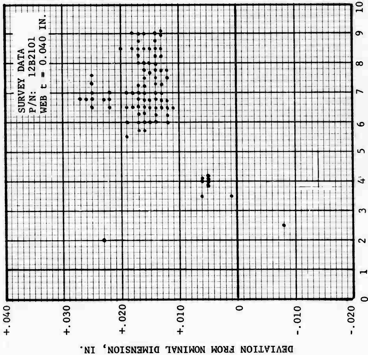
FIGURE 6 WEB DIMENSIONAL DEVIATIONS FOR EXCESSIVE STIFFENER SPACING
