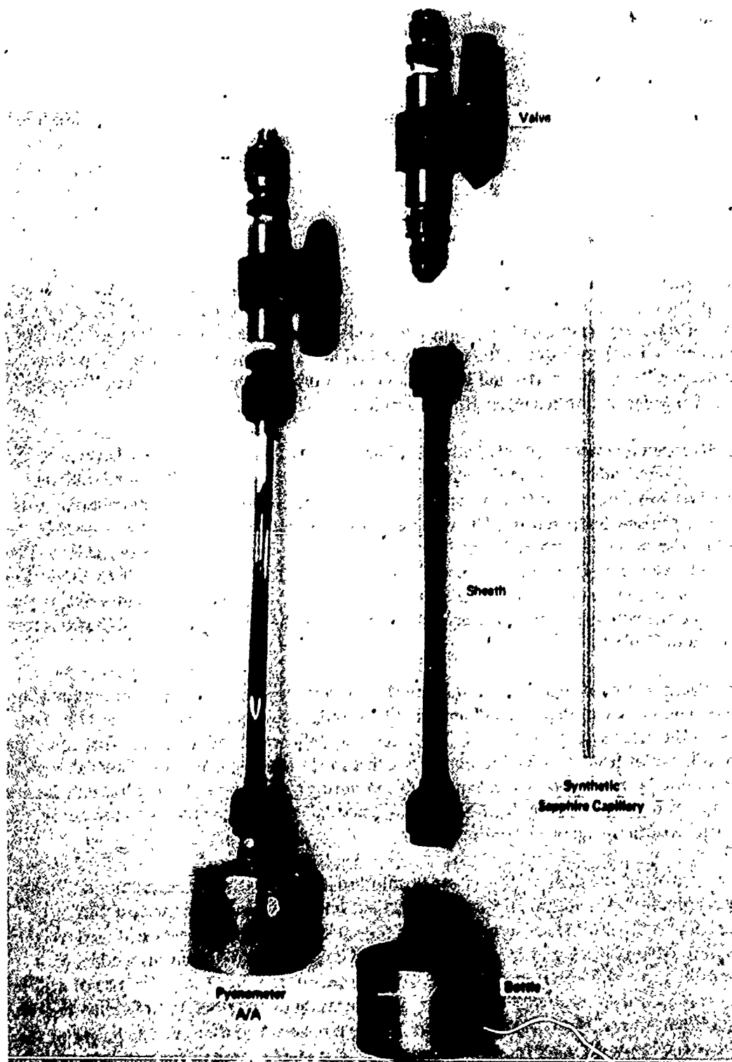
Figure 1. Pycnometers
