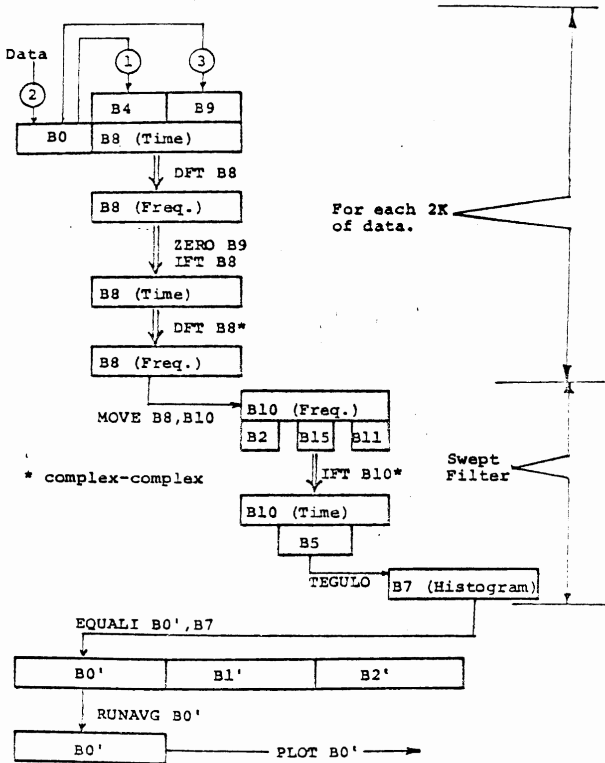
Figure 3 Data Flow For HISCAN
