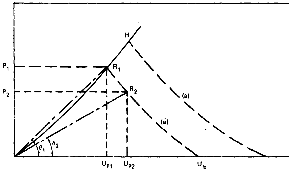
Fig. 3. Projectile velocity.
