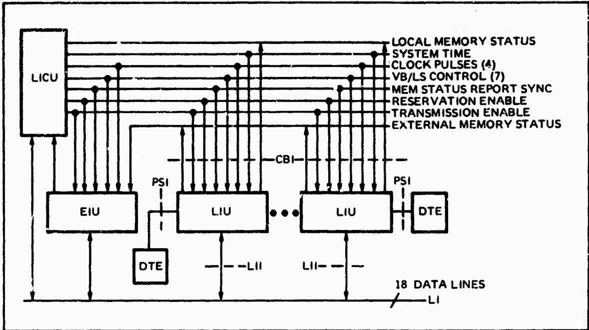
Figure 4.6.A.3-1. Control Bus Interface. The bus structure of the interfaces minimize LIU, EIU, and LICU hardware.
