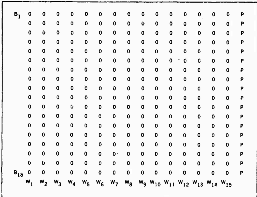
Figure 4.9.2-1. Header Parity Implementation
