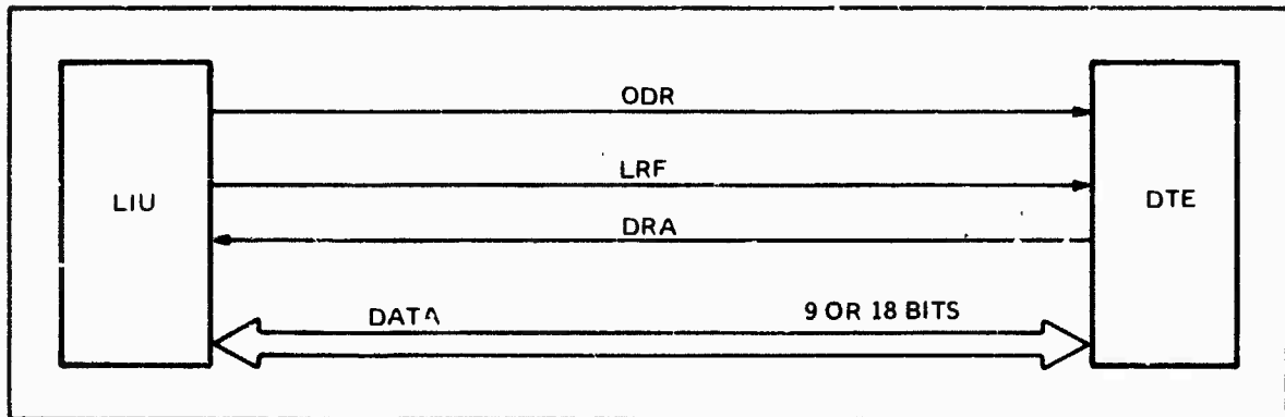
Figure 4.5.6-1. LIU Output to DTE: Applicable Signal Lines. Three of the four unidirectional PSI control lines are applicable to message transfer from LIU to DTE.
