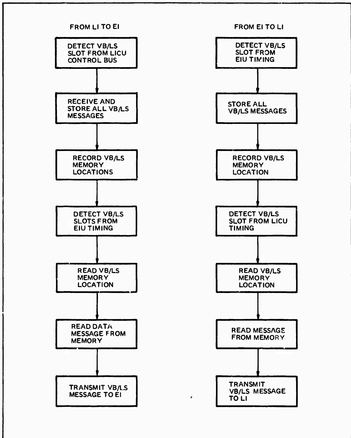
Figure 4.7.9-1. VB/LS Message Transfer. The EIU transfers VB and LS messages between the Local and External Intraconnects and maintains their sequential order by sensing Sequence Numbers in their headers.
