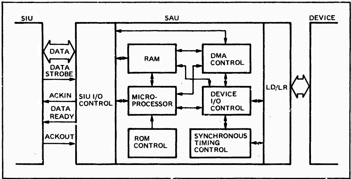
Figure 3.5-1. Device SAU Functions. The basic functional configuration of all SAUs is similar with some identical components and some device peculiar components.
