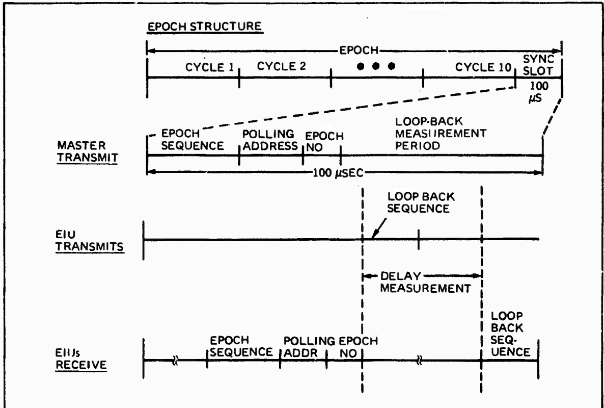
Figure 4.4.6-1. Epoch Structure for External Timing Acquisition. An epoch timing acquisition technique is used to measure propagation delay times.
