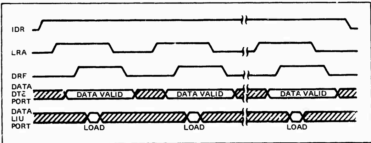
Figure 4.5.5.3. LIU Input From DTE (FSI): Timing. All message segment transfers are identical, whether the transfer is the first one, the middle one, or the last one. Transfer events are not a function of rise times or of pulsed signals.
