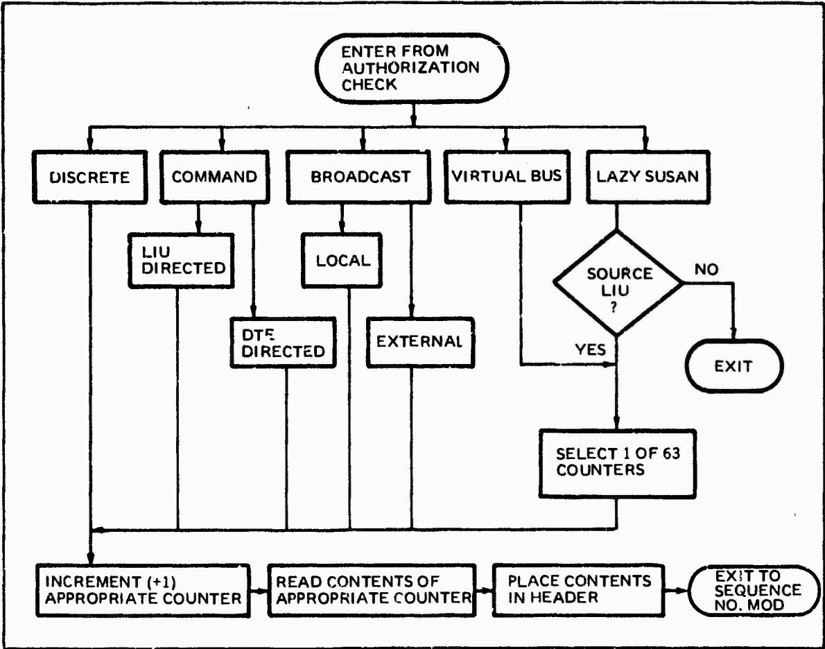
Figure 4.6.B.8-1. Message Number Modifications
