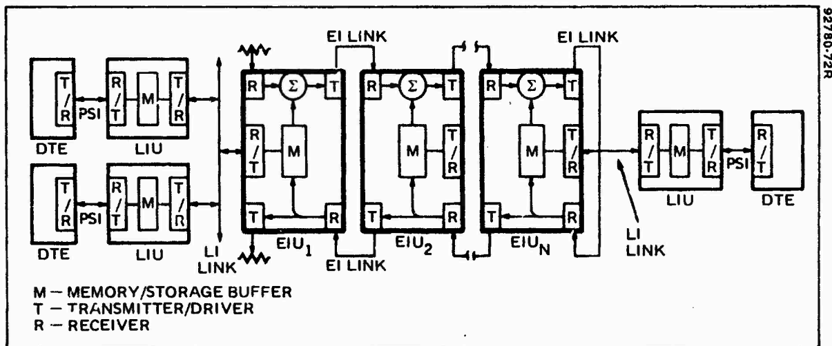
Figure 4.9.1-1. Modular C 3 Transmission Diagram. The intrashelter configuration consists of LIUs on one LI link only. The intershelter configuration uses the EIUs and EI links as well.
