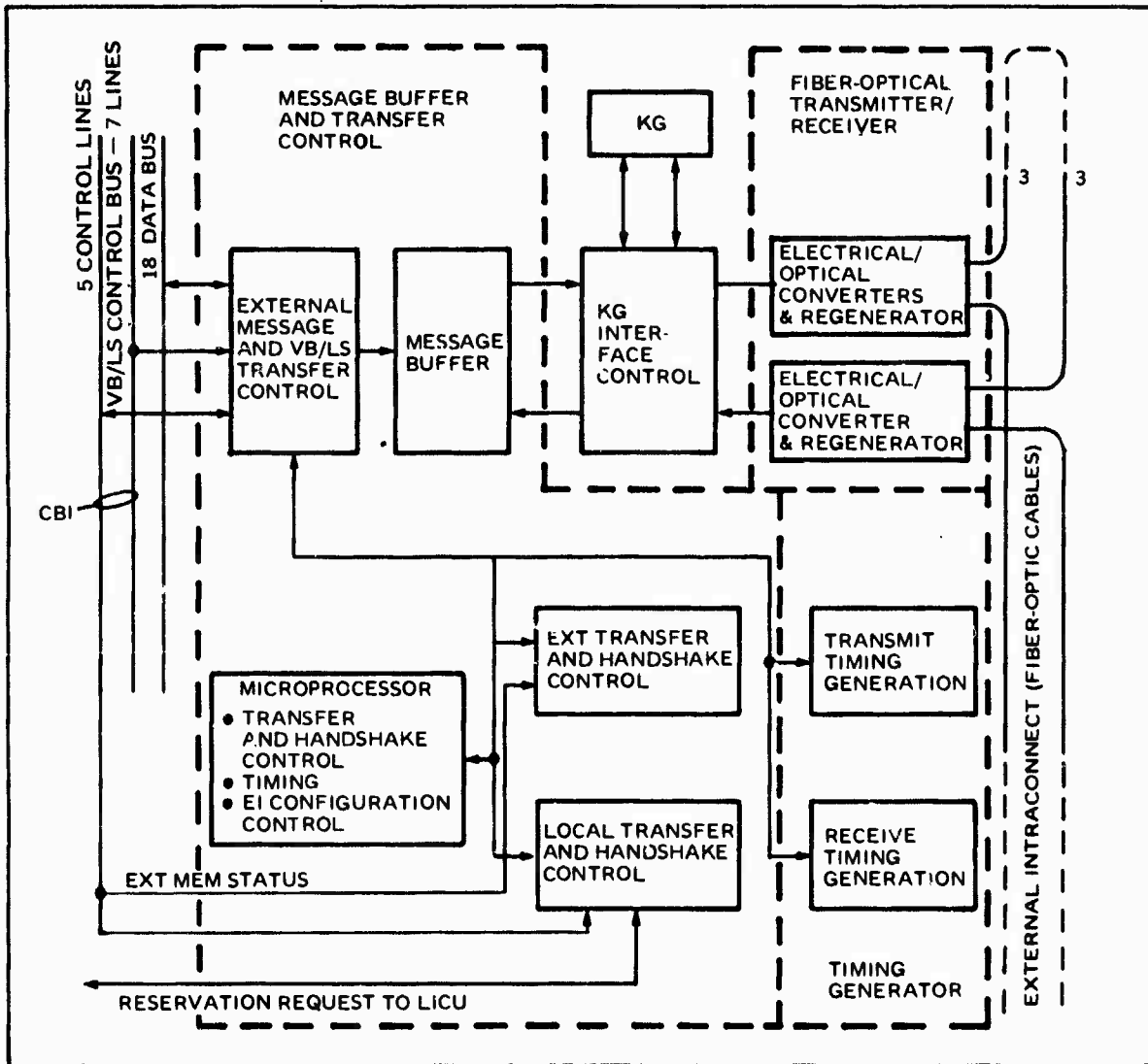
Figure 4.7.1-1. The EIU Functional Block Diagram. The functions are performed by discrete ICs or by a microprocessor, depending on the processing speed required.
