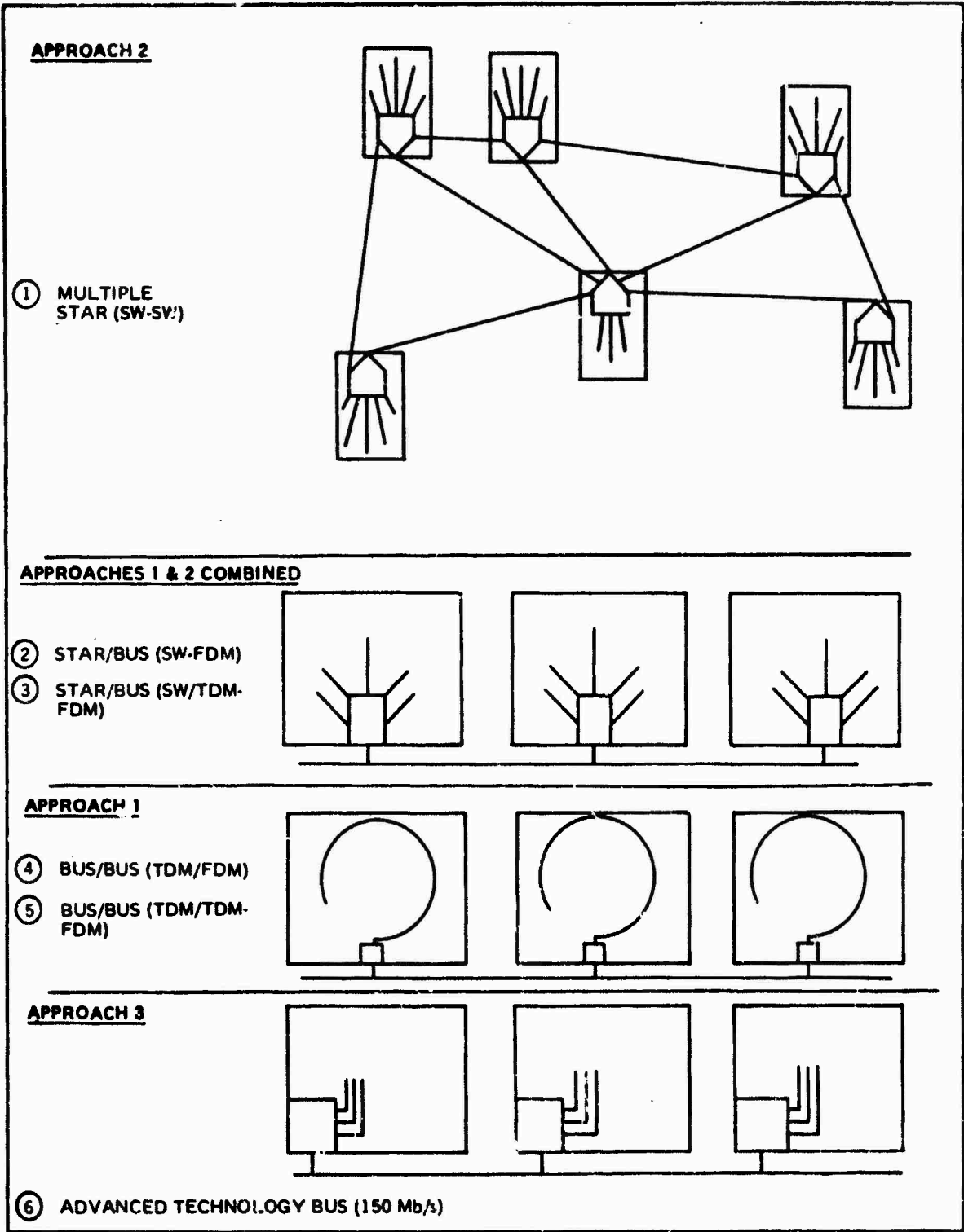
Figure 2.4-2. Candidate Flexible Intraconnect Architectures. Six candidates were developed from three basic approaches.
