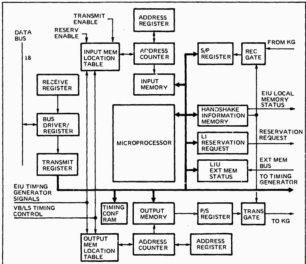
Figure 4.7.2-1. EIU Message Buffer and Transfer Control Block Diagram. Implementation exploits integrated circuits and a microprocessor to satisfy speed and flexibility requirements and to minimize hardware.
