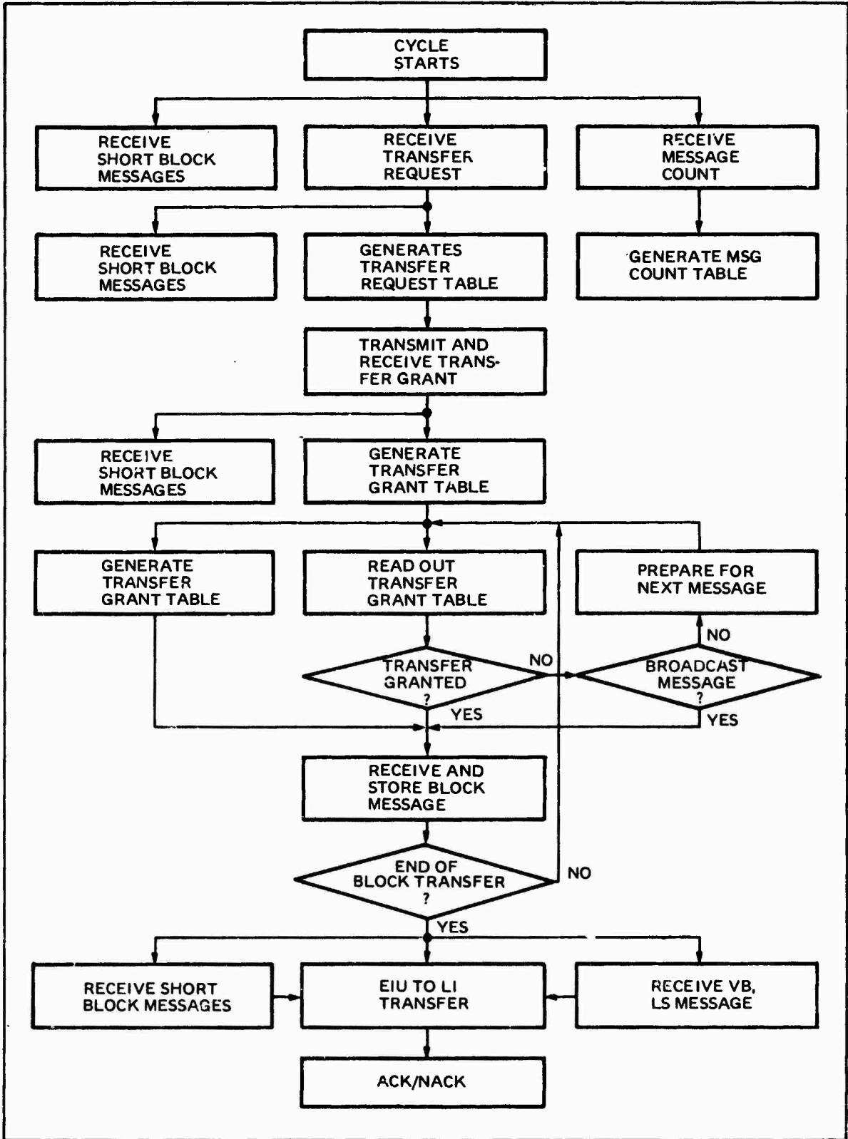
Figure 4.7.7-1. Block Message Reception From EI
