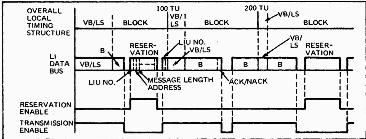
Figure 4.4.2-1. Timing of Local Data Bus and Transfer Control Bus. Using the data bus for message and reservation transfers, and a separate bus for control provides efficient data transfers as well as positive and flexible control of data flow.
