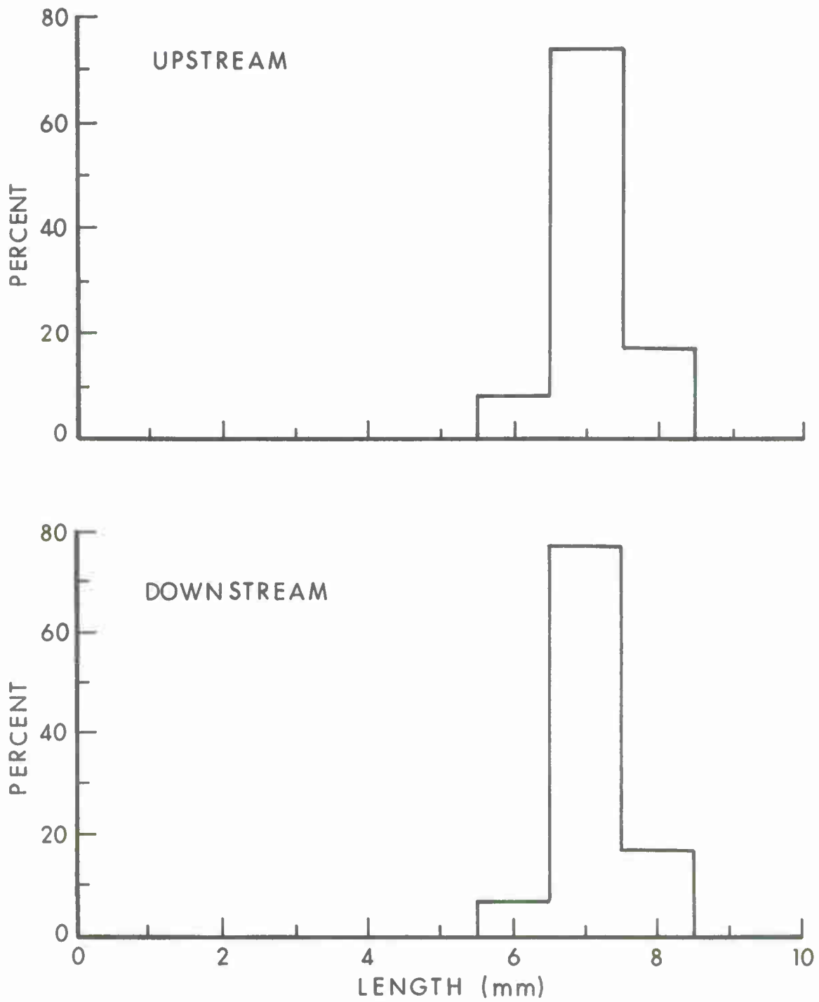
Figure 10. Typical Length Distributions for Air Conditioner Filter Tests
