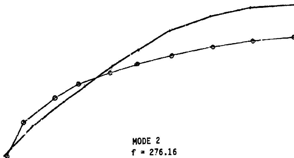
Figure 201. QSRA Fuselage Modal Plot
