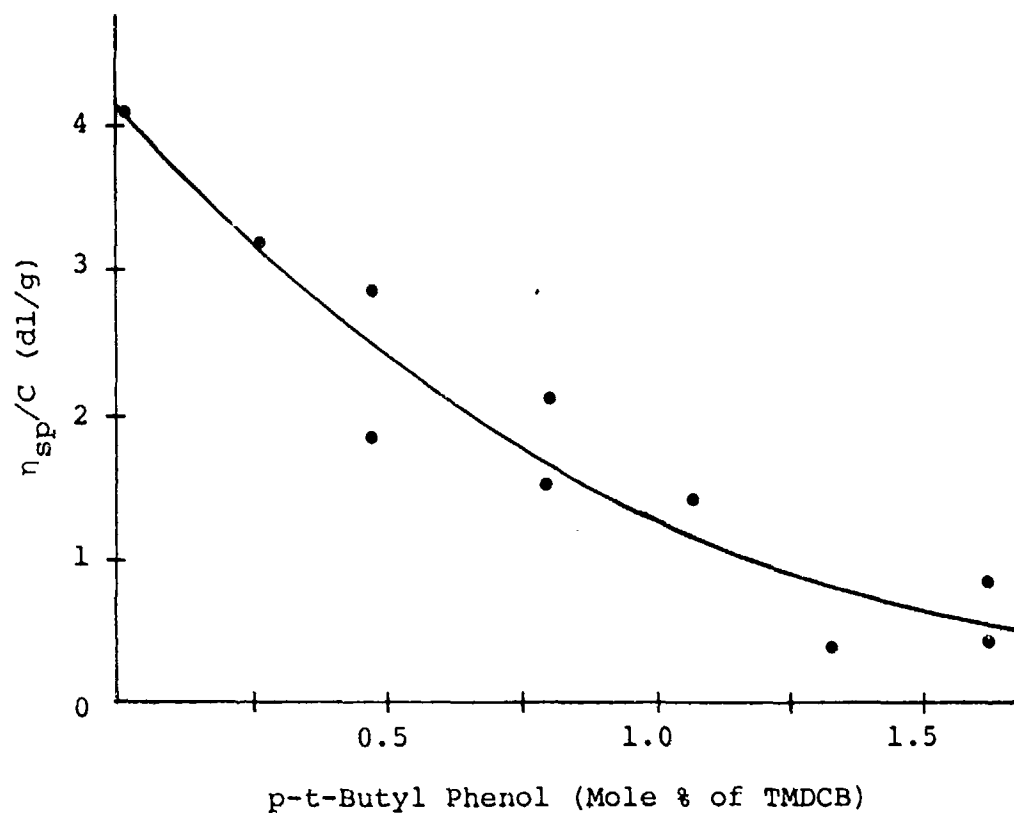
FIGURE 2. Variation of Polymer Reduced Specific Viscosity with Amount of Regulator for AF-TP-2 Prepared by Two-Stage Interfacial Process
