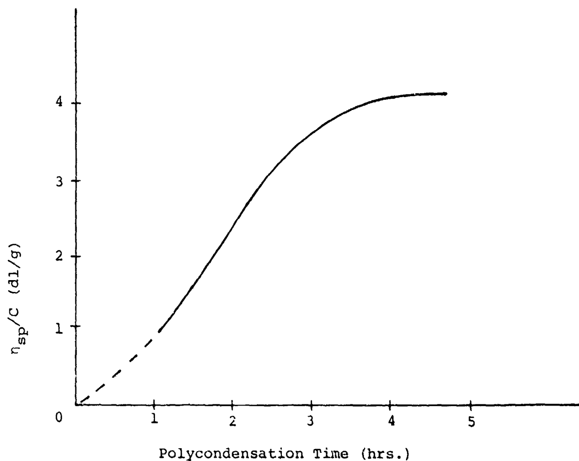
FIGURE 1. Variation of Reduced Specific Viscosity with Polycondensation Time for AF-TP-2 Preparations without Regulator
