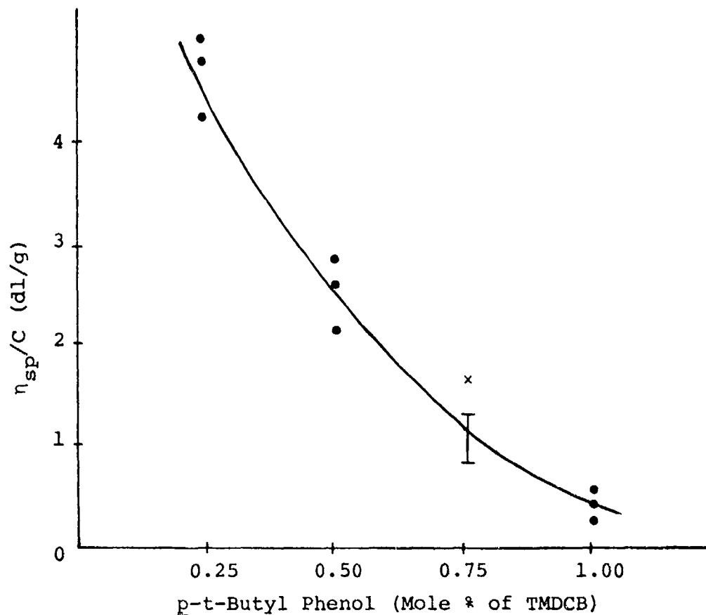
FIGURE 3. Variation of Polymer Reduced Specific Viscosity with Amount of Regulator for AF-TP-2 Prepared by Combination Solution-Interfacial Process
