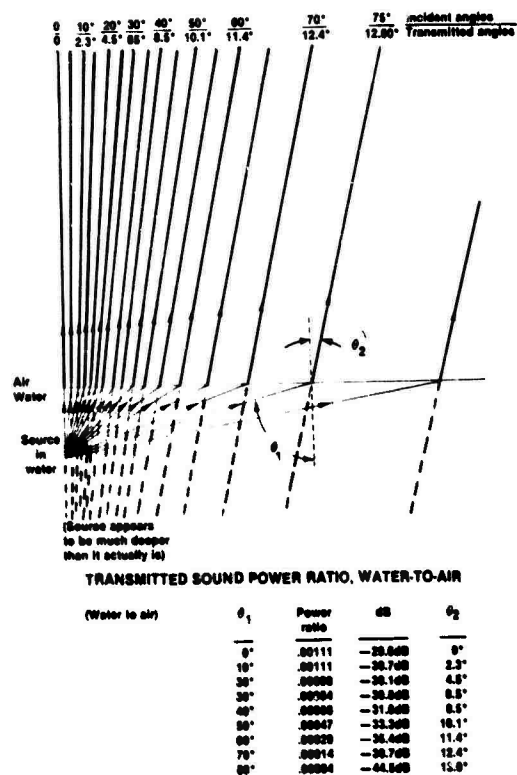
Figure 3.44b. Water-to-Air
