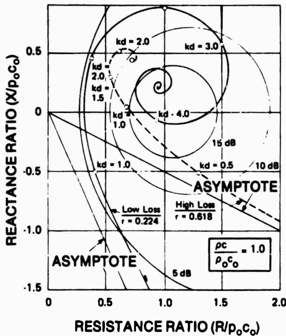
Figure 5.23. Impedance Spirals for Two Loss Parameters
