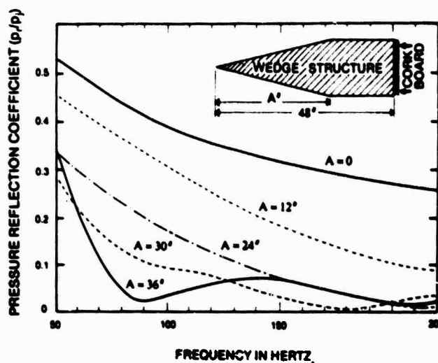
Figure 5.27. Gradual Transition Matching
