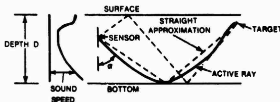
Figure 1.46. Range Finding using Arrival Angles or Time Delays
