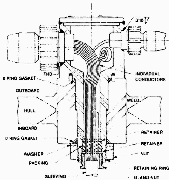
Figure 5.12. Hull Penetrator
