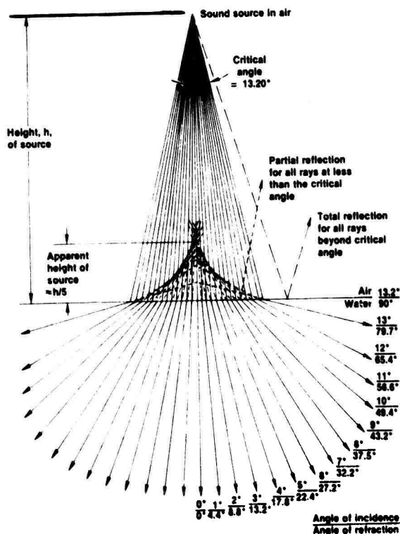
Figure 3.44a. Air-to-Water
