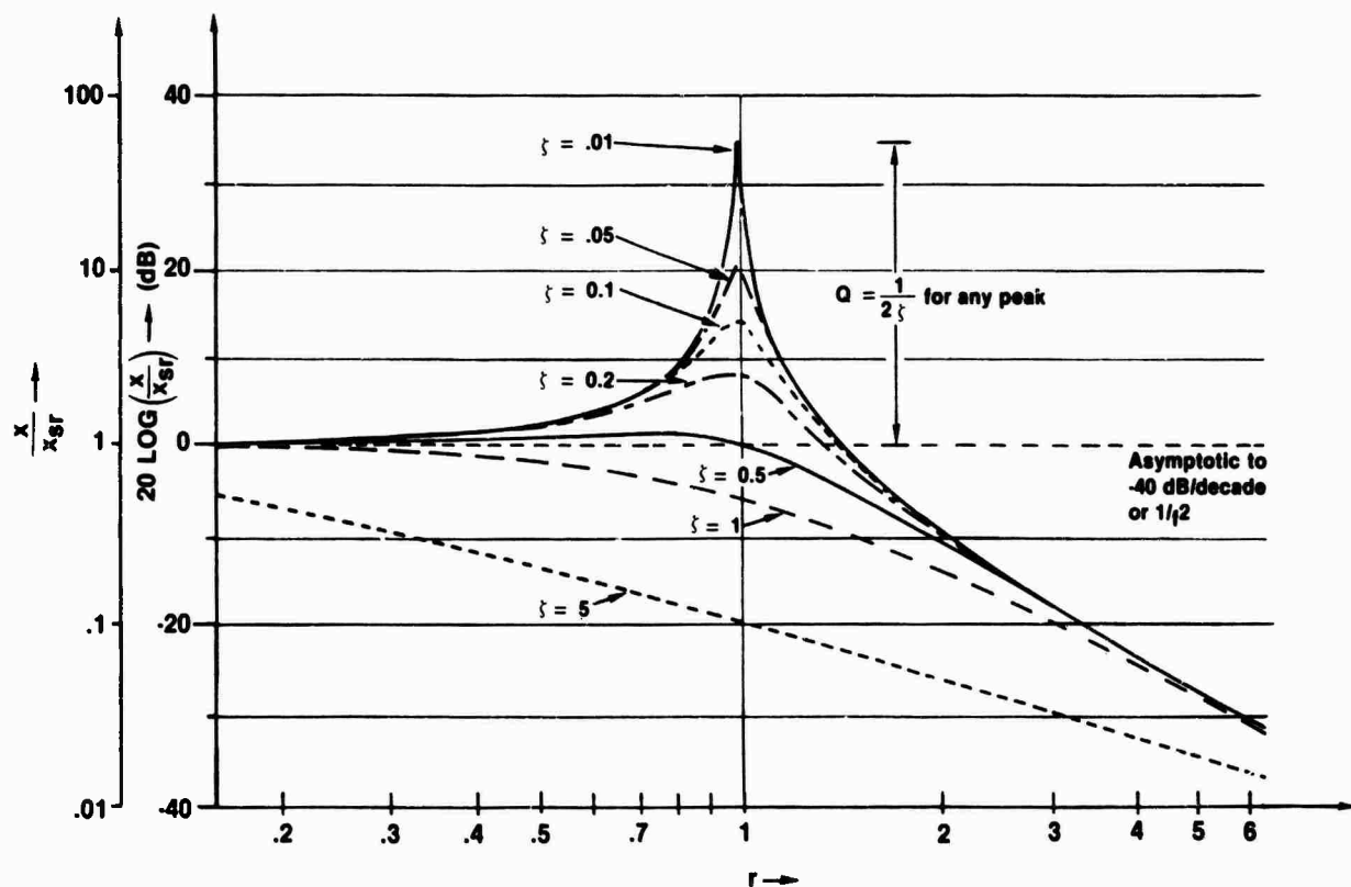
Figure 3.8. Displacement Response of Driven Mass
