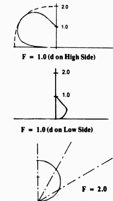
Figure 3.53. Hydrophone Response Patterns for Various Standoff Distances as Function of Incidence Angle
