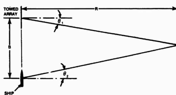
Figure 1.45. Range Finding using Triangulation
