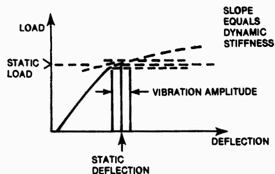
Figure 2.11. Belleville Spring Application
