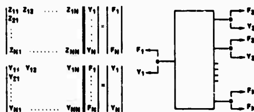
Figure 3.17c. N Port System
