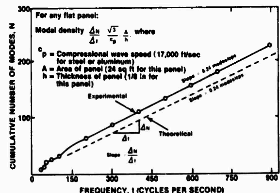
Figure 3.31. Modal Density
