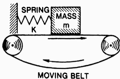
Figure 2.6. Chatter or Stick-Slip System
