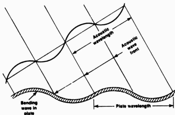
Figure 3.55. Coincidence Effect
