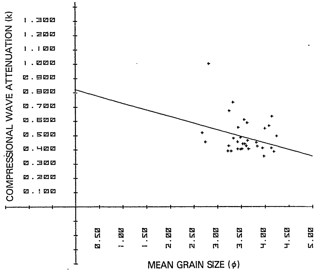
Figure 16B. Regression of sediment geoaoustic properties for fine sand sediments; attenuation with mean grain size.
