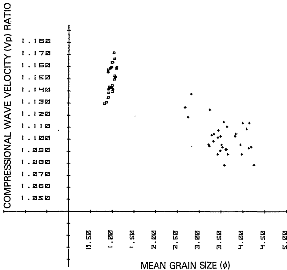
Figure 11C. Scatter plots of sediment geoaoustic properties for fine (+) and coarse (o) sand sediments; velocity ratio vs mean grain size.
