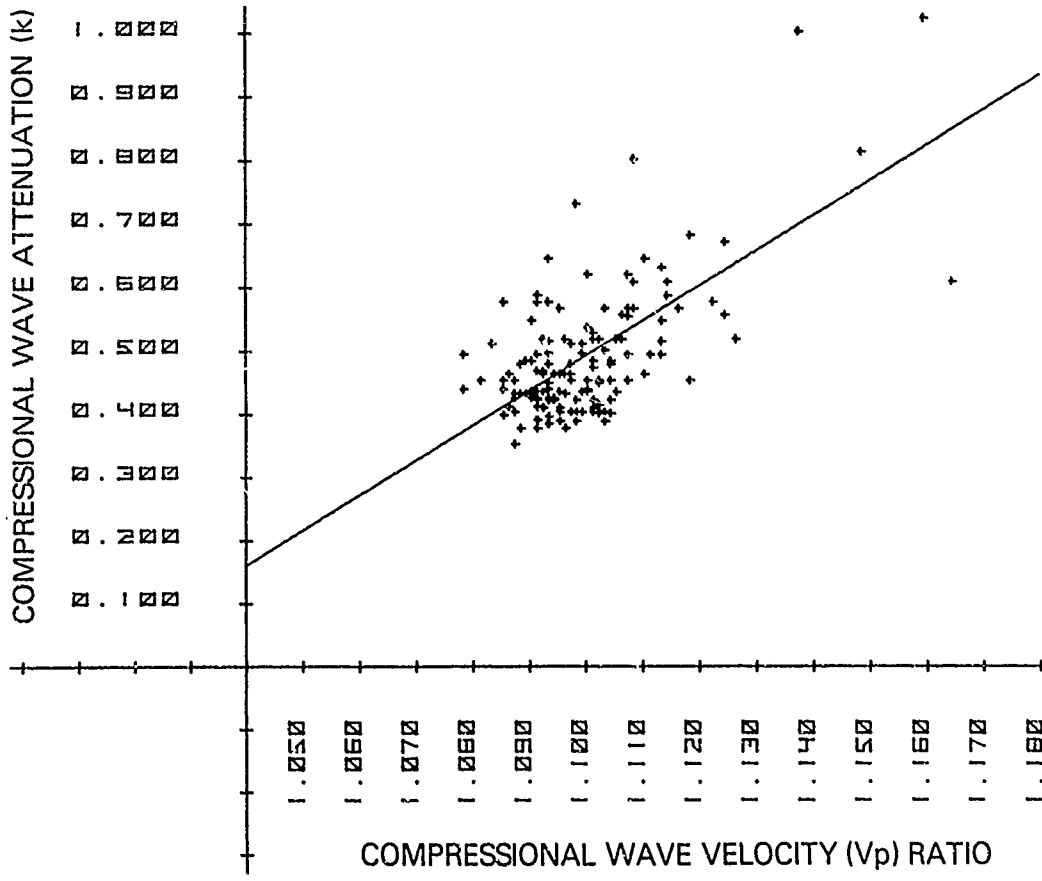
Figure 16A. Regression of sediment geoaoustic properties for fine sand sediments; attenuation with velocity ratio.
