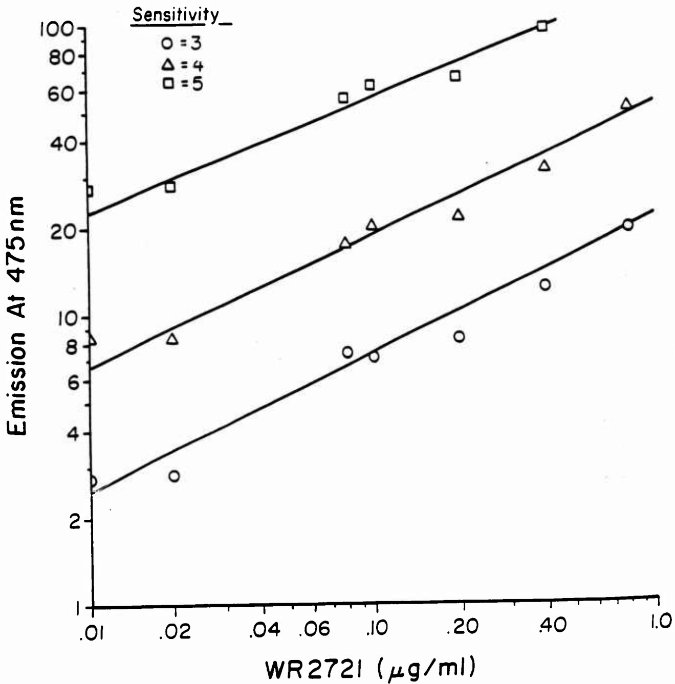
Figure 7a. Fluorescence emission of fluorecamine-WR 2721 derivative obtained at various spectrofluorometer sensitivity settings as function of WR 2721 concentration (0-01 - 1.0 micrograms/mL).
