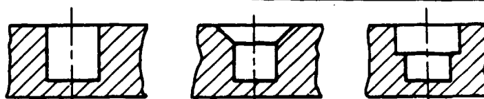
Blind Hole
