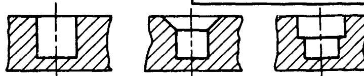
Blind Hole
