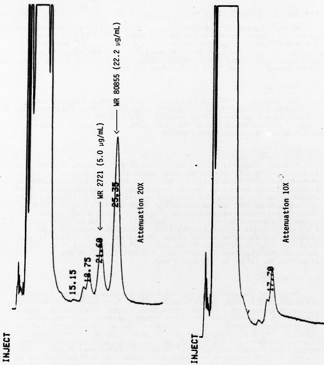
a) Beagle plasma spiked with WR 2721 and WR 80855.
